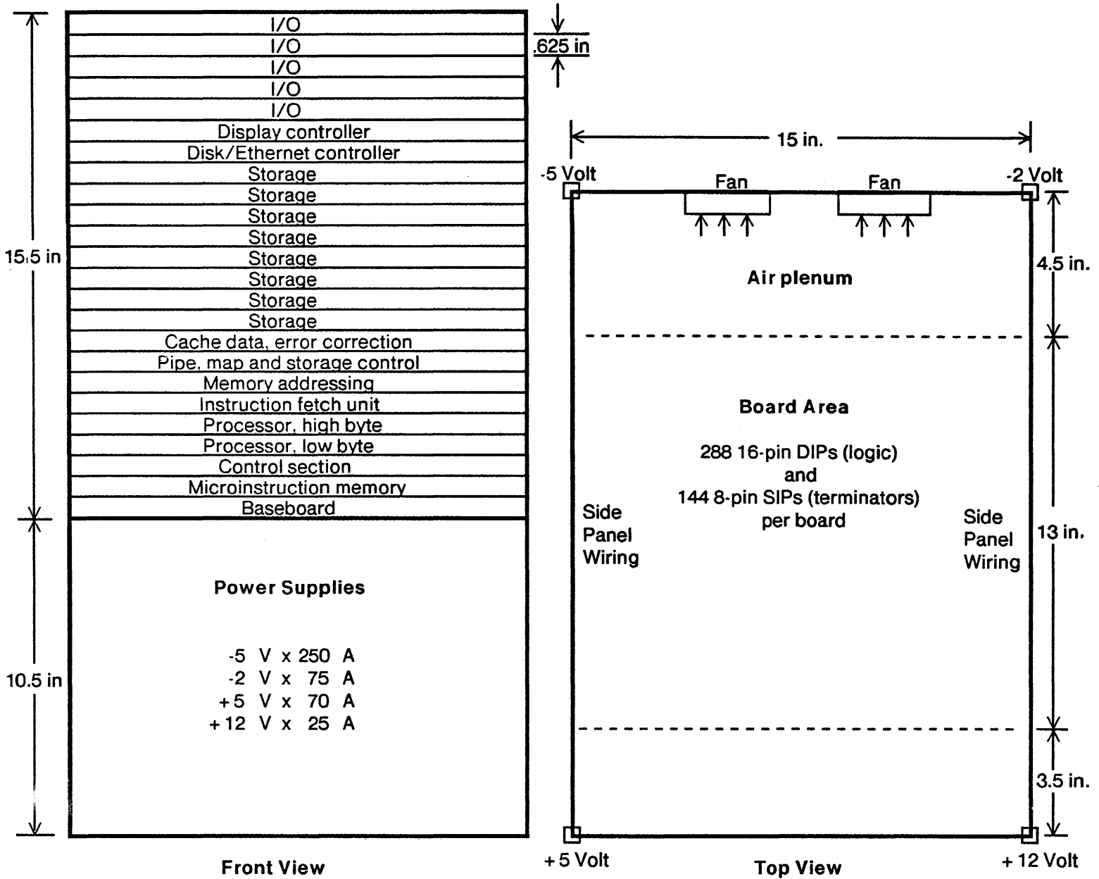
Figure 1a: Dorado chassis
