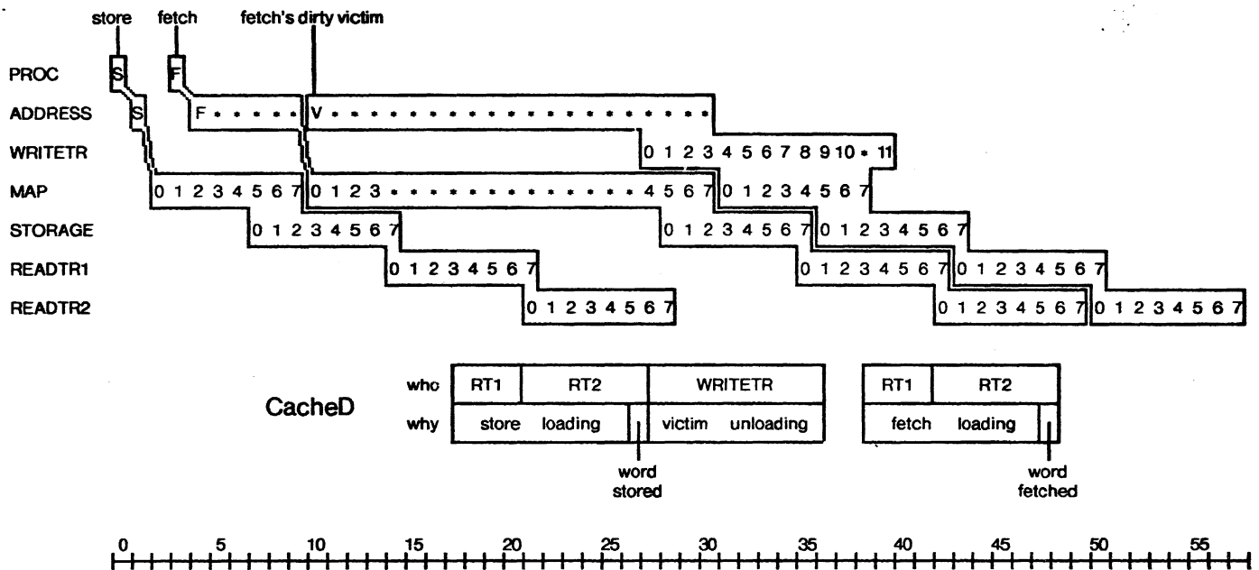
Figure 15: Cache load/unload conflict for CacheD
