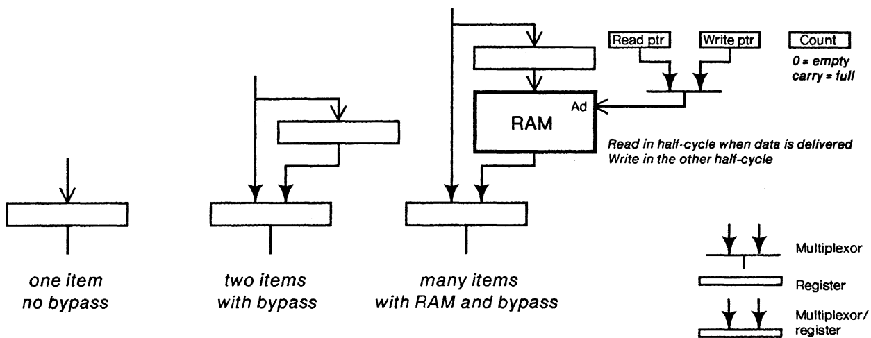
Figure 6: One, two and many item buffers with bypassing
