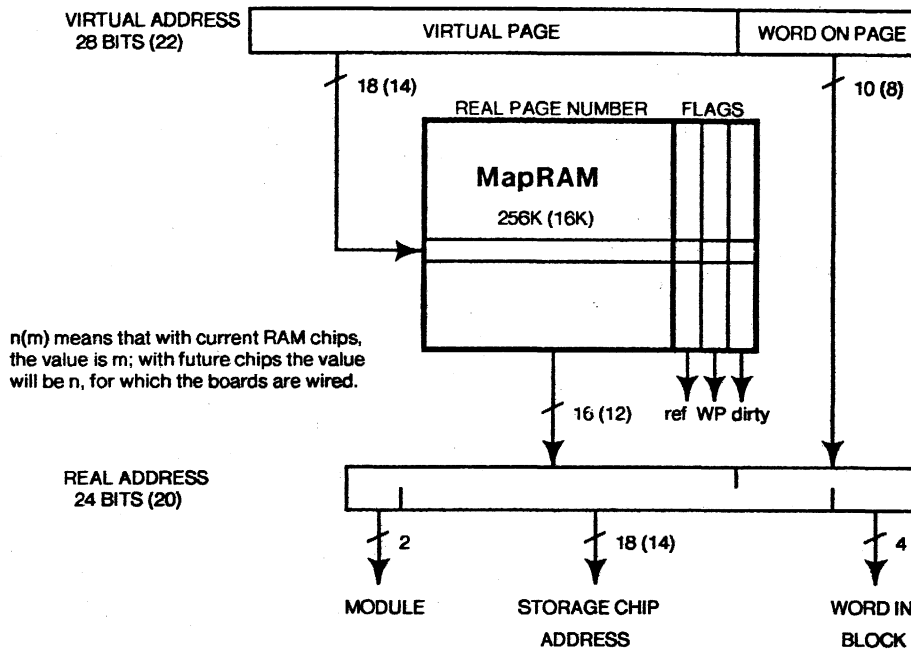
Figure 5: Virtual address to real address mapping.
