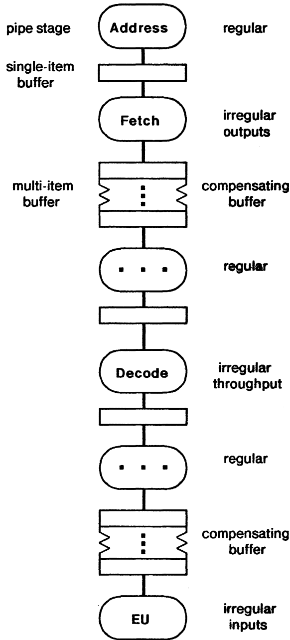
Figure 2: Sources of irregularity in an IFU pipeline
