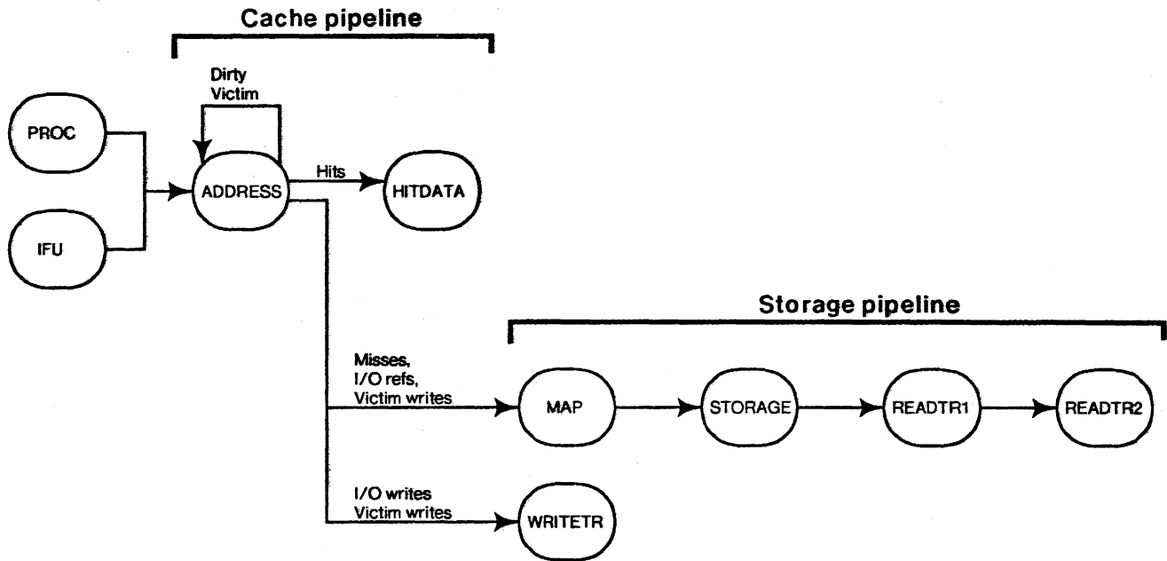
Figure 3: Cache and Storage Pipelines
