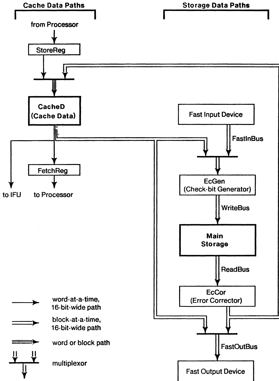
Figure 2: Data Paths
