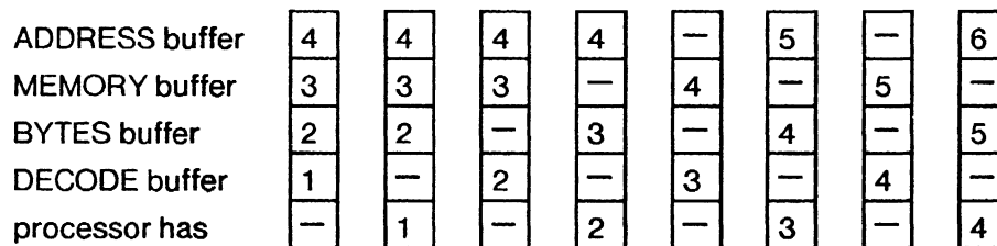
Figure 5a: Cogging with local control and one item buffering
