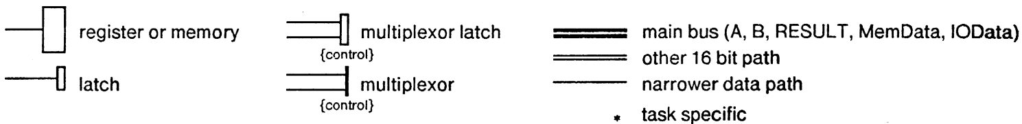
Figure 6: Data section
