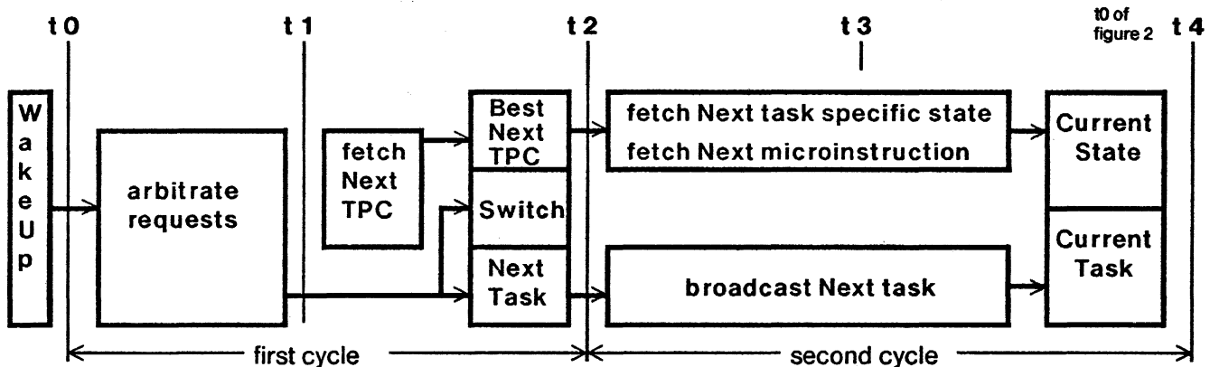
Figure 3: Task arbitration pipeline
