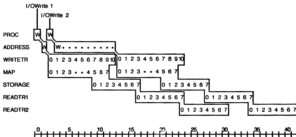
Figure 13: Two I/Owrites
