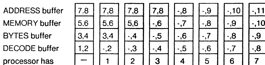
Figure 5b: Smooth operation with local control and two item buffering
