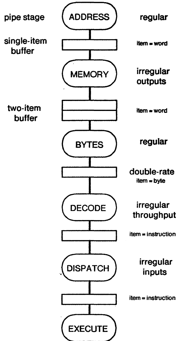
Figure 3: Pipeline stages in the Dorado IFU
