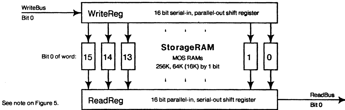
Figure 6: One bit-slice of StorageRAM and its data registers.
