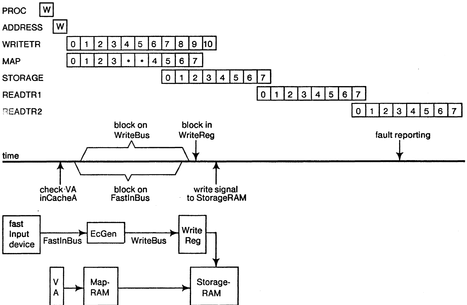
Figure 8: An I/OWrite reference
