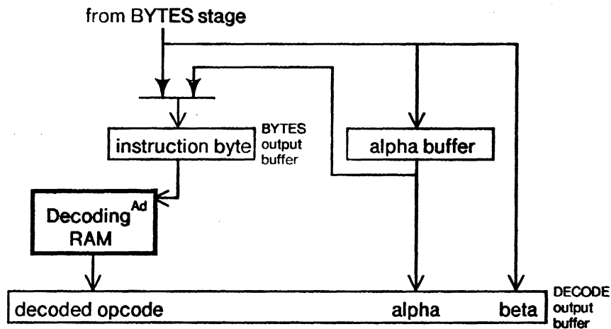
Figure 7c: Recycling implementation of DECODE
