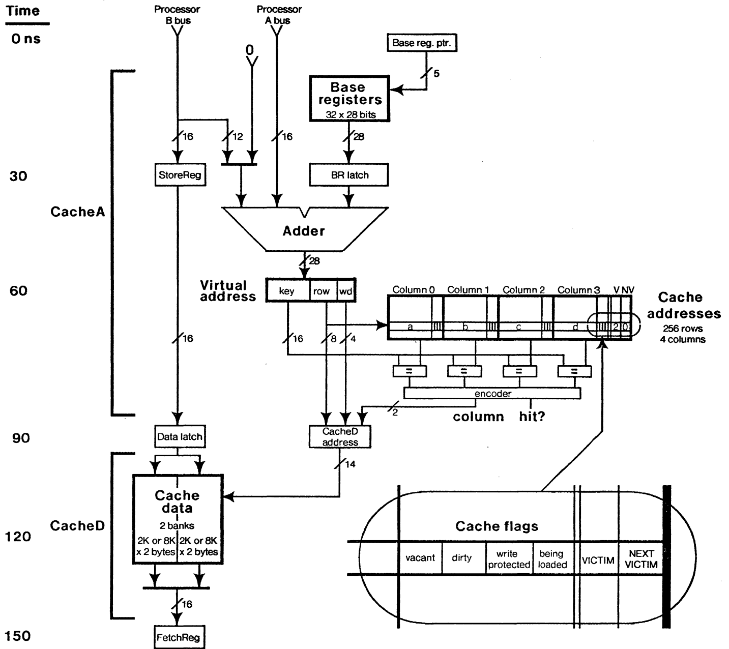
Figure 4: Data paths in the cache
