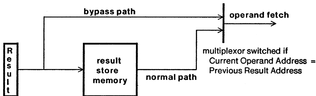
Figure 4: Bypassing example
