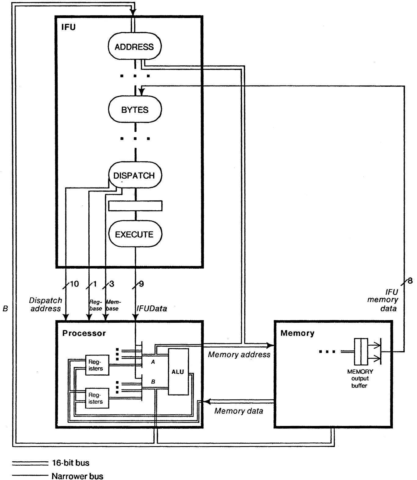
Figure 4: Buses between the IFU and the processor/memory
