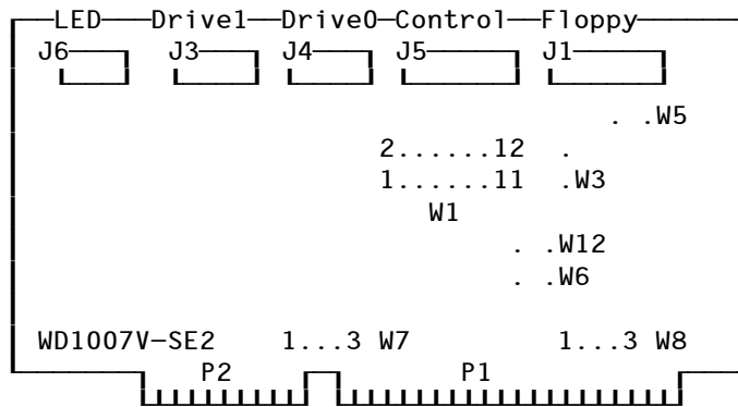
FIGURE 2-2. WD1007V-SE2
