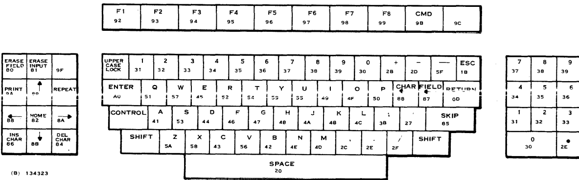
Figure 3-7. Keyboard Showing Uppercase Mode Character Positions and Hexadecimal Codes
