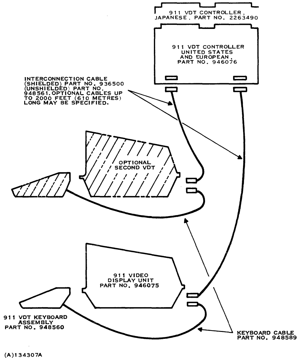
Figure 1-2. Model 911 VDT Standard Configuration
