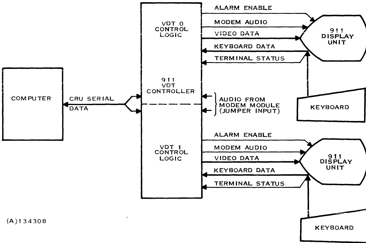
Figure 1-3. Major Terminal System Components
