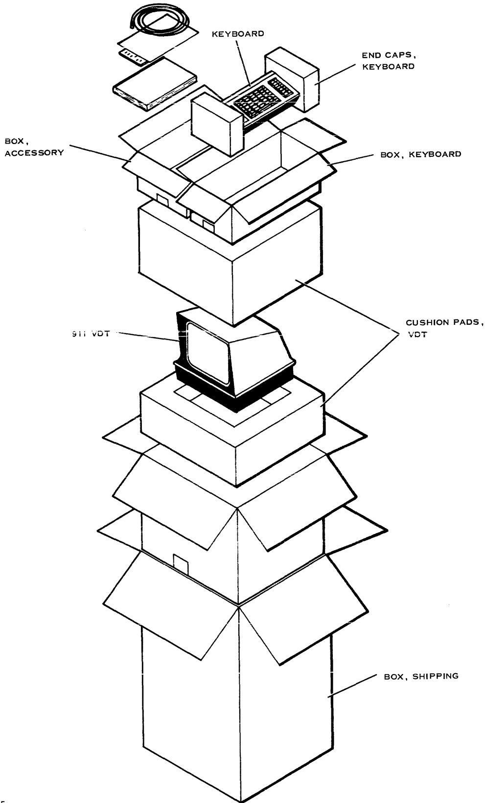
Figure 2-2. Model 911 Video Display and Keyboard Shipping Container
