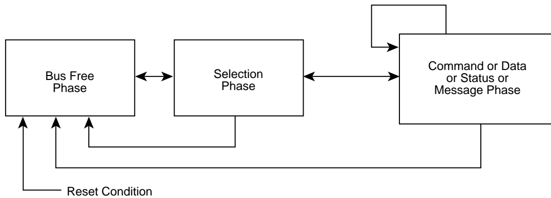
Figure 3.3-2. Phase sequences without arbitration
