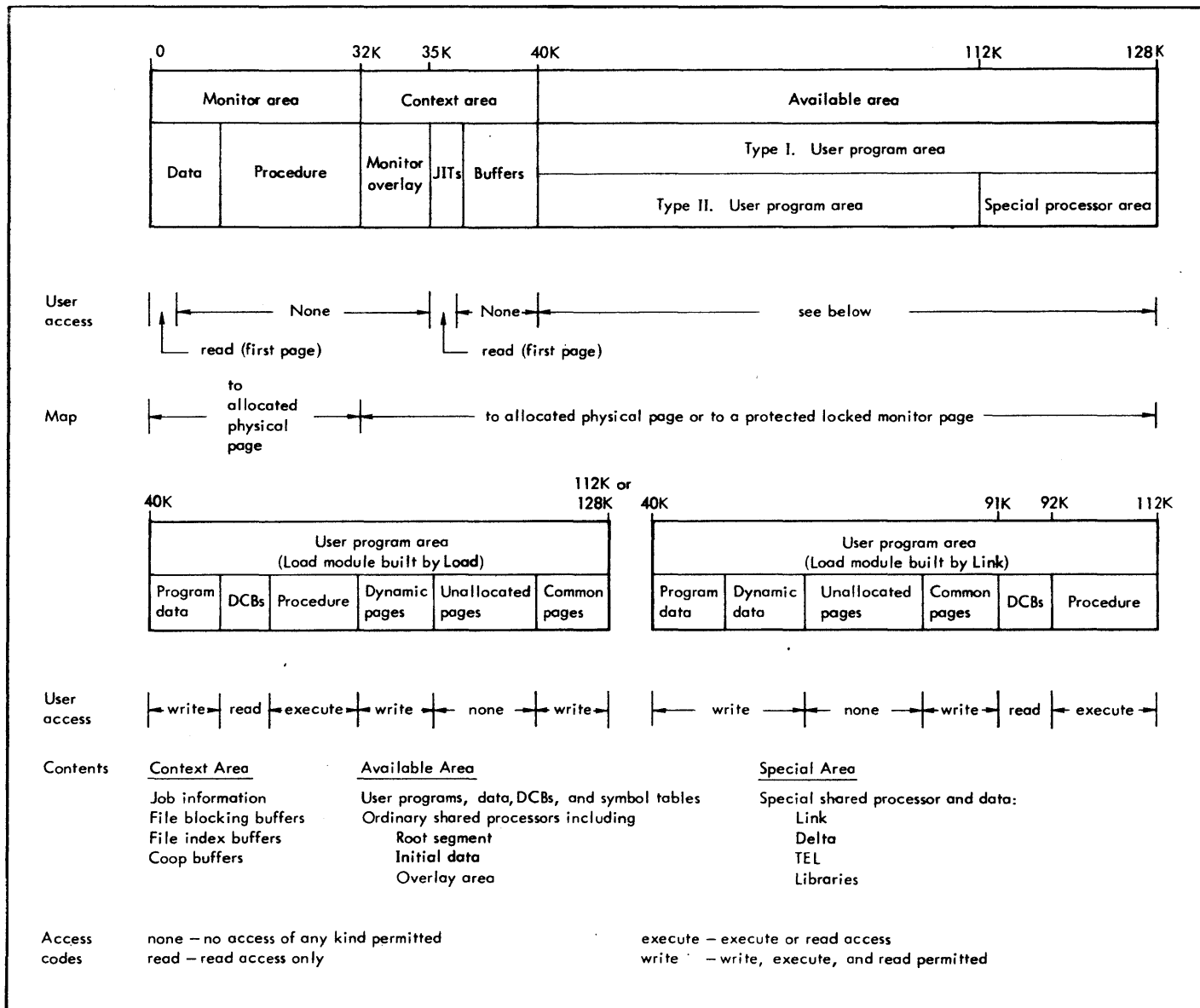
Figure 2. Typical User Program - Virtual Memory Layout (not to scale)
