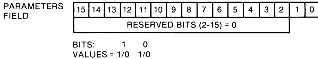
Figure 4-9. Parameters Field in TPAB
