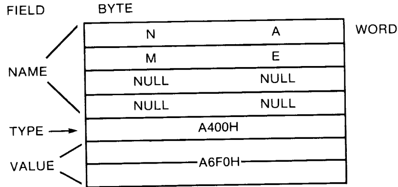
Figure 3-3. Entry in Symbol Table
