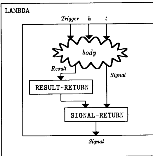
Figure 4.6: Dataflow graph for procedure cons.
