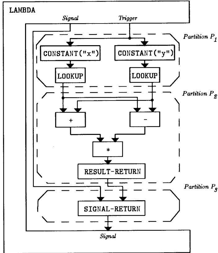
Figure 4.20: Partitioning of graph for (lambda () (* (+ x y) (- x y))).
