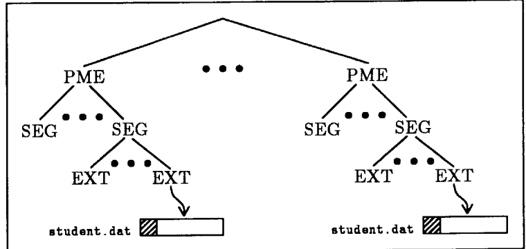
Figure 5.6: Allocation of initial physical extents in student files.
