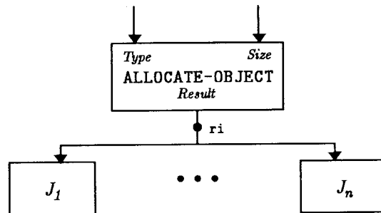
Figure 4.23: Reuse of result value in slot r_i .
