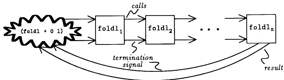
Figure 4.15: Modified unfolding of computation for (\text{foldl} + 0 1) .
