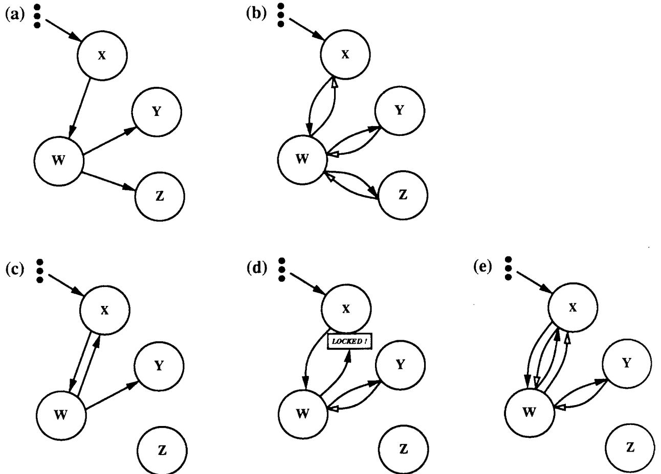
Figure 1: Graph fragments and calling patterns in the abstract query example. In the calling pattern diagrams, call and reply messages are represented by solid and hollow arrowheads respectively. (a) A non-recursive graph fragment. (b) Call pattern in the non-recursive graph fragment. X calls W , which concurrently calls Y and Z . (c) A recursive graph fragment. (d) Call pattern in the recursive graph fragment. X calls W , which concurrently calls X and Y , resulting in deadlock. (e) A deadlock-free call chain, which uses the solution techniques presented in the paper.
