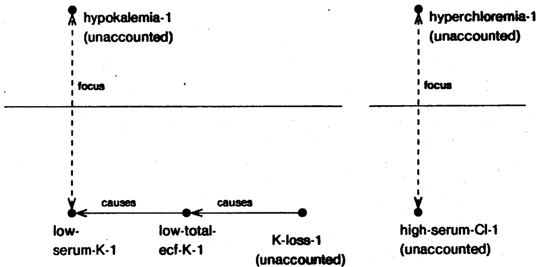
Fig. 22. Causal aggregation: fully unaccounted node
