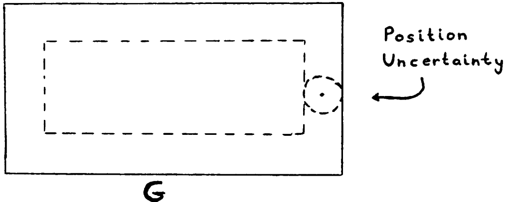
Figure 3.29. All points inside the dashed region are recognizable in the goal. The dashed region is so chosen that the possible sensor interpretations of all points lie within the larger goal region.
