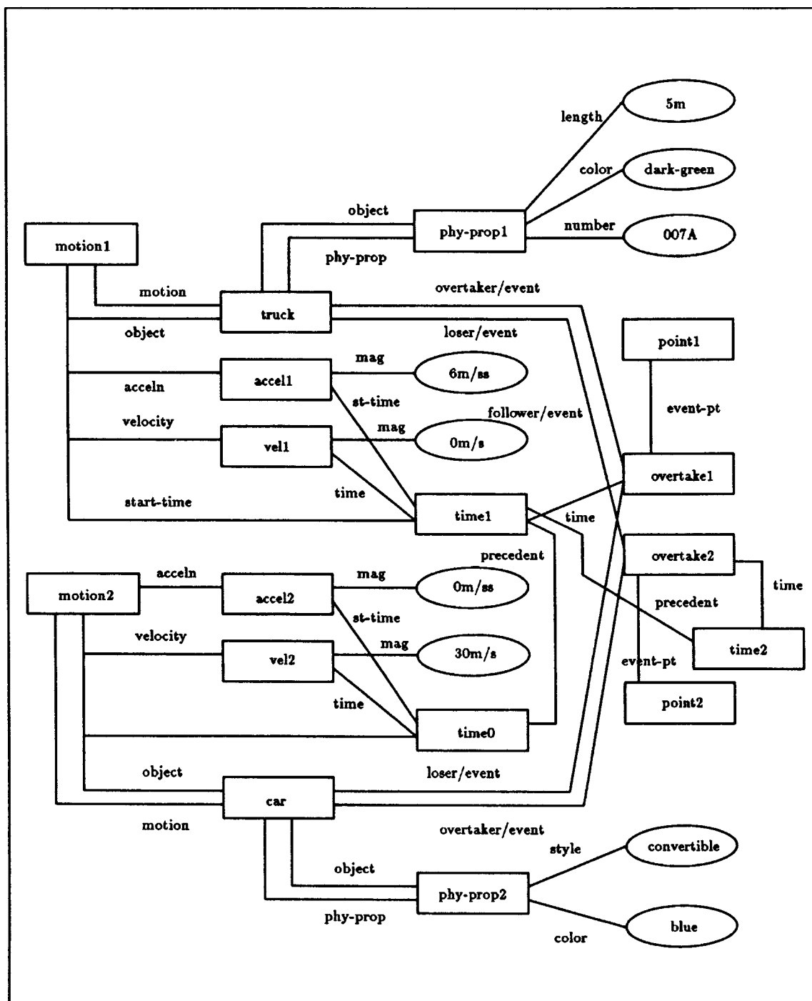
Figure 1.1: A Semantic Net Representation of the OVERTAKE Problem
