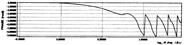
Figure 10-7: Time-varying frequency responses at (a) \theta = 0.0 \text{ rad} (target 1), (b) \theta = 0.5 \text{ rad} (on the extension movement), and (c) \theta = 1.0 \text{ rad} (target 2). The natural frequencies, given by the point at which phase angle crosses -90 degrees, are respectively (a) 1.77 Hz, (b) 0.63 Hz, and (c) 2.51 Hz. Data are for subject S2 moving at the 750 ms rate in the vertical plane.
