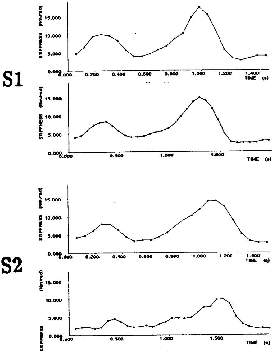
Figure 10-15: Same as Figure 10-11, except that the movement occurred in the vertical plane.
