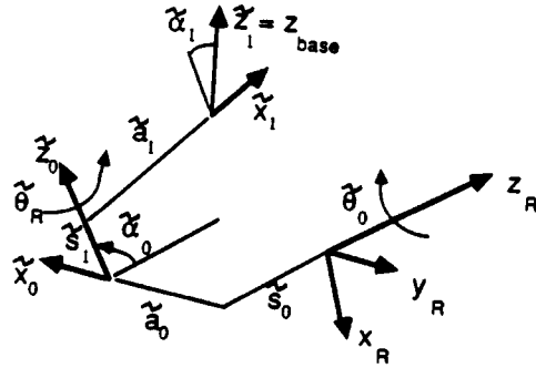
Figure 5-2: The right camera axes to base D-H transformations. The first transformation locates the line of action of the right camera rotation. The second transformation locates the base coordinate z-axis, which is also the left camera axis of rotation.
