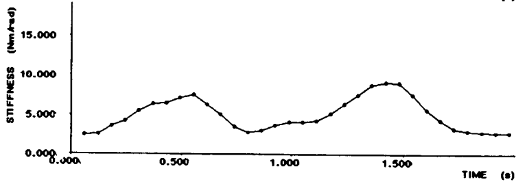
Figure 10-11: Stiffness profiles for two speed conditions for subjects S1 and S2 moving in the horizontal plane.
