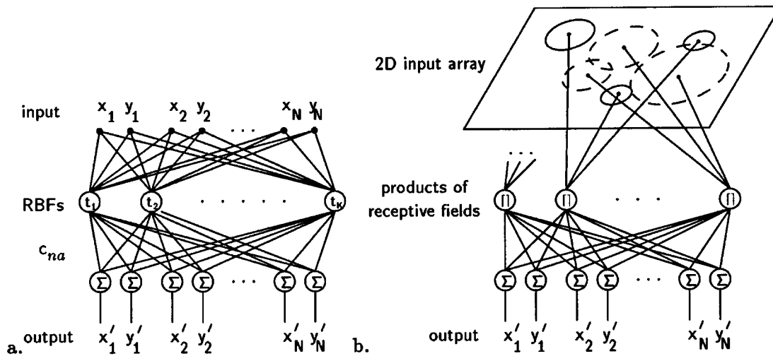
Figure 2: (a) A network representation of approximation by Generalized Radial Basis Functions. (b) shows an equivalent interpretation of (a) for the case of Gaussian radial basis functions. The solid circles in the image plane represent the 2D Gaussians associated with the first radial basis function, which corresponds to the first view of the object. The dotted circles represent the 2D receptive fields that synthesize the Gaussian radial function associated with another view.
