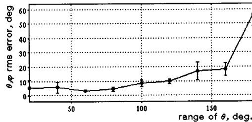
Figure 11: Errors in the viewpoint coordinates \theta, \phi recovered by the module vs. the range of the viewpoint coordinates ( M = K = 40, \sigma = 30 ).
