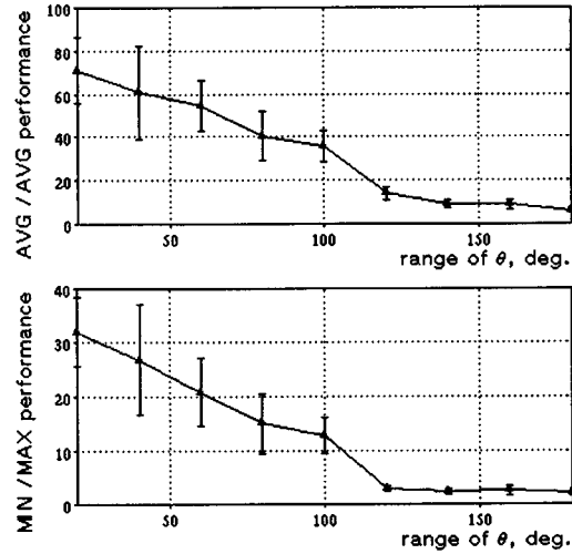
Figure 10: AVG/AVG and MIN/MAX performance vs. the range of the viewpoint coordinates \theta, \phi (the objects are a cube and an octahedron, M = K = 40 \sigma = 30.0 , and the error bars are standard deviations over 10 sets of random training and testing views). Here and in the next figure, \phi_{max} = 2\theta_{max} , so that \theta_{max} = 180^\circ corresponds to the full viewing sphere.
