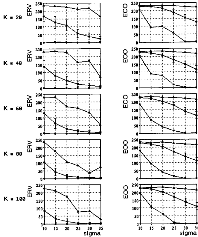
Figure 6: Error (distance between actual and ideal output) vs. the size \sigma of the basis functions, for modules with different number of centers K (the number of training views M is equal here to K ). Data are shown for two input sets: random views of the trained object (ERV, left column) and views of other nine objects (EOO, right column). Three measures of the error, MIN (lower curves), AVG (middle curves) and MAX (upper curves) are shown separately. Bars indicate standard deviation, computed over ten different training objects.
