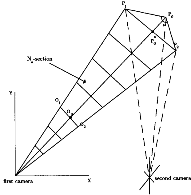
Figure 14: The N_o -section of a plane containing P_1 , P_0 , P_2 and the first camera.
