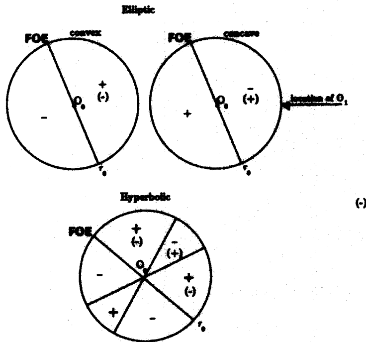
Figure 7: The sign of \Upsilon(\tau) depends on the relative position of O_1 with respect to O_0 and the FOE. In the figure, the circle represents possible locations of O_1 , the +/- inside indicates the sign of \Upsilon(\tau) whereas the sign of the normal curvature is given in parentheses. Above is the elliptic case, below is the hyperbolic case.
