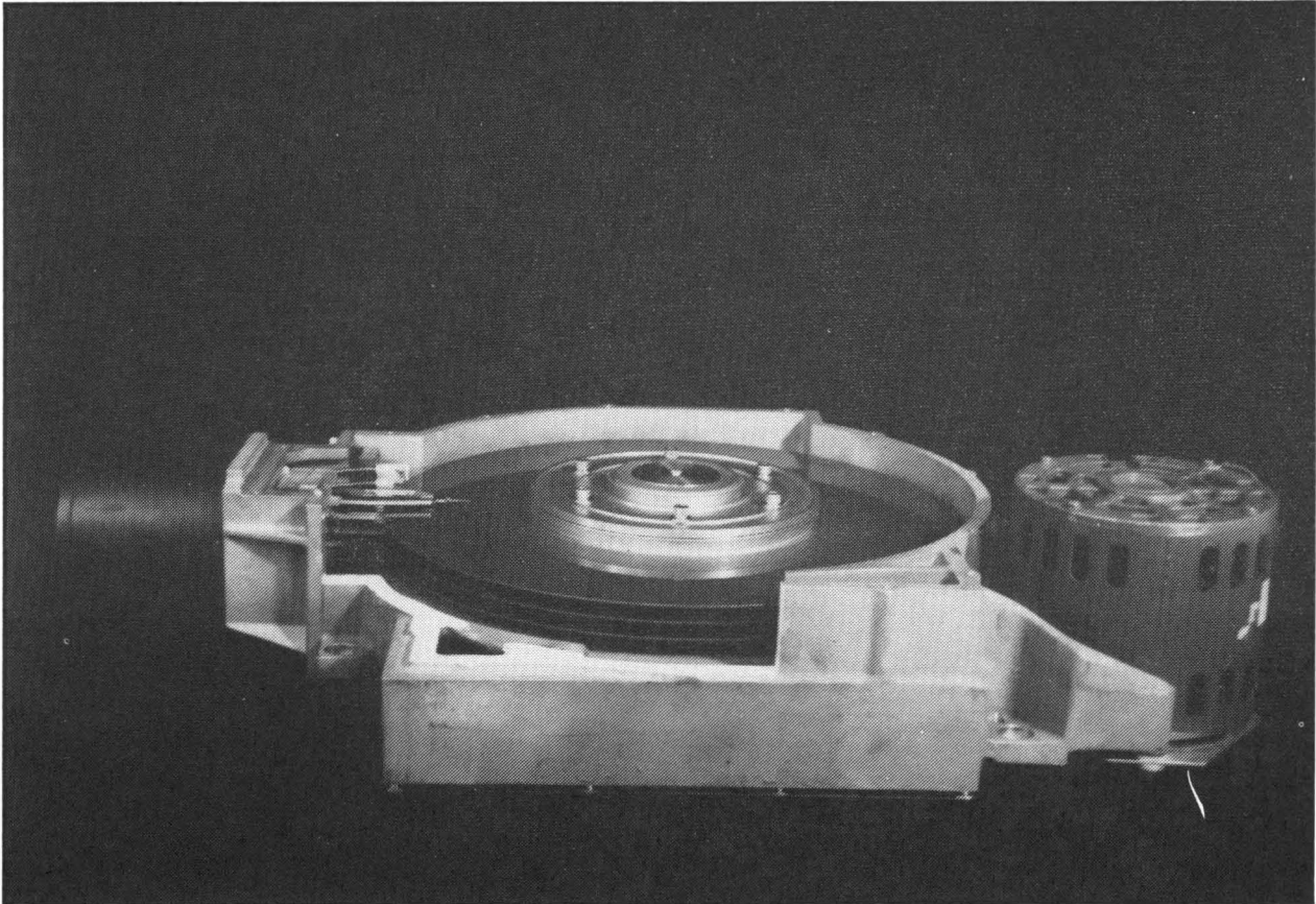
Figure 1. Reflex I Sealed Module (Cutaway View)
