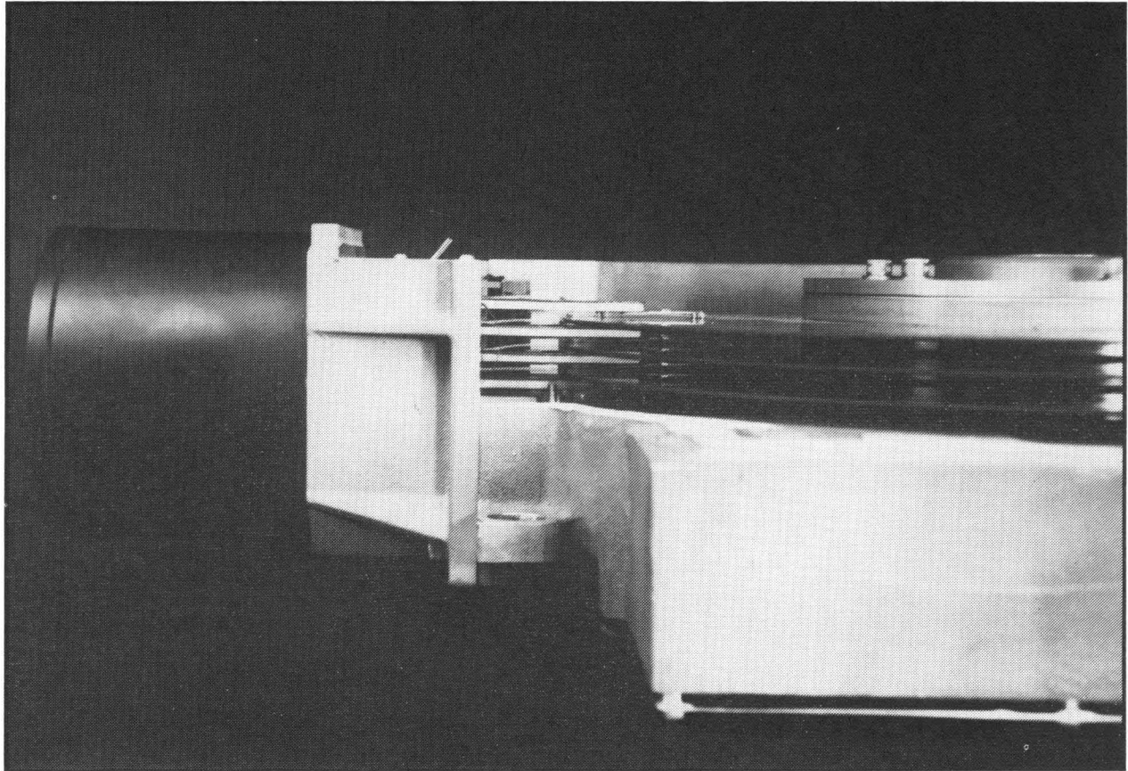
Figure 2. Reflex I Heads and Platters
