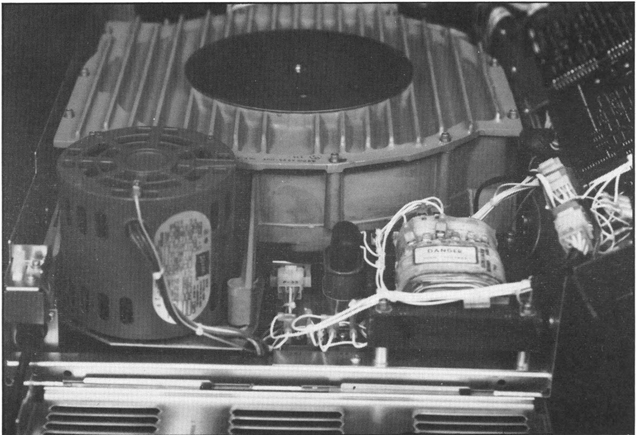
Figure 33. Transformer Assembly Removal.
