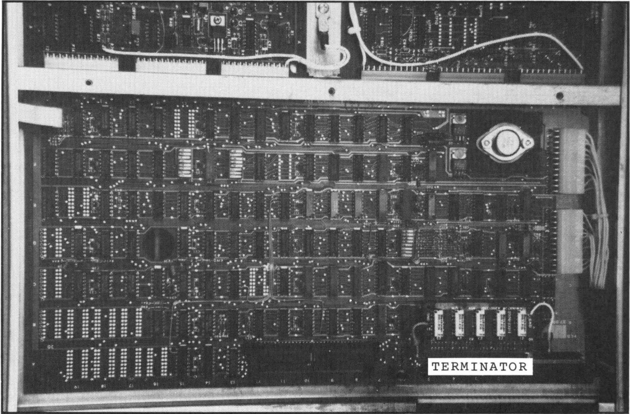
Figure 10. Logic Interface PCB
