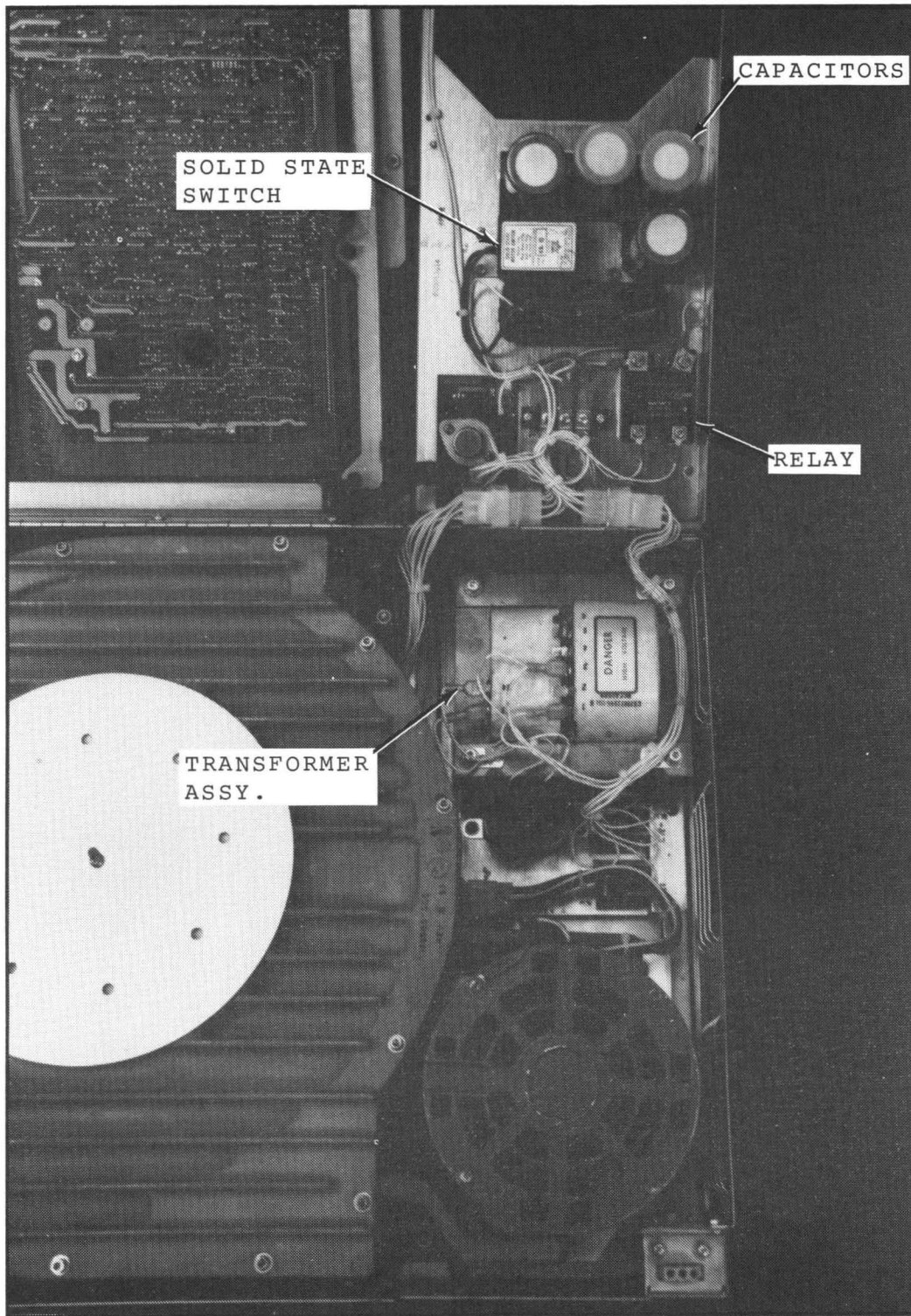
Figure 9. Power Components
