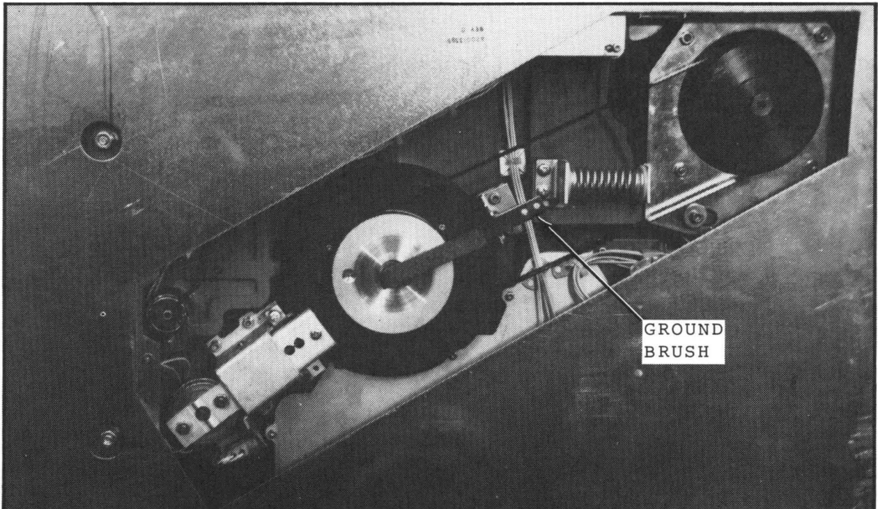
Figure 21. Ground Brush Assembly
