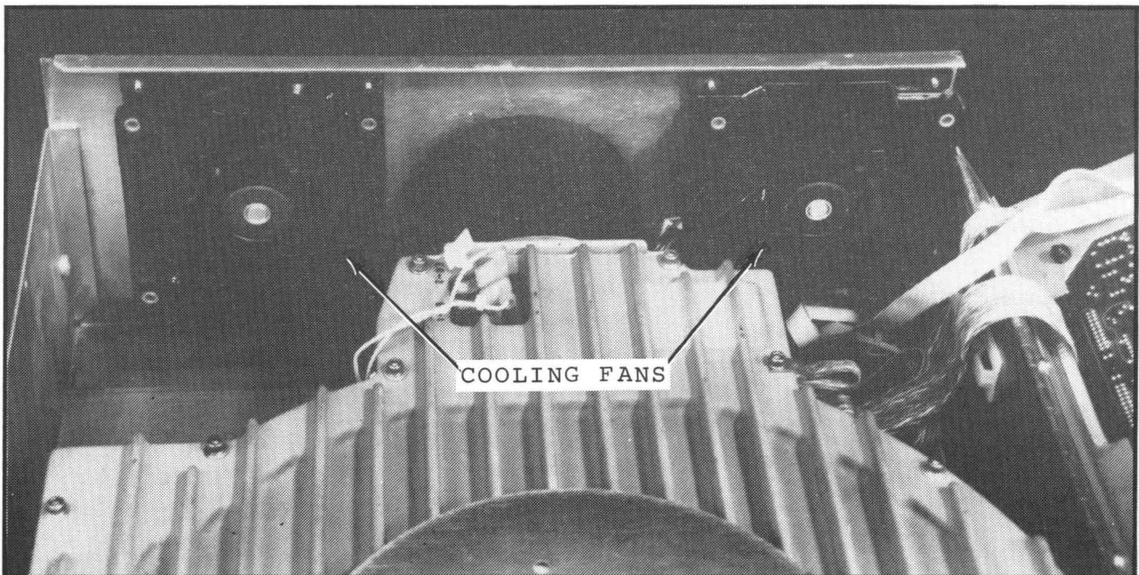
Figure 8. Cooling Fan Location 16
