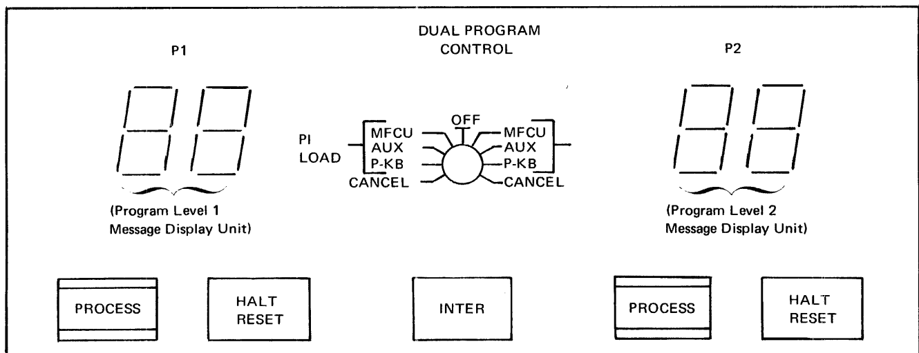
Figure 3-4. Dual Programming Control Panel
