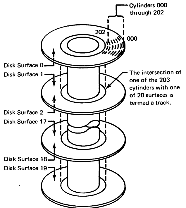
Figure 6-16. Cylinder Concept
