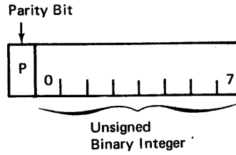
Figure 1-5. Binary Format
