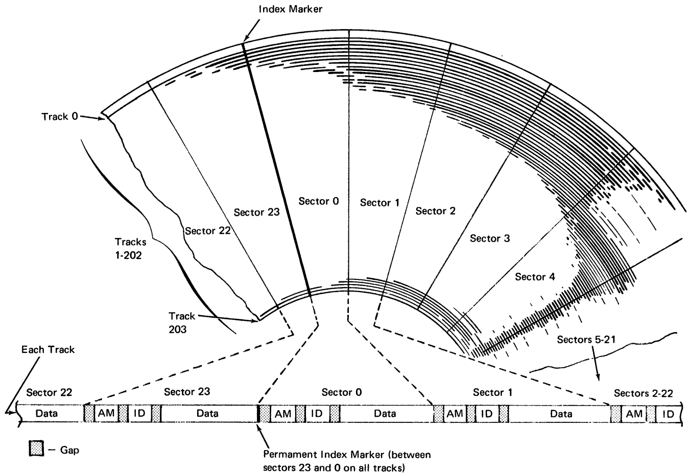
Figure 6-4. Sector Layout
