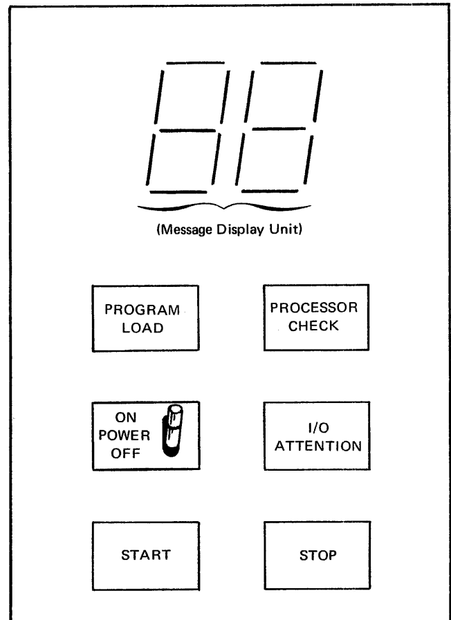
Figure 3-3. System Controls
