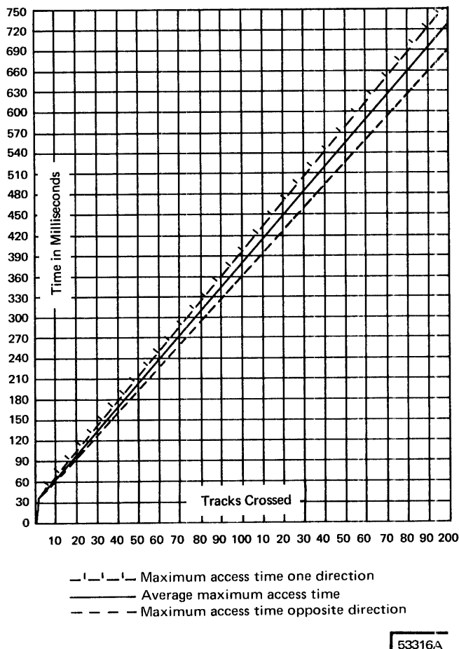
Figure 6-5. Access Timing (Models 1, 2, and 3)
