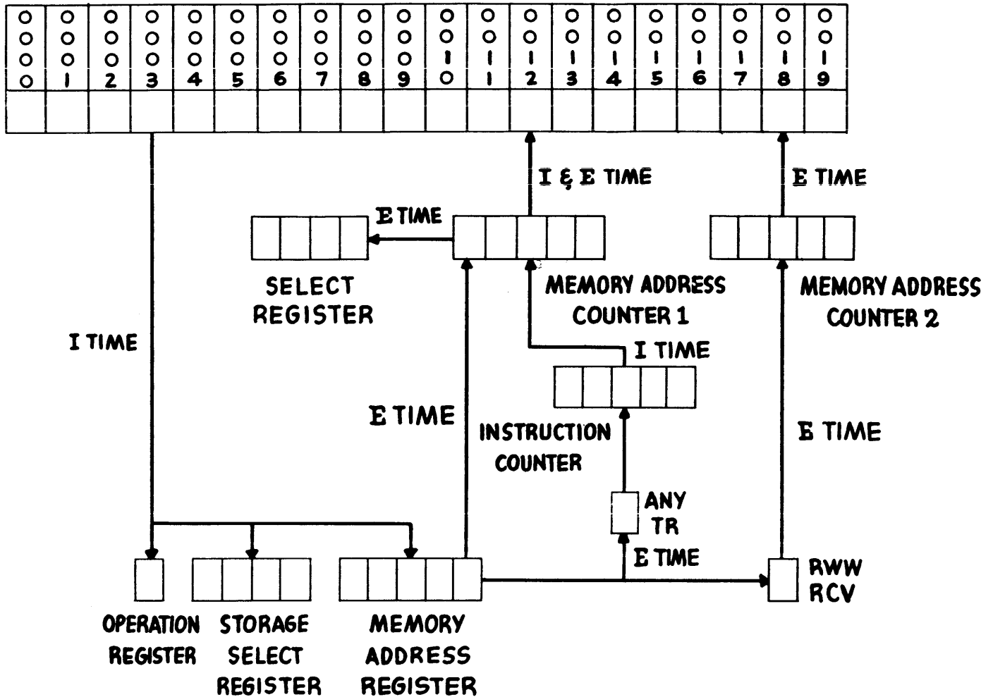
SCHEMATIC REPRESENTATION OF RELATIONSHIP BETWEEN. MEMORY ADDRESS REGISTER OPERATION REGISTER INSTRUCTION COUNTER MEMORY ADDRESS COUNTER 1 MEMORY ADDRESS COUNTER 2 SELECT REGISTER STORAGE SELECT REGISTER
