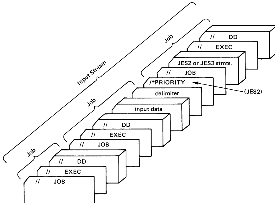
Figure 7. Job Boundaries in the Input Stream
