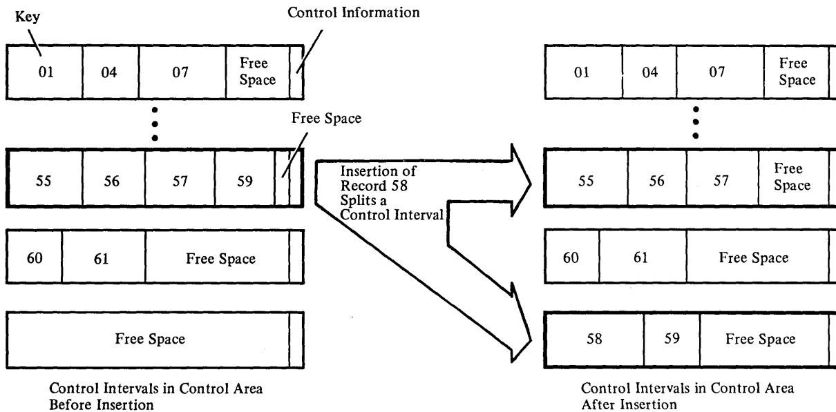
Figure 6. Control-Interval Split
