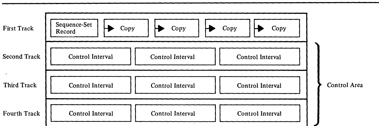
Figure 10. Index-Record Replication
