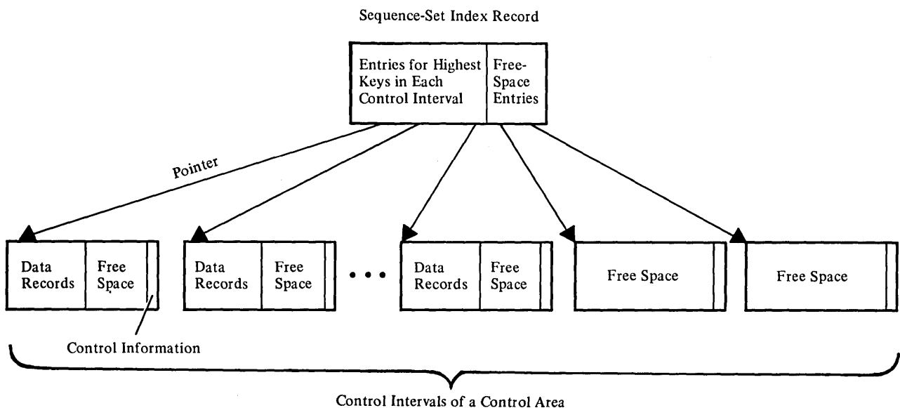
Figure 5. Free-Space Distribution
