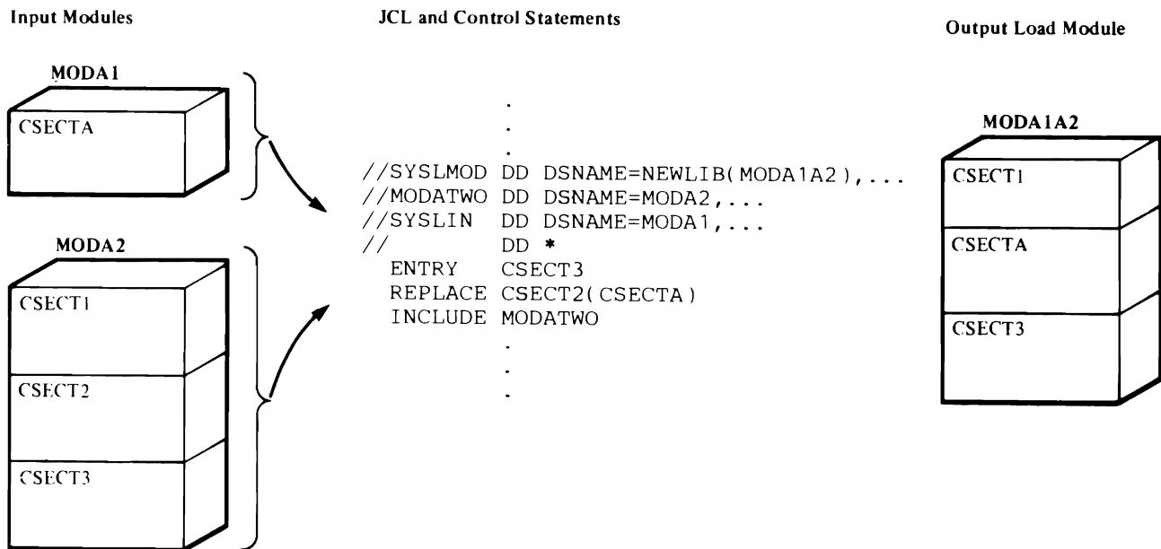
Figure 16. Editing a Module
