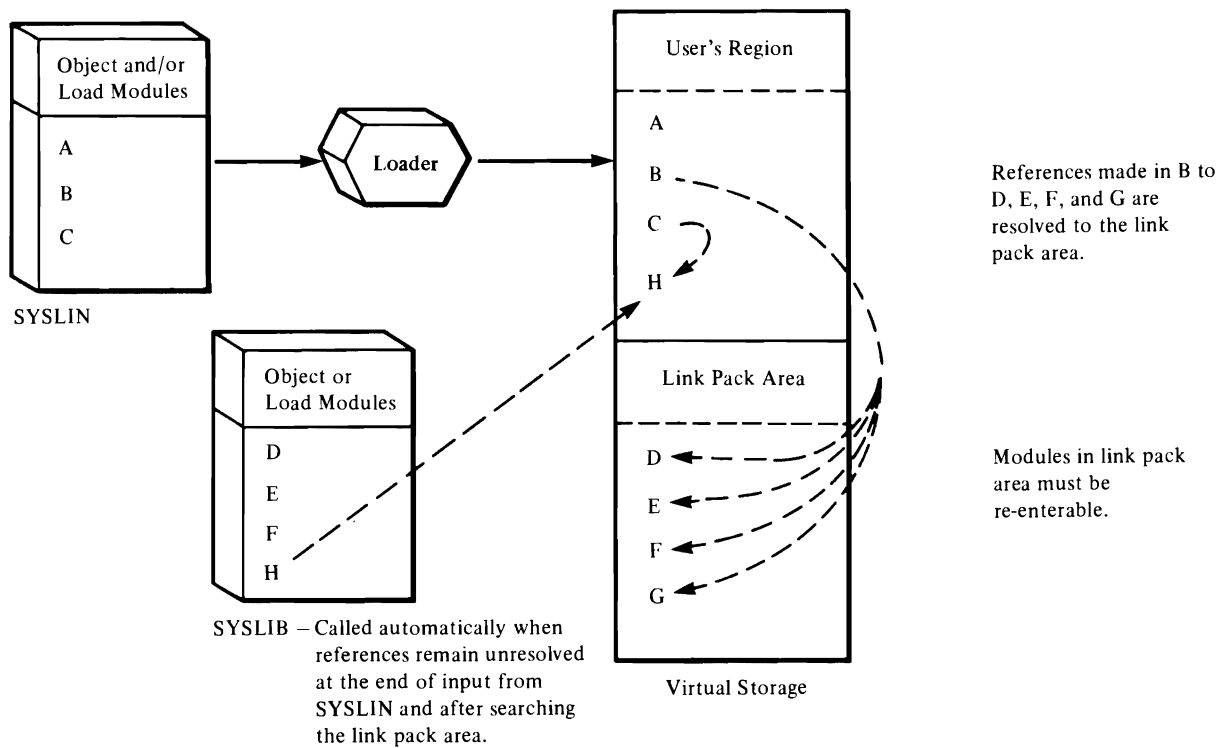
Figure 65. Loader Processing—Link Pack Area and SYSLIB Resolution
