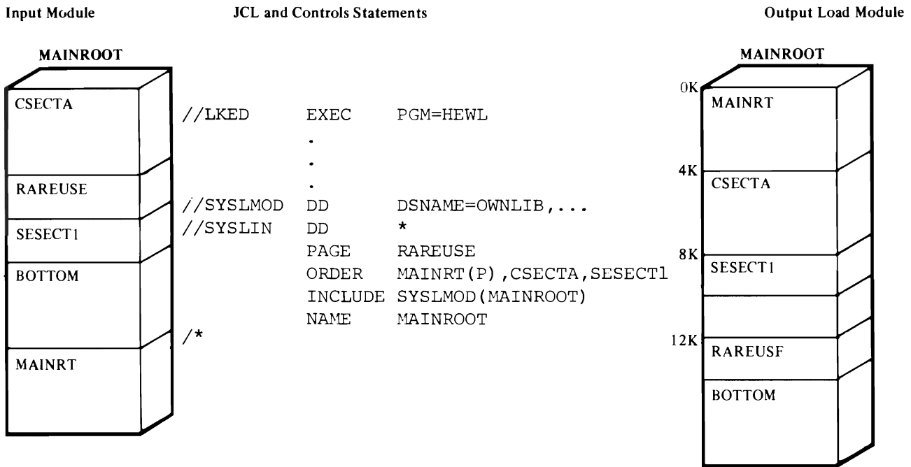
Figure 22. Aligning Control Sections on Page Boundaries
