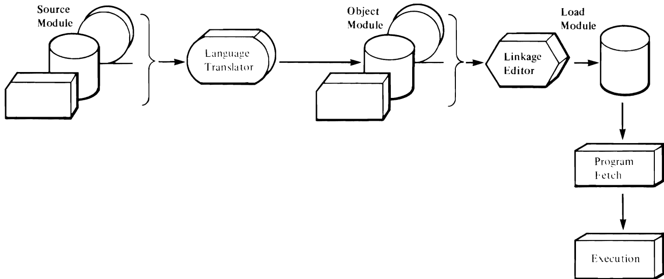
Figure 2. Preparing a Source Module for Execution, and Executing the Load Module
