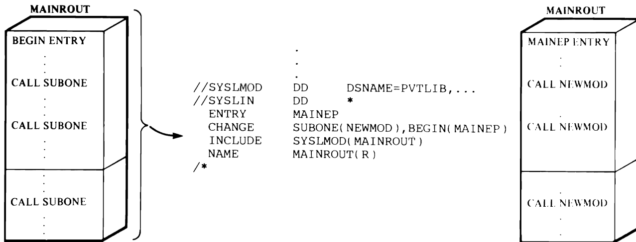
Figure 17. Changing an External Reference and an Entry Point
