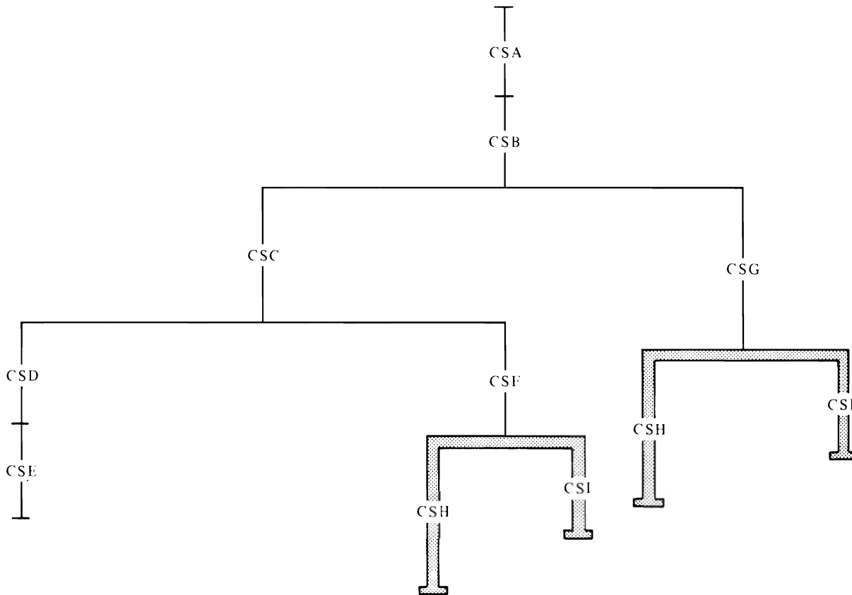
Figure 30. Control Sections Used by Several Paths
