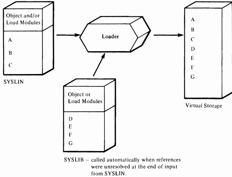
Figure 64. Loader Processing—SYSLIB Resolution
