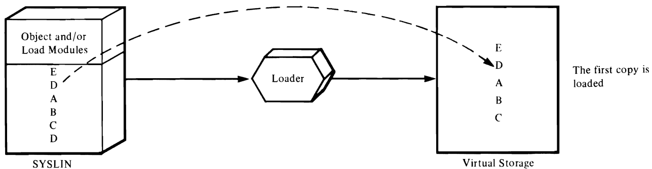
Figure 66. Loader Processing—Automatic Editing
