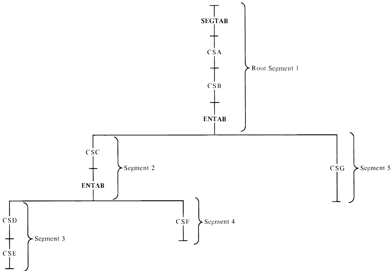
Figure 29. Location of Segment and Entry Tables in an Overlay Module
