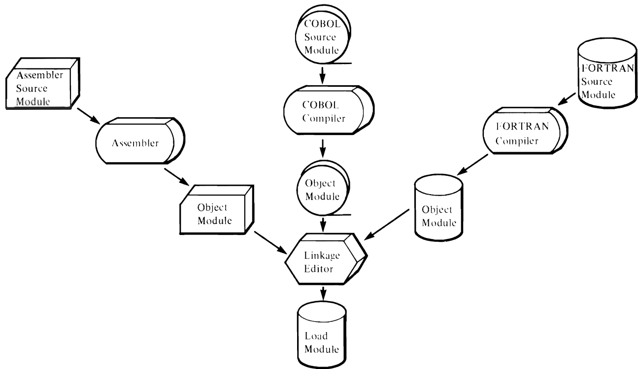
Figure 7. Linkage Editor Processing—Module Linkage
