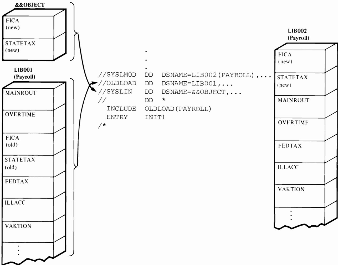
Figure 18. Automatic Replacement of Control Sections
