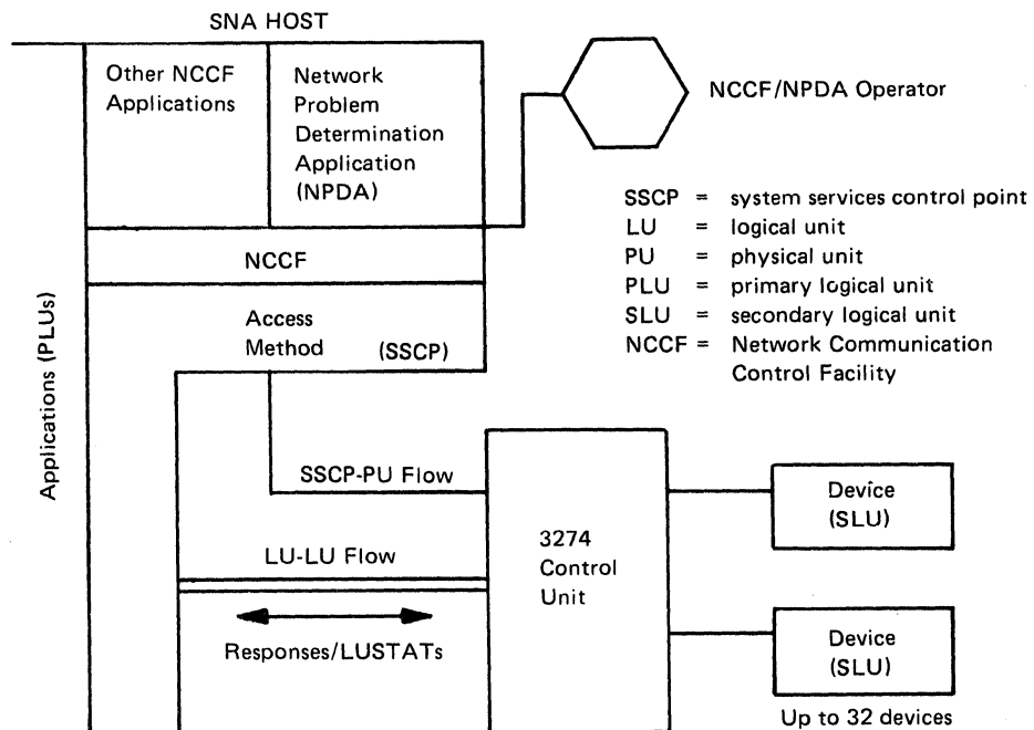
Figure 8-6. SNA Host Connection
