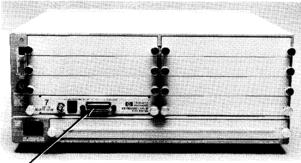
Internal HP-IB
