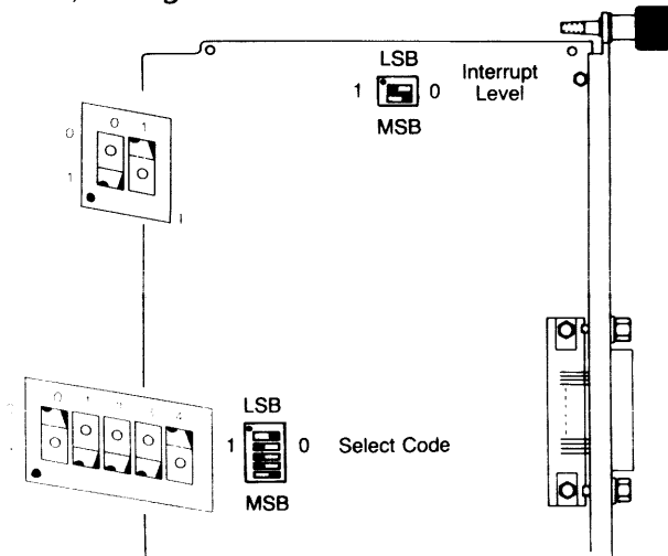
Configuring the HP 98625A High-speed Disc Interface for HP-UX
