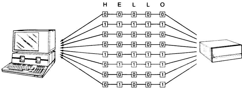
Parallel Transmission
