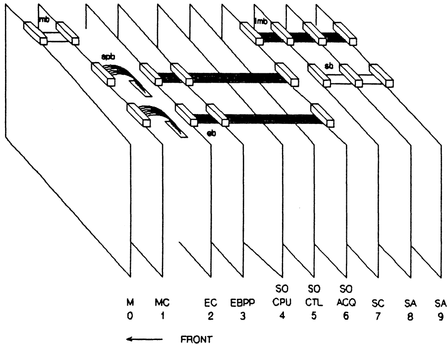
HP 64340A WITH EBPP / SPLIT BUS EMULATION
