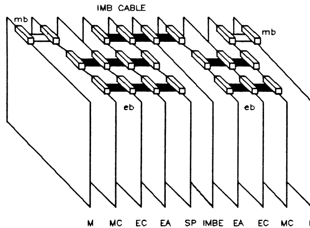
EXAMPLE OF AN IN-STATION CONFIGURATION
