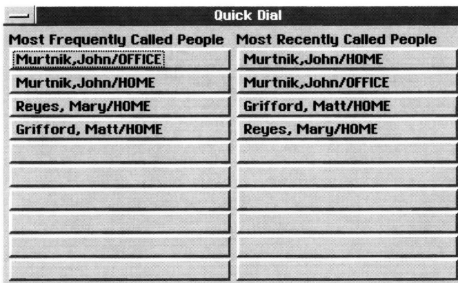
The Quick Dial window. The column of buttons on the left shows the numbers you dial most often, while the column on the right shows the last ten numbers you've dialed.
