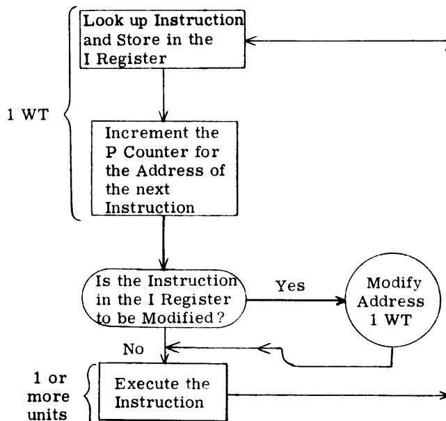
Figure 19. GE-225 Instruction-Execution Cycle
