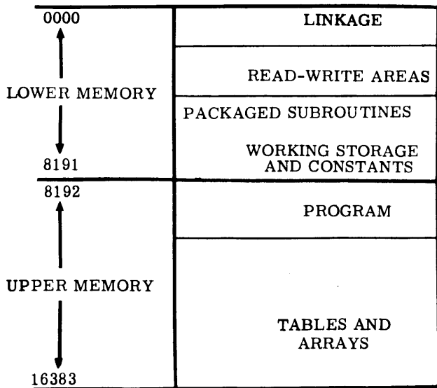
Figure 25. 16k Memory Layout
