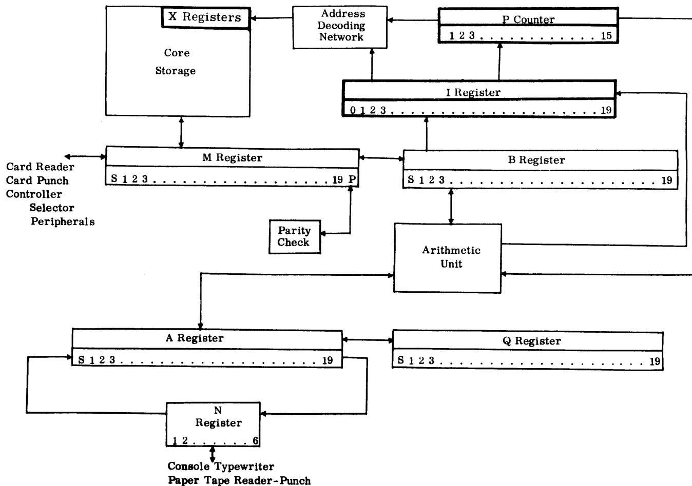
Figure 17. GE-225 Control Registers
