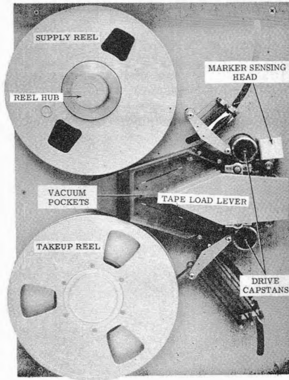
Figure 3. Tape Handler Mechanism
