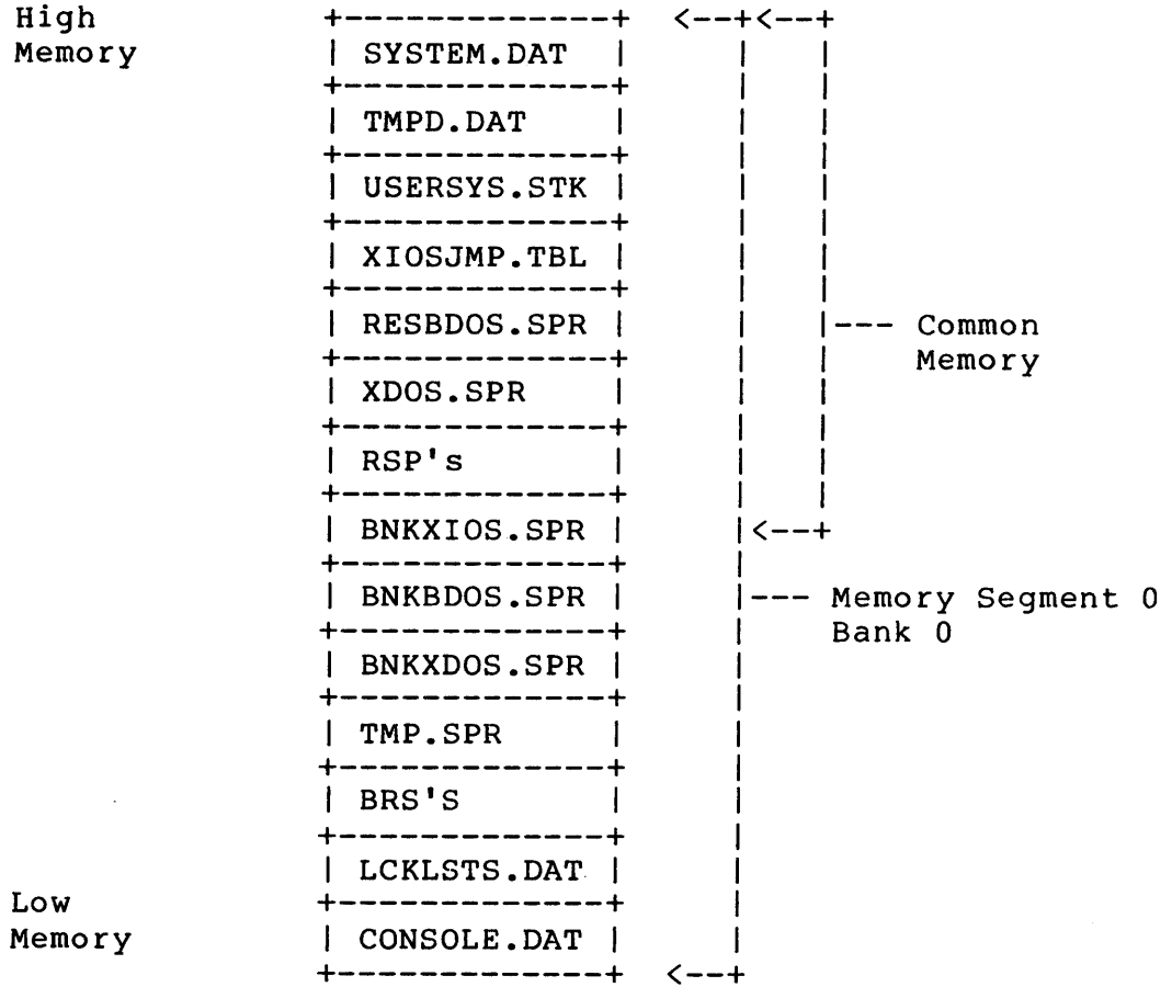
Figure 1-2. MP/M II Memory Structure
