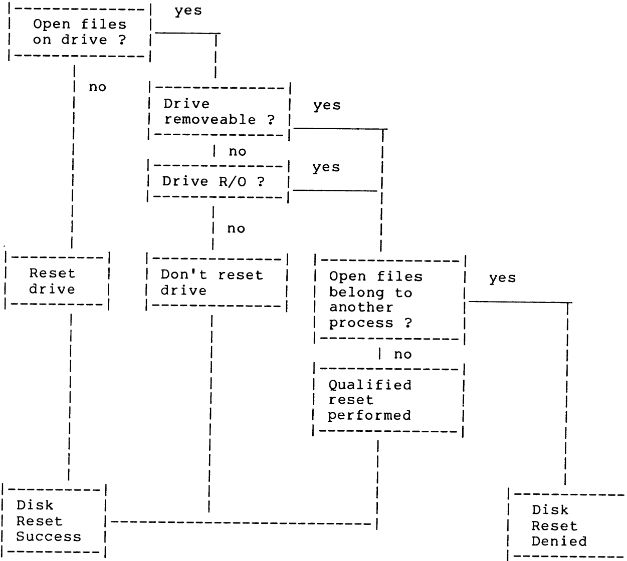
Figure 2-1. Disk System Reset
