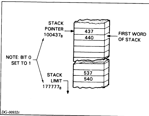
Figure 2.10 Unprotected stack area
