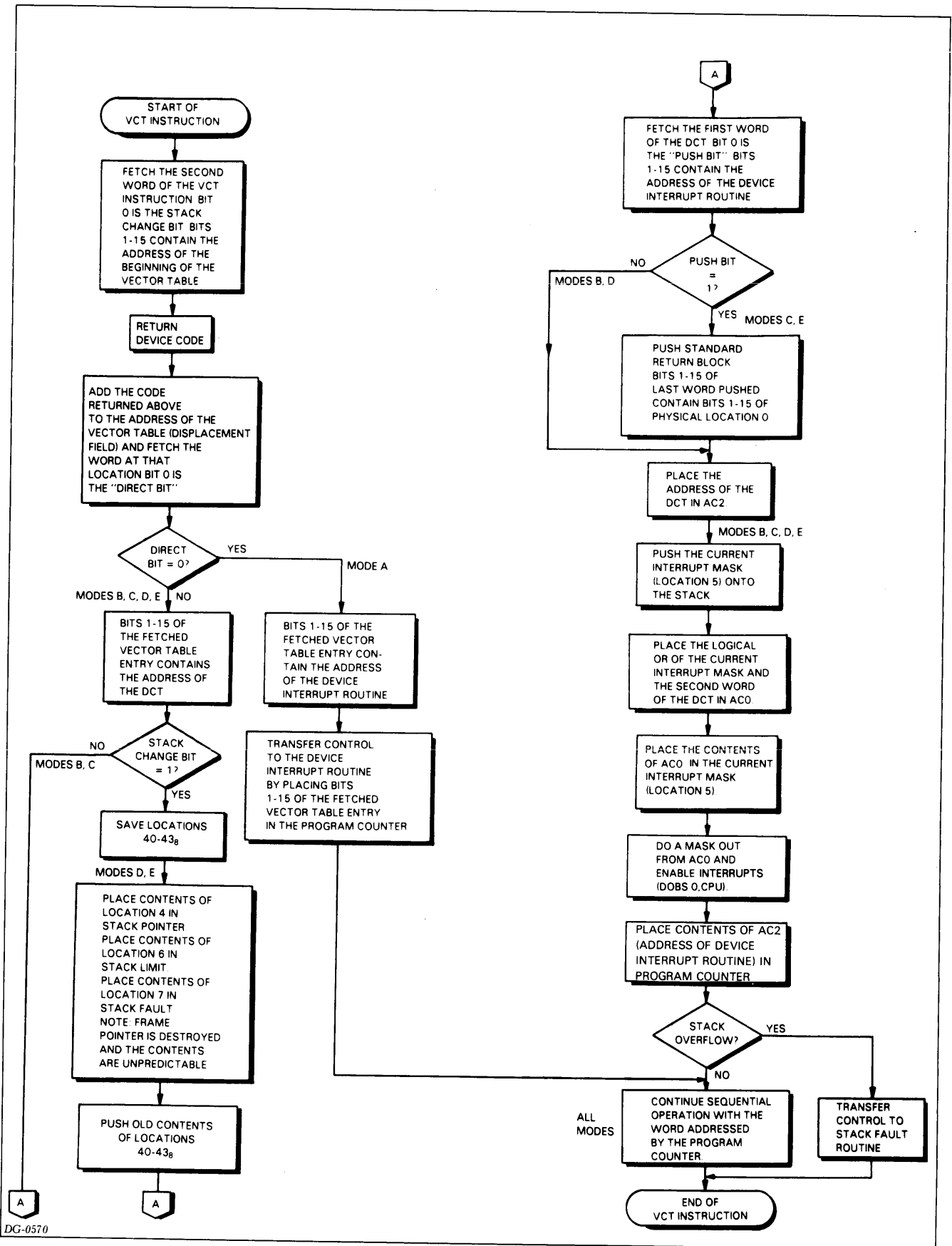
Figure 5.2 Operation of the Vector instruction
