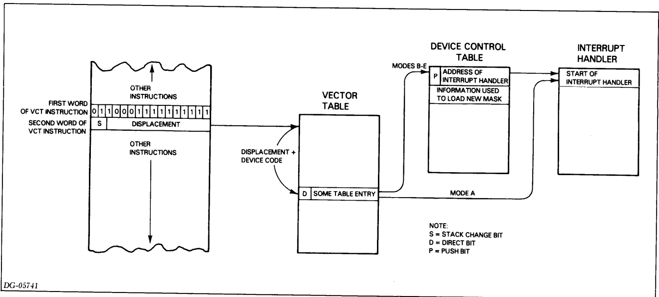
Figure 5.1 Overview of the Vector instruction
