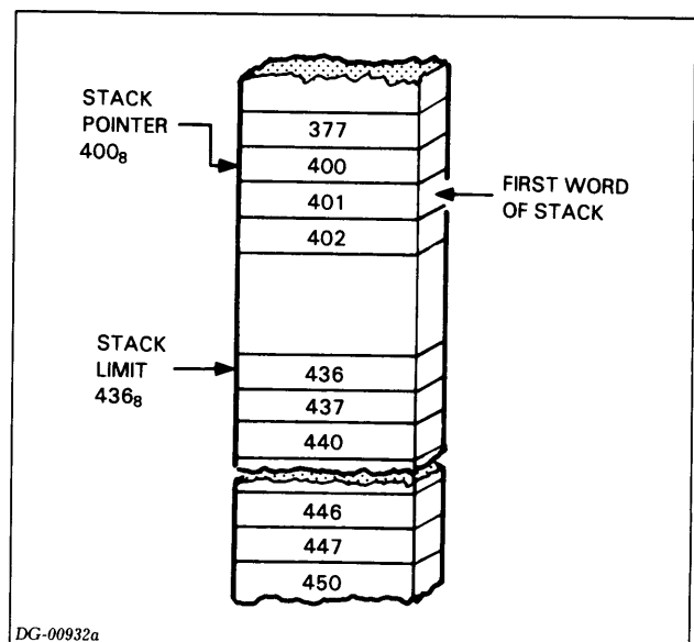
Figure 2.8 Underflow protected stack area
