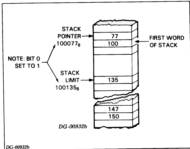
Figure 2.9 Overflow protected page zero stack area
