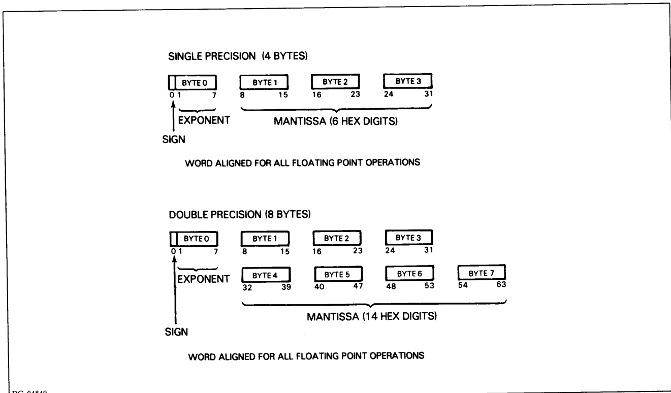
Figure 3.1 Floating point format
