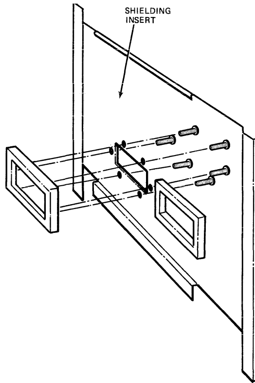
Figure 4-11 Mounting the Cable Trough to the Shielding Insert
