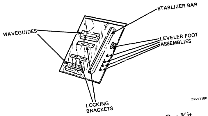
Figure 4-6 Cable Trough/Stabilizer Bar Kit
