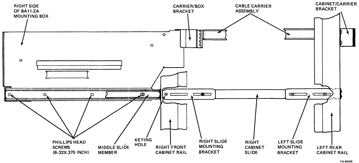
Figure 5-4 Mounting the BA11-Z Mounting Box to the Cabinet Slides
