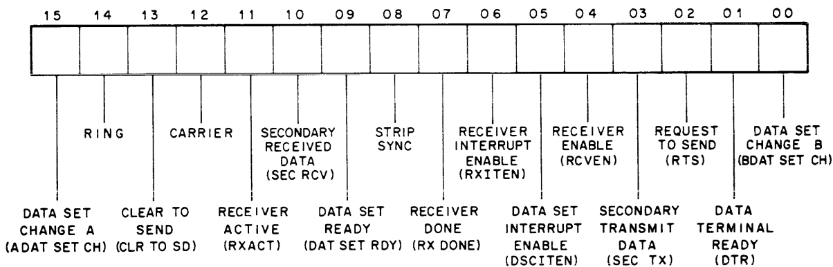
Figure 3-2 Receiver Control and Status Register Format
