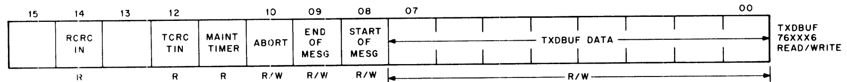
Figure 3-1 DUP11 Register Configurations and Bit Assignments
