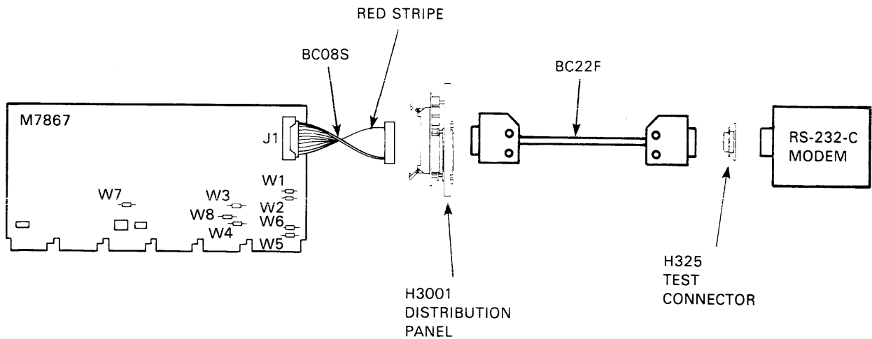
Figure 2-3 DUP11 Cabling
