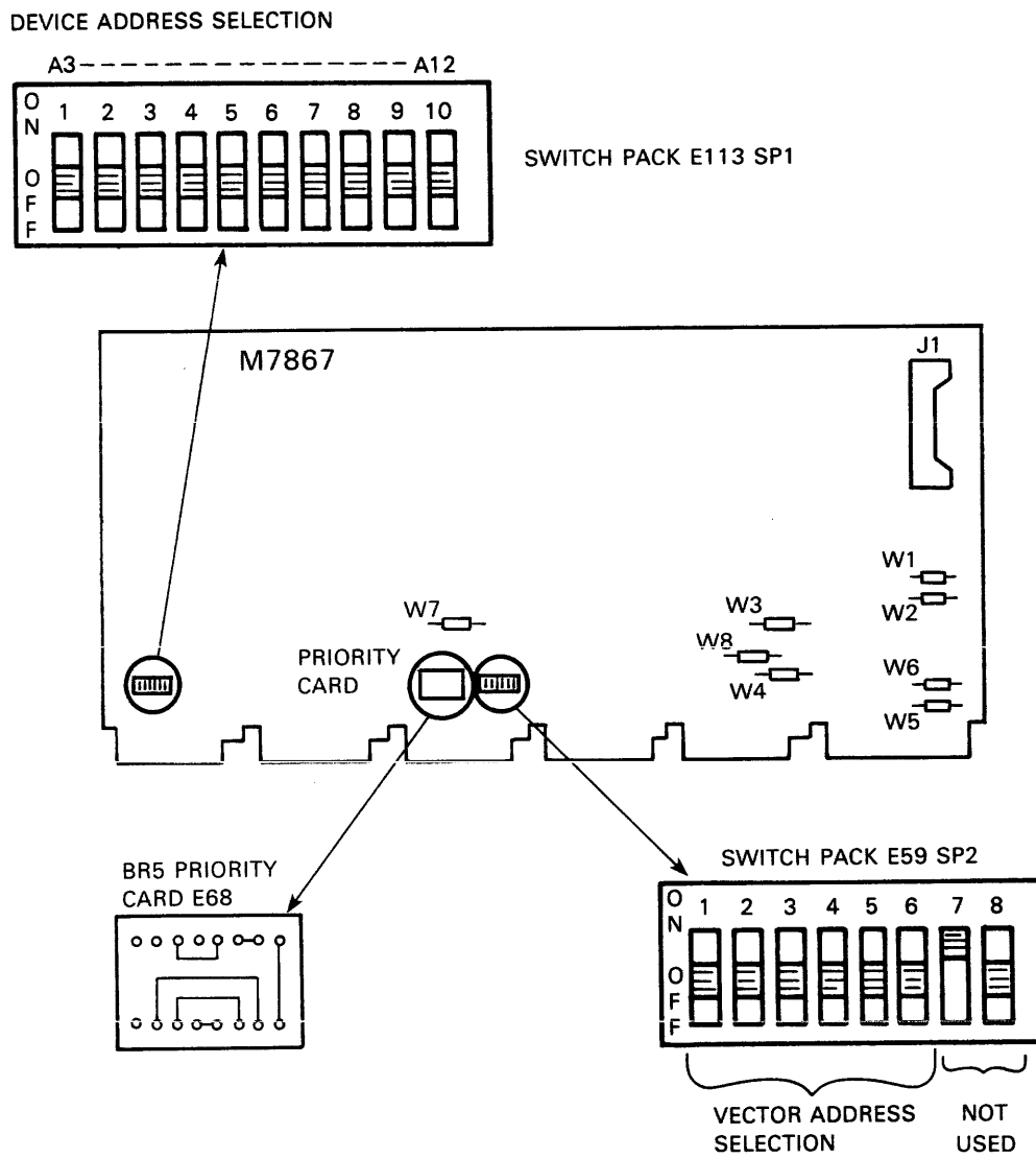
Figure 2-2 Component Location
