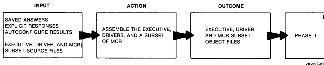
Figure 4-1 Processing Steps in SYSGEN Phase I
