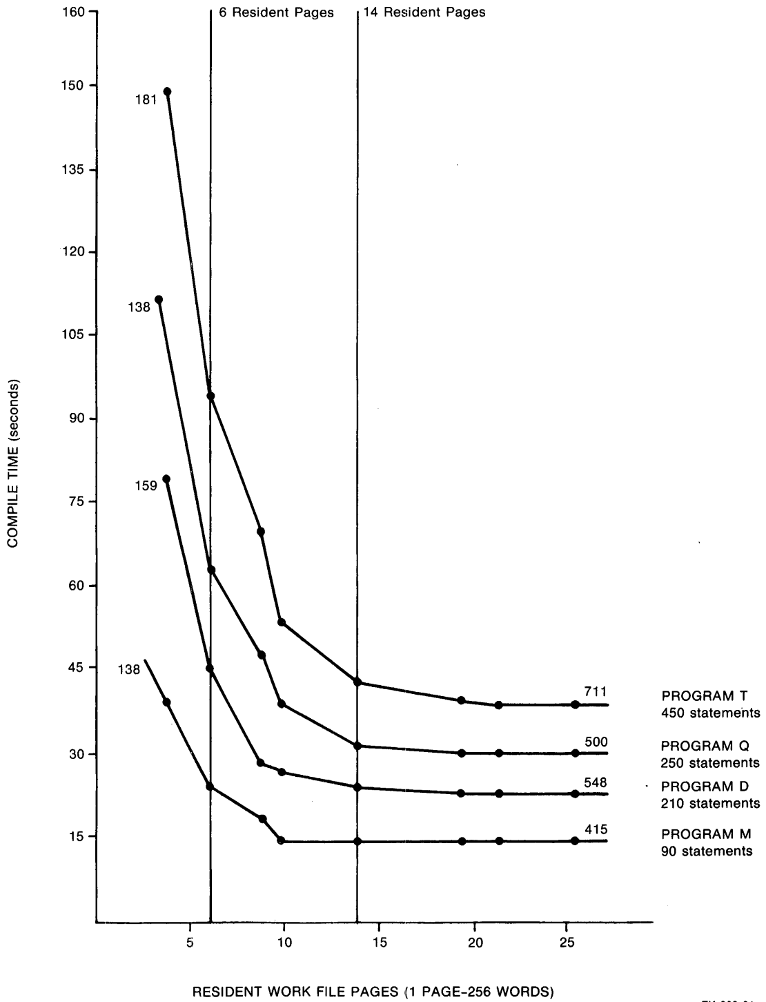
Figure 3-1 Compiler Performance
