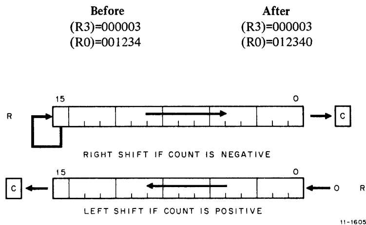
Figure 3-3 ASH Operation
