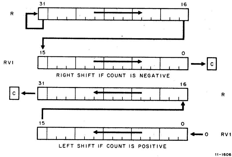
Figure 3-4 ASHC Operation
