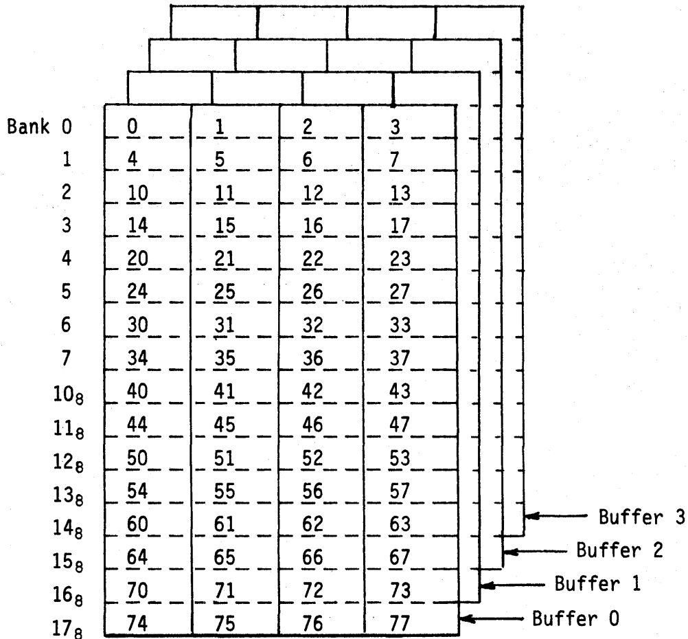
Figure 3-7 Instruction buffers
