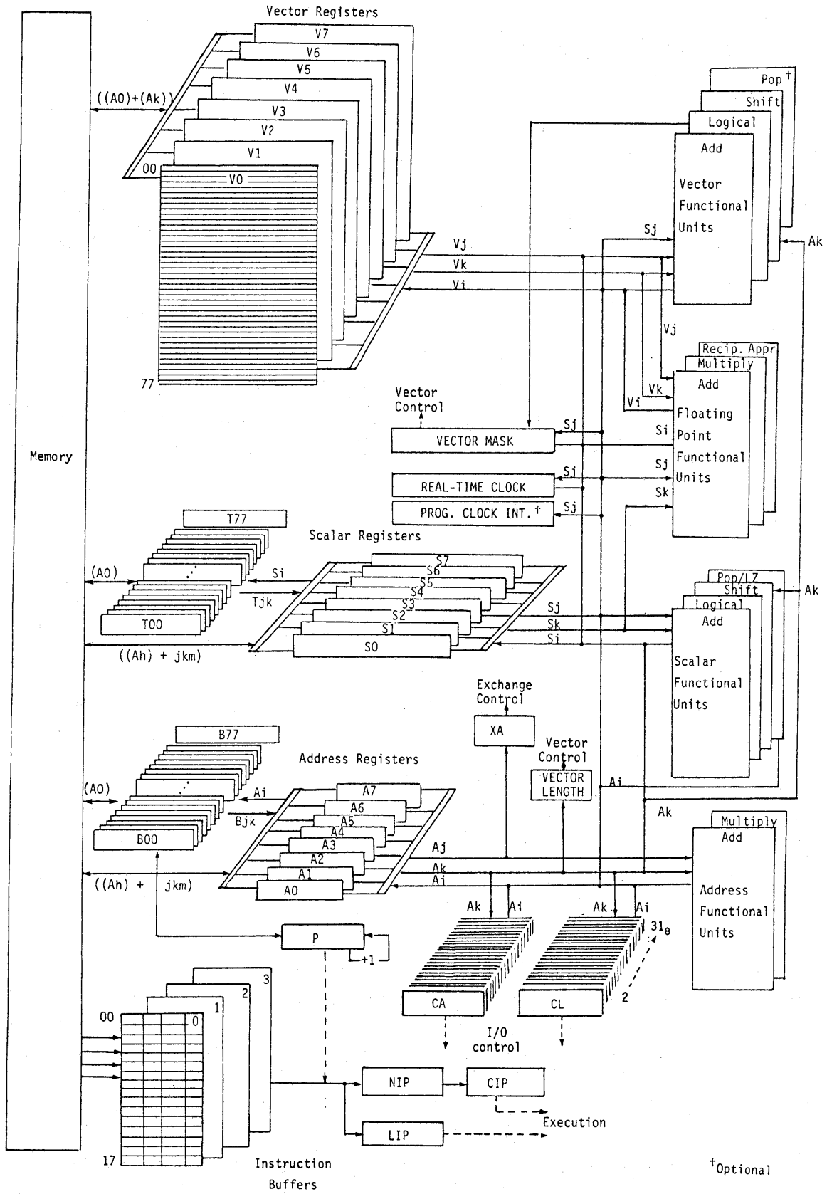
Figure 3-1. Computation section
