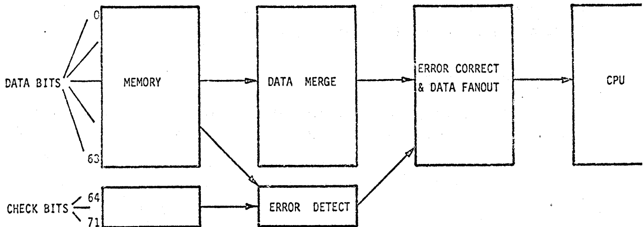
Figure 5-2. Memory data path with SECDED
