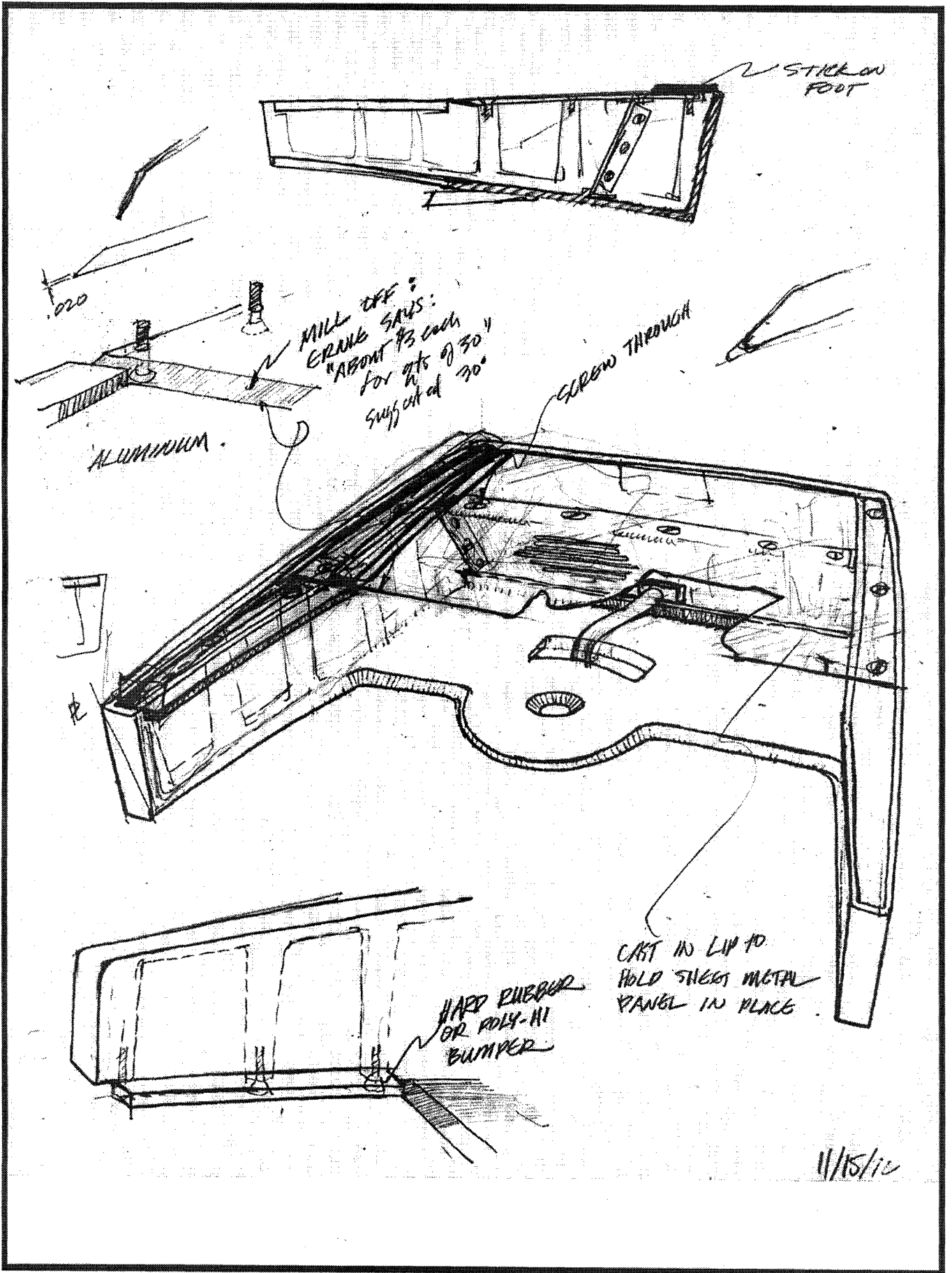
MANUFACTURING THE BASE
