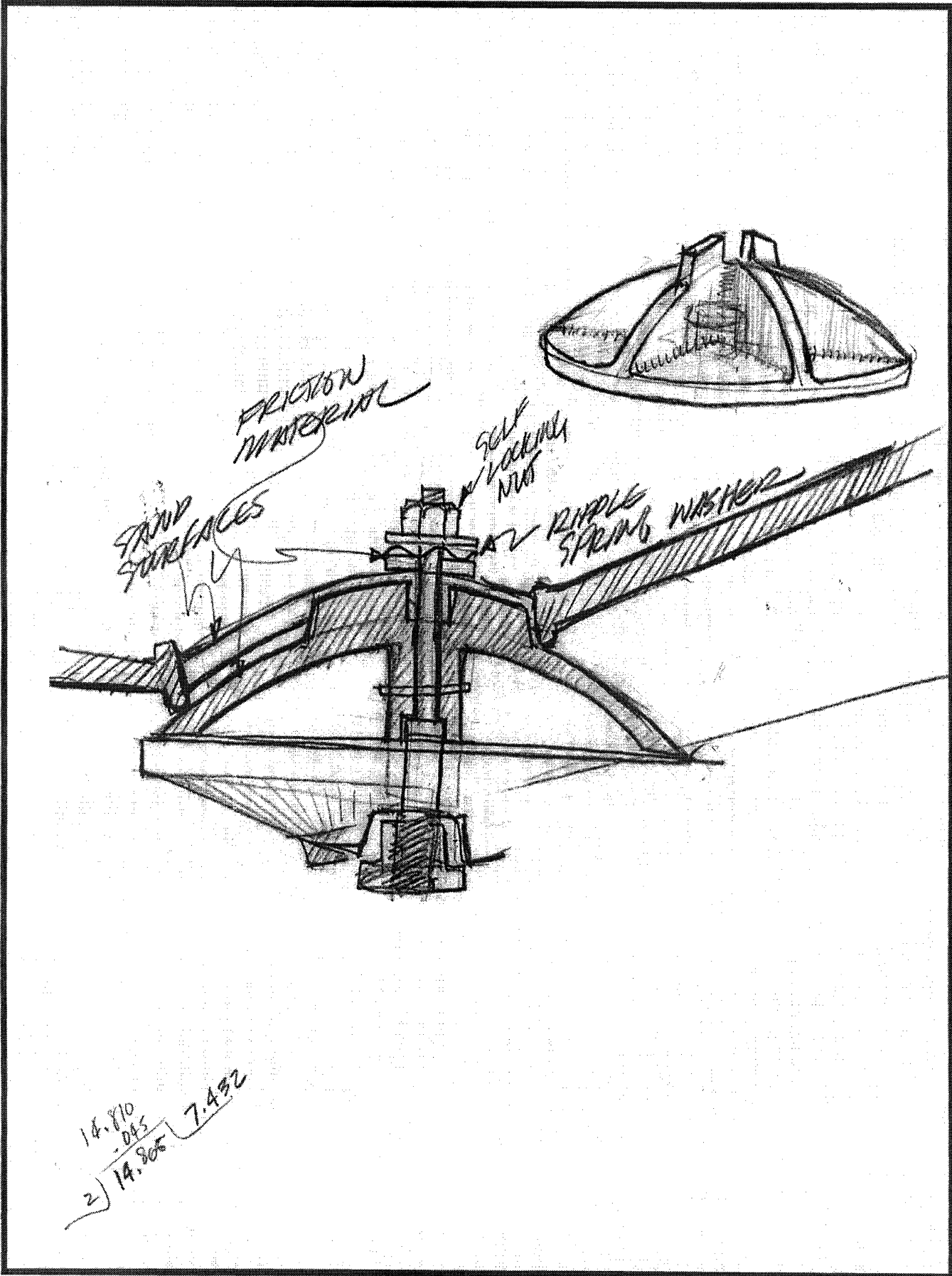
THE ROTILTER PRODUCTION DETAILS
