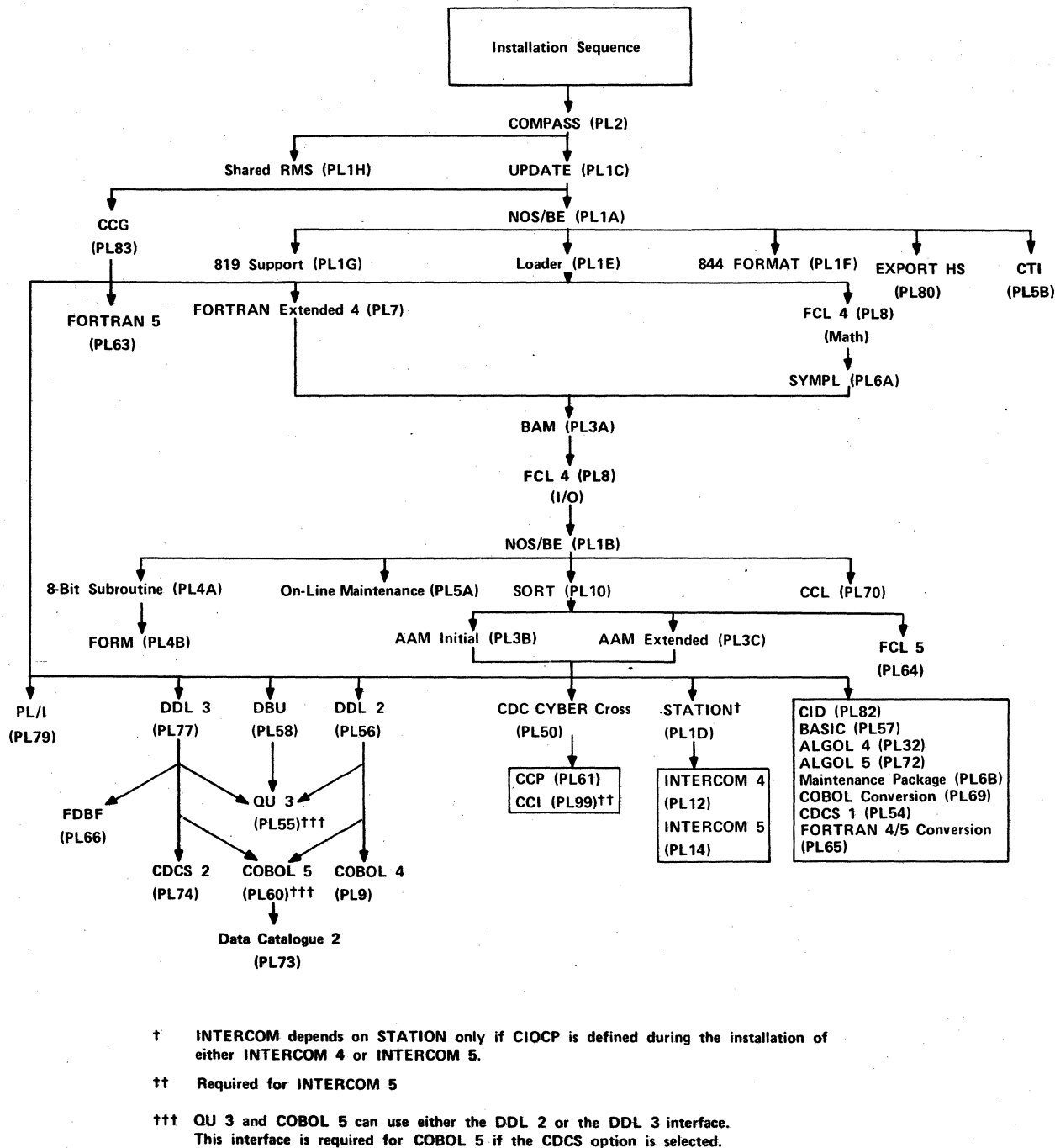
Figure I-1-1. Installation Sequence
