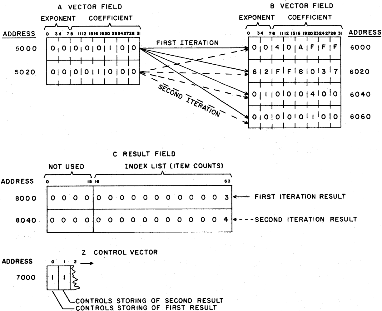
Figure 6-84. Example of Search EQ; A = B, Index List → C
