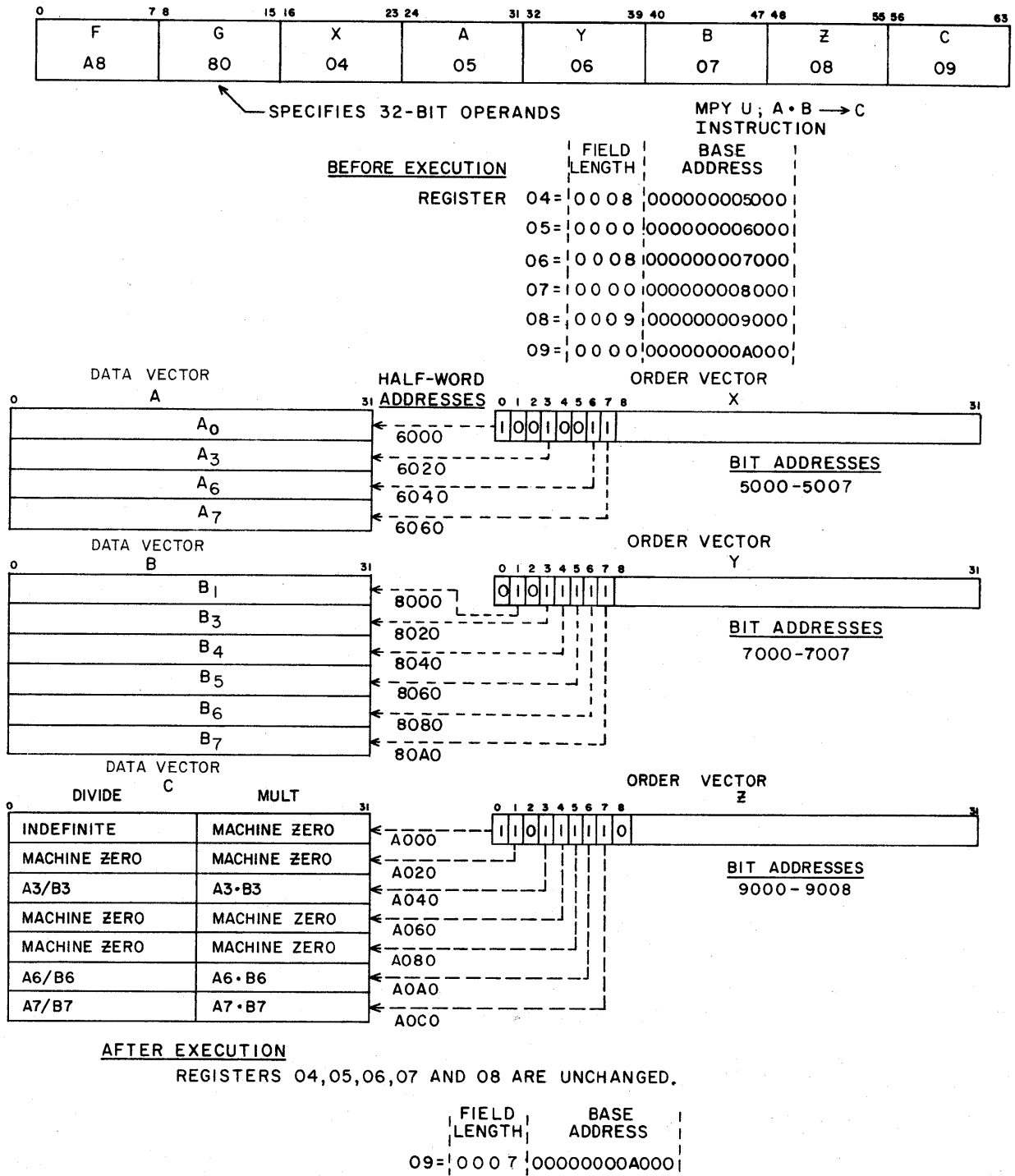
Figure 6-33. Example of a Div or Mpy U Sparse Vector Instruction when G Bit 1 = 0 and G Bit 2 = 1
