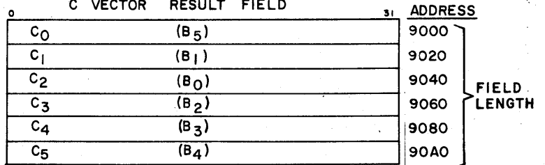
Figure 6-39. Example of Transmit Indexed List →C Instruction
