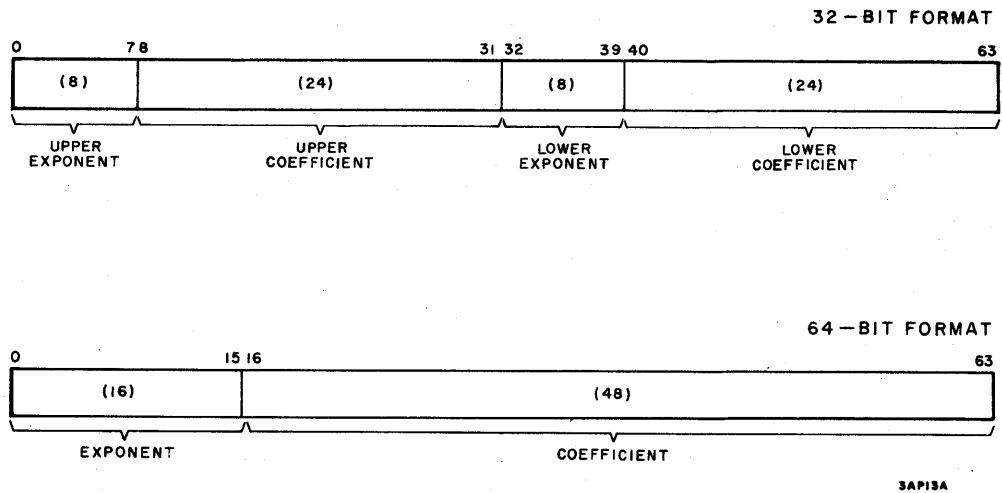
Figure 3-5. Operand Formats
