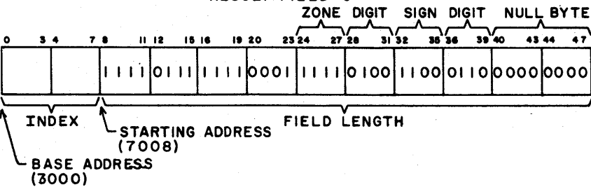
Figure 6-62. Example of Merge Per Byte Mask A, B Per G→C Instruction
