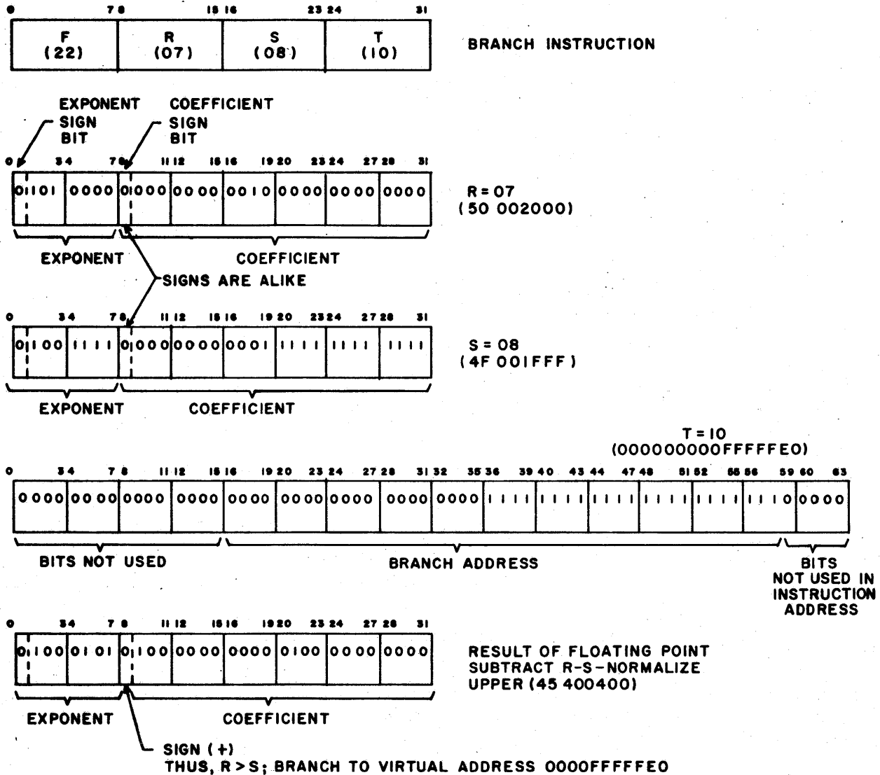
Figure B-4. Example of Branch if (R) \geq (S) (32/64 Bit FP) Instruction
