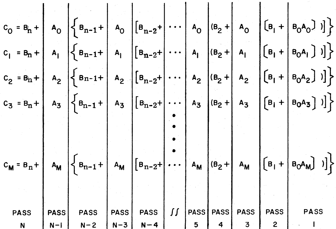
Figure 6-38. Basic Arithmetic Sequence for Polynomial Evaluation Instruction
