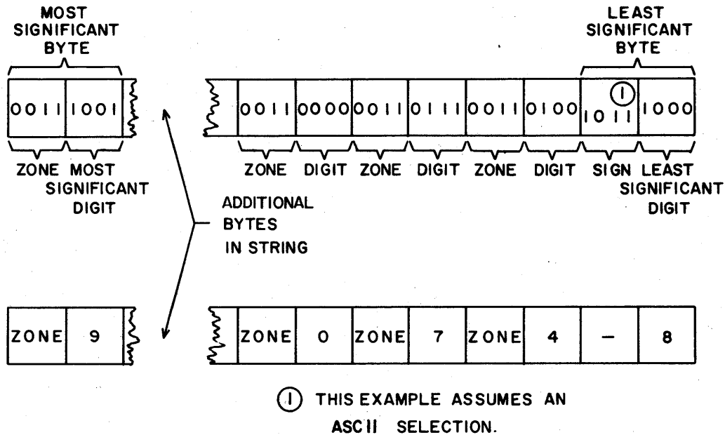
Figure 6-42. Example of the Zoned BCD Format
