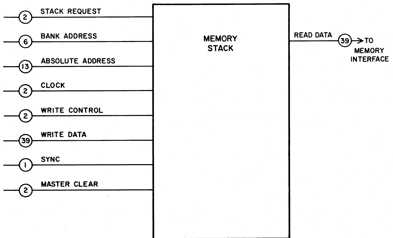
Figure 2-3. Memory Interface/Stack Connections
