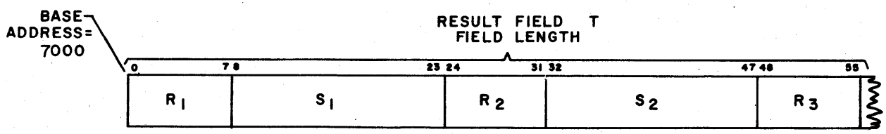
Figure 6-79. Example of Bit Merge Instruction
