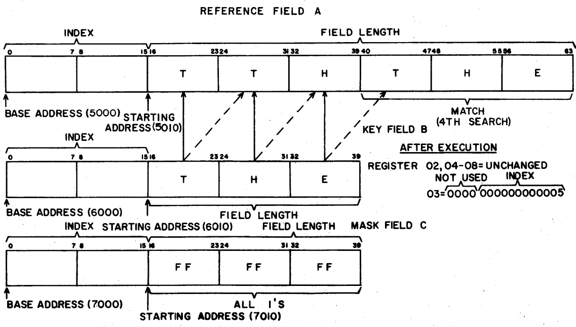
Figure 6-64. Example of Search for Masked Key Byte; A, B Per C, G Instruction
