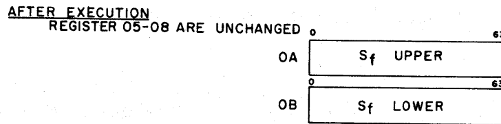
Figure 6-82. Example of Sparse Dot Product to (C) and (C+1) Instruction
