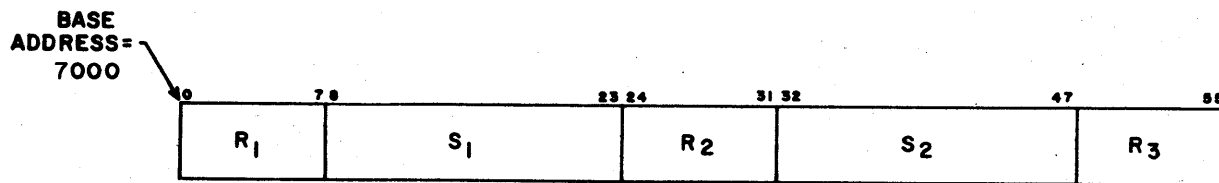
Figure 6-80. Example of Bit Mask Instruction
