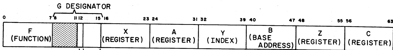
FORMAT B USED FOR THE 33 BRANCH INSTRUCTION
