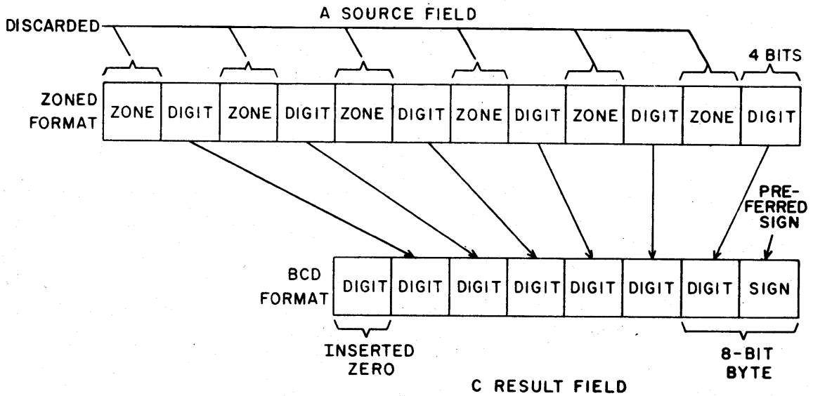
Figure 6-52. Example of Zoned to BCD Format Conversion (G Bit 0 = 1 and G Bit 1 = 1)
