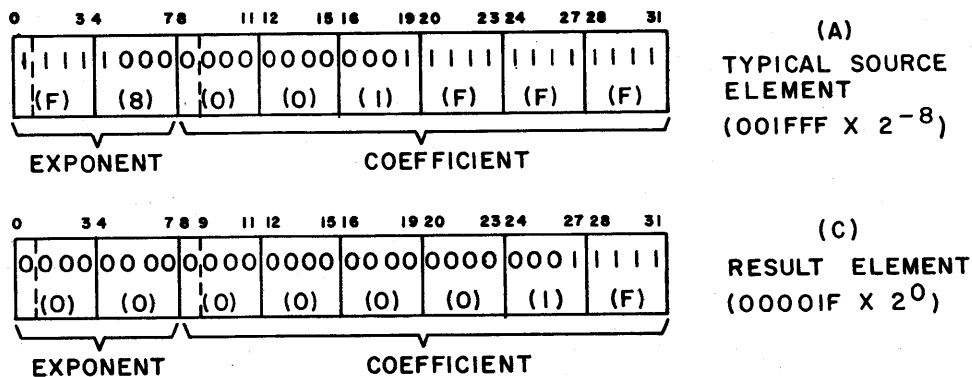
Figure 6-23. Example of Source and Result Elements for a Truncate A → C Instruction
