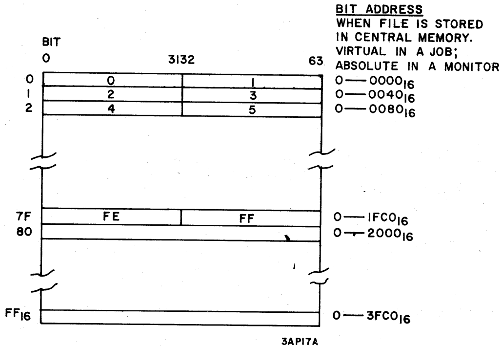
Figure 5-8. Register File
