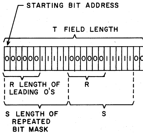
Figure 6-92. Example of Repeated Bit Mask Data Format (Leading Zeros)
