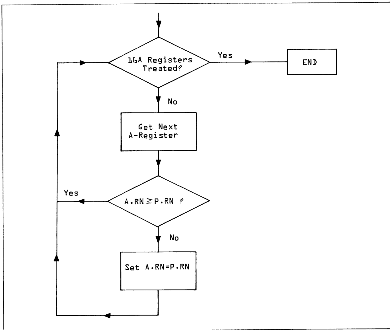
Figure 7-7. Rippling
