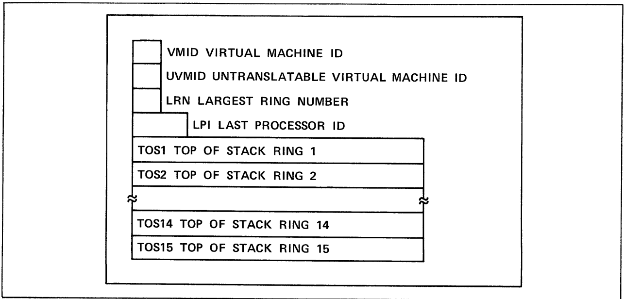
Figure 5-7. Process State Registers Accessed by Exchange Operation
