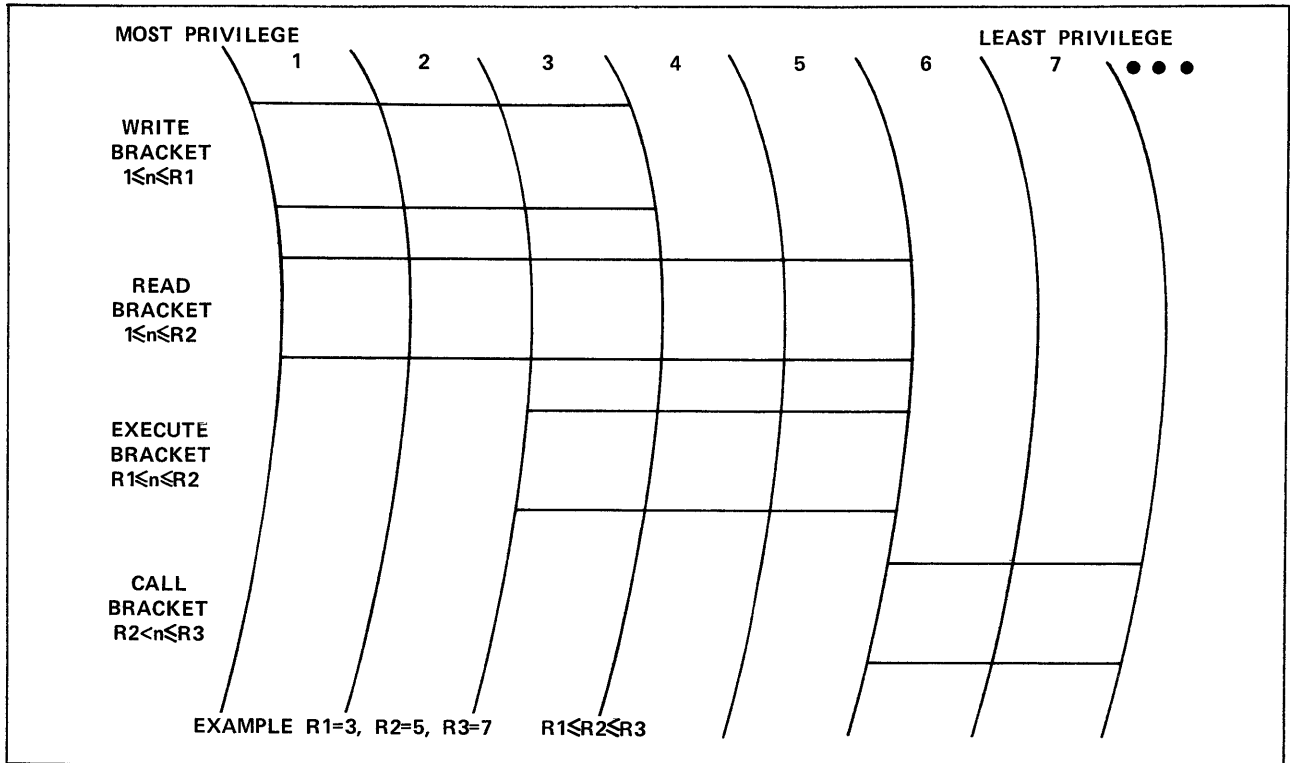
Figure 3-5. Ring Brackets
