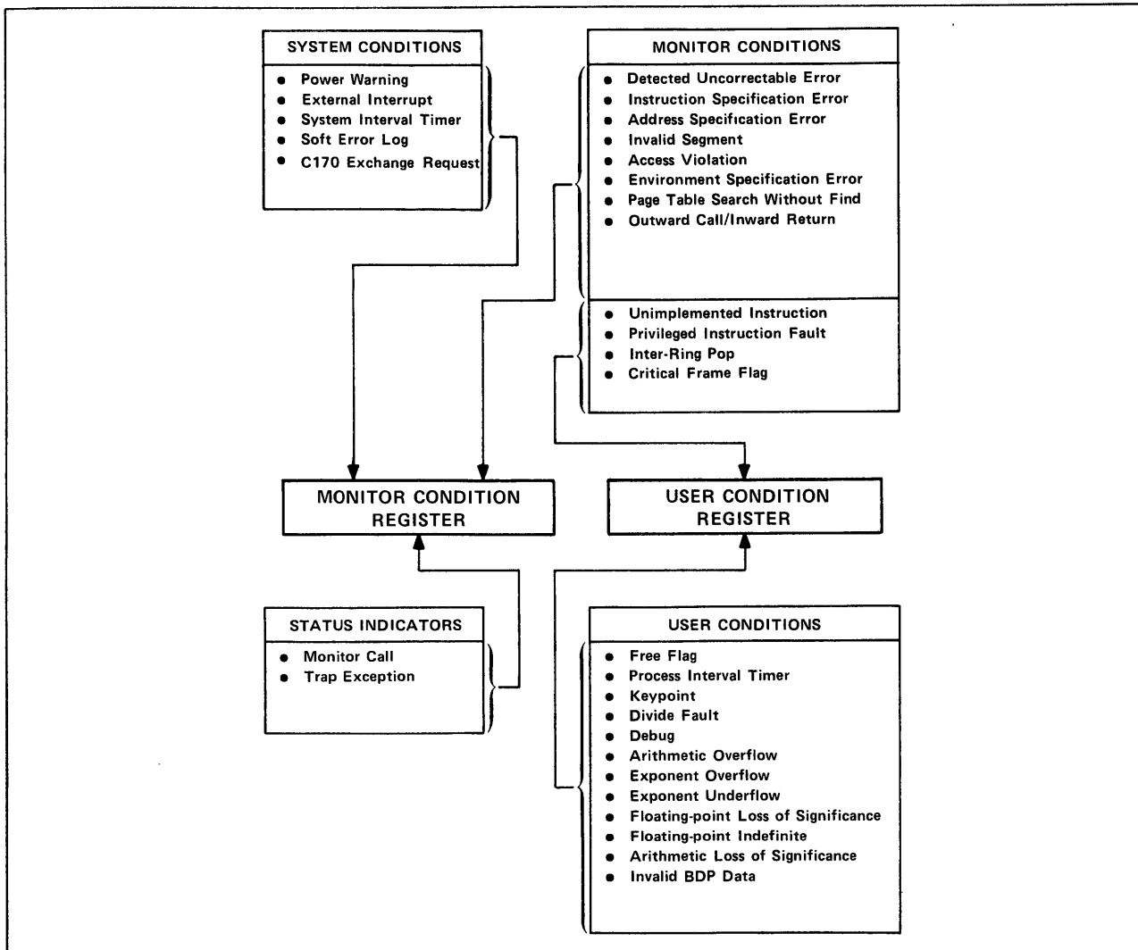
Figure 6-2. Interrupt Conditions
