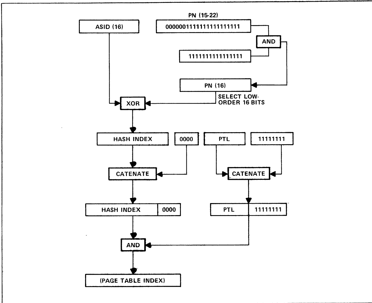
Figure 2-4. Hashing Algorithm
