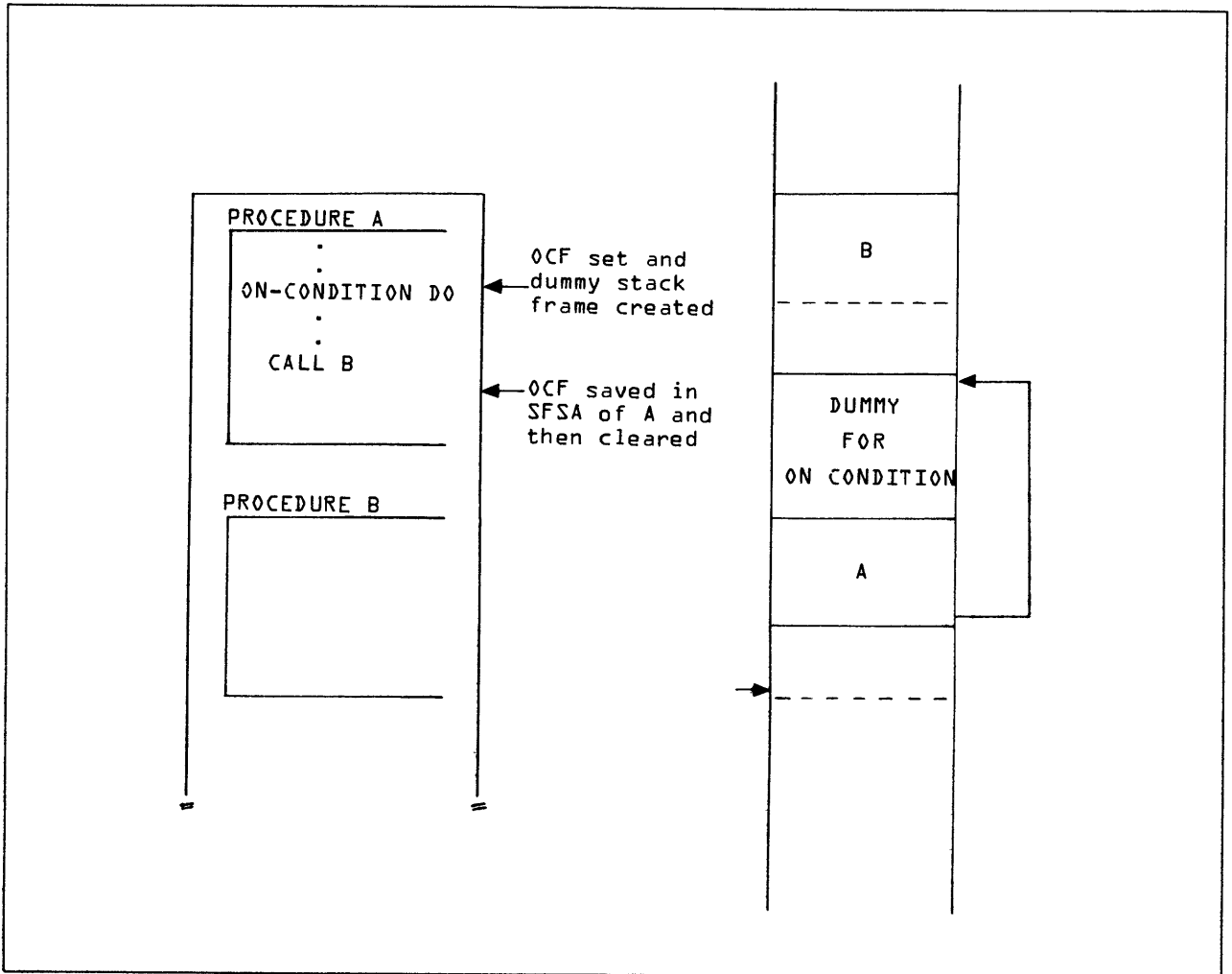
Figure 7-12. On-Condition Handling
