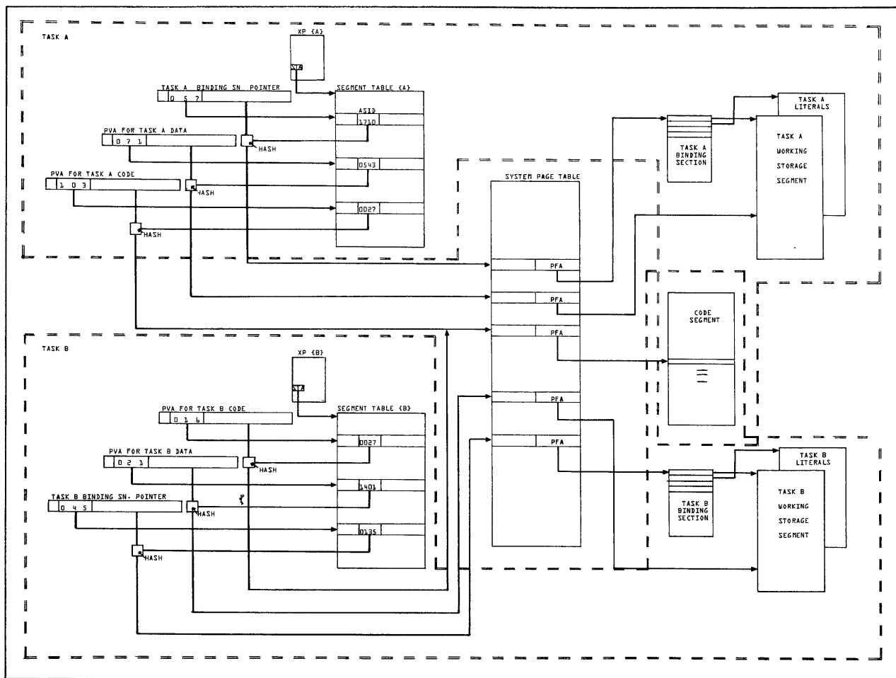
Figure 7-10. Code Sharing
