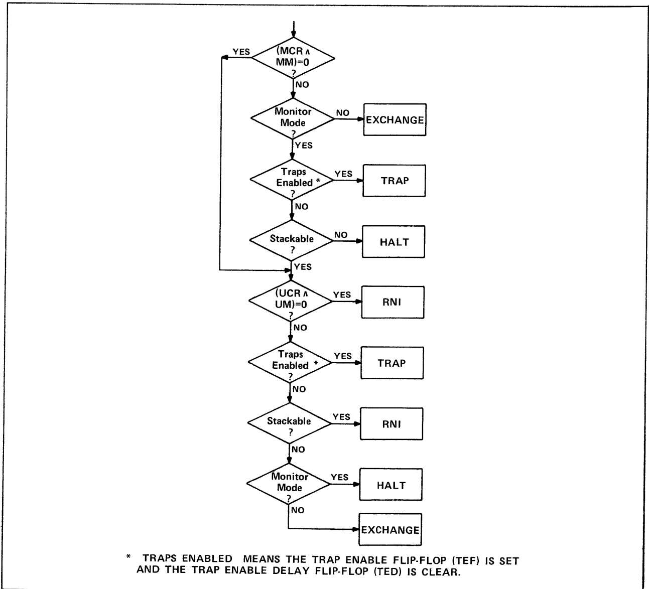
Figure 6-4. Interrupt Flowchart
