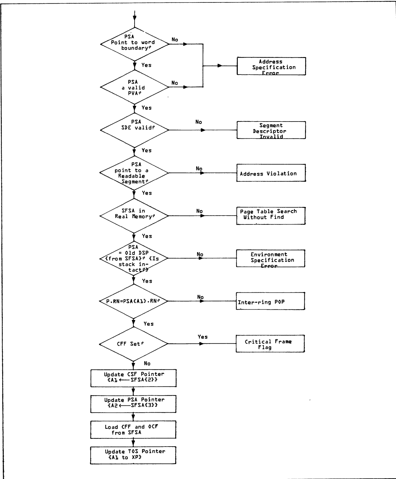
Figure 7-22. Pop
