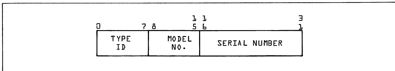
Figure 5-3. EID Register
