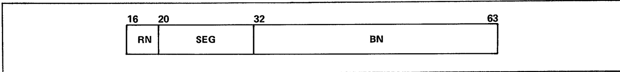
Figure 3-8. Process Virtual Address (PVA)
