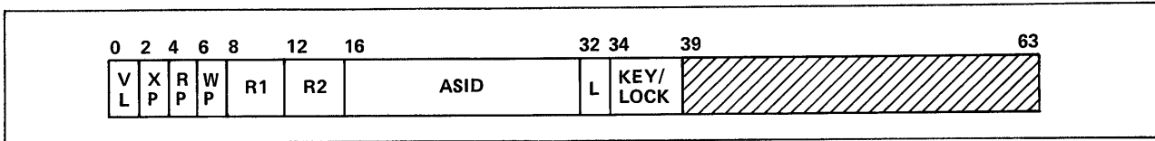
Figure 3-3. Segment Descriptor Table Entry (SDE)
