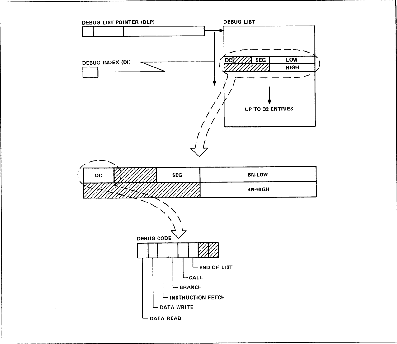
Figure 10-1. Debug List
