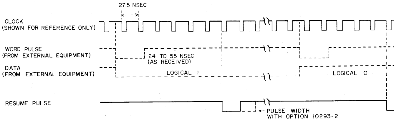
Figure 5-18. Input Channel Timing
