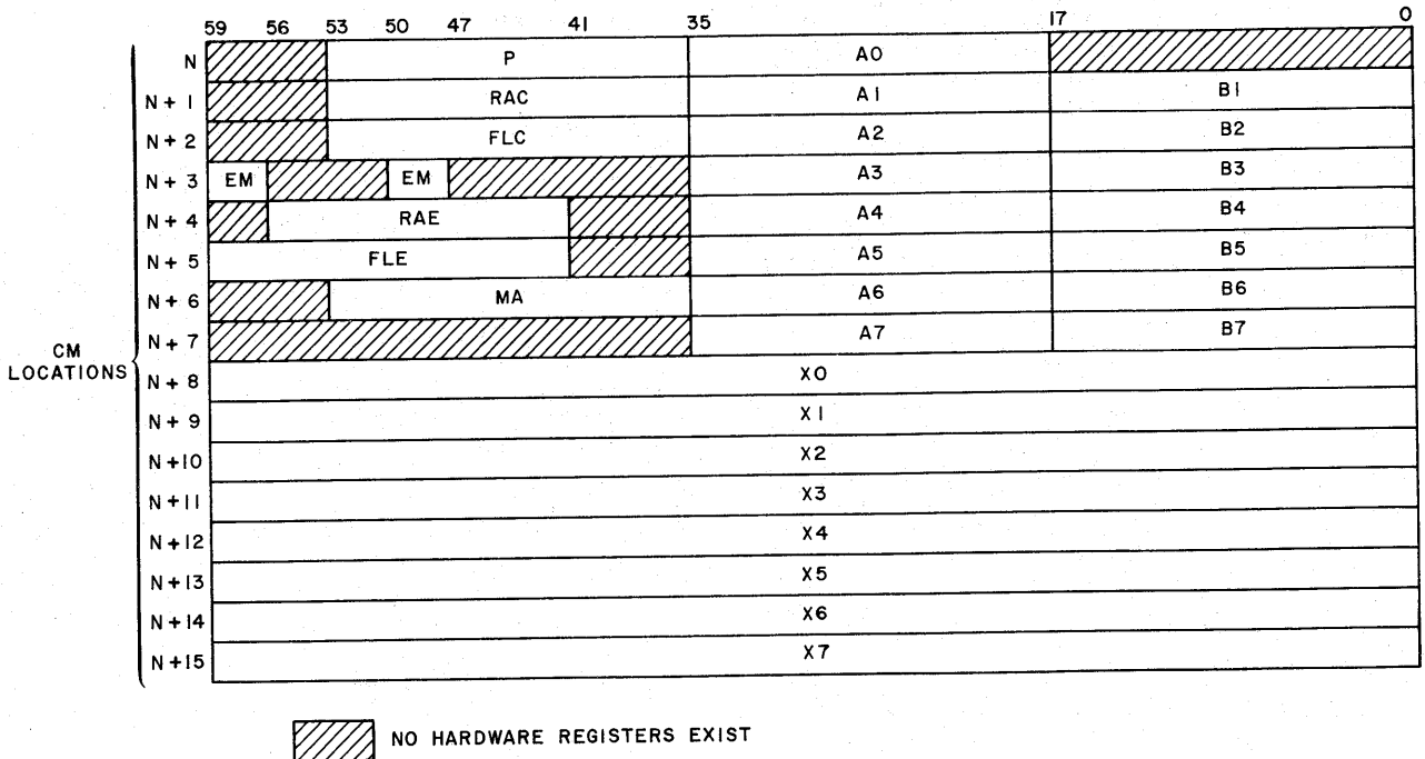
Figure 5-1. Exchange Package - Models 720 through 760
