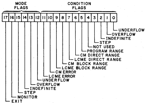
Figure 2-2. PSD Register Flag Bit Arrangement
