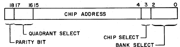
Figure 2-6. Models 720 through 760 CM Address Format
