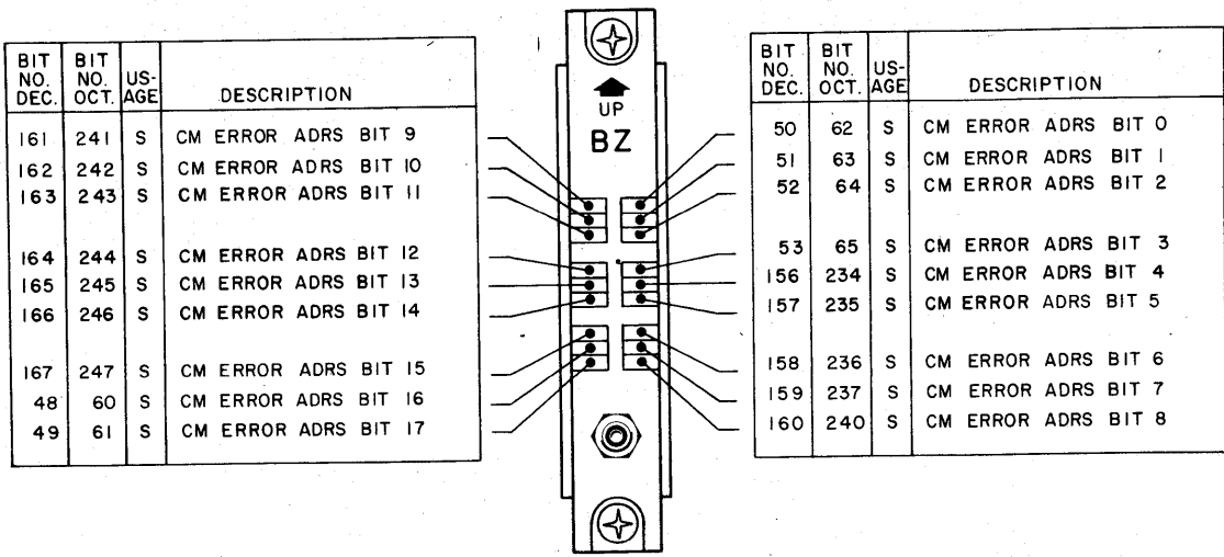
Figure 3-32. PPS-0 Module at 2F41 - Model 176
