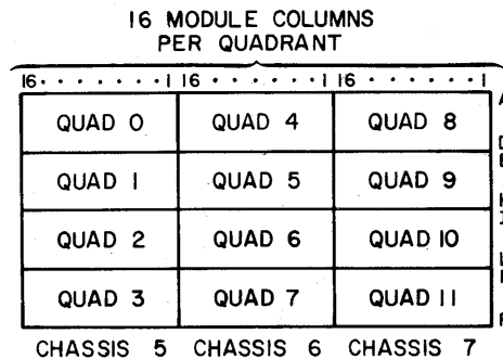
Figure 5-23. CP Chassis Quadrants (Viewed from Module Side) - Models 740, 750, and 760
