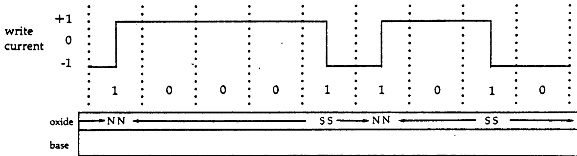
Figure 6-4: NRZI (Non Return to Zero—Invert on ones)
