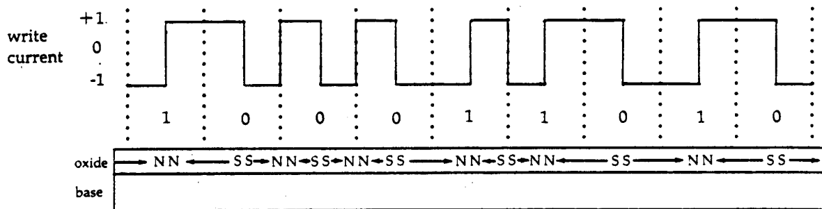
Figure 6-5: Phase Encoding
