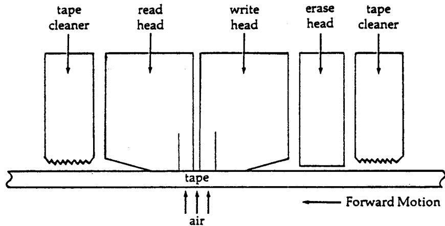
Figure 6-1: Read-Write Unit
