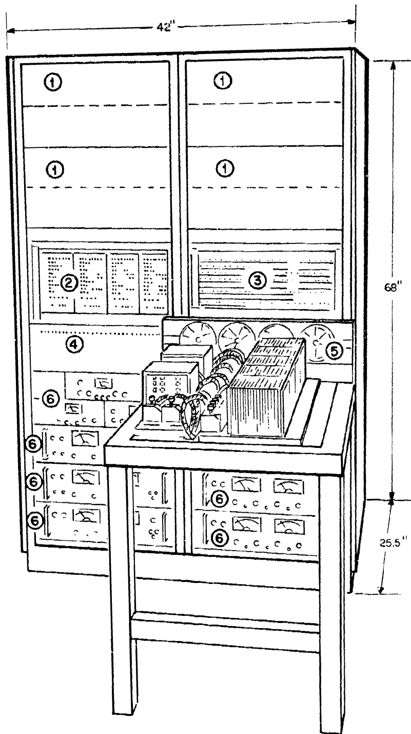
Figure 28. Aerospace Multiprocessor Configuration
