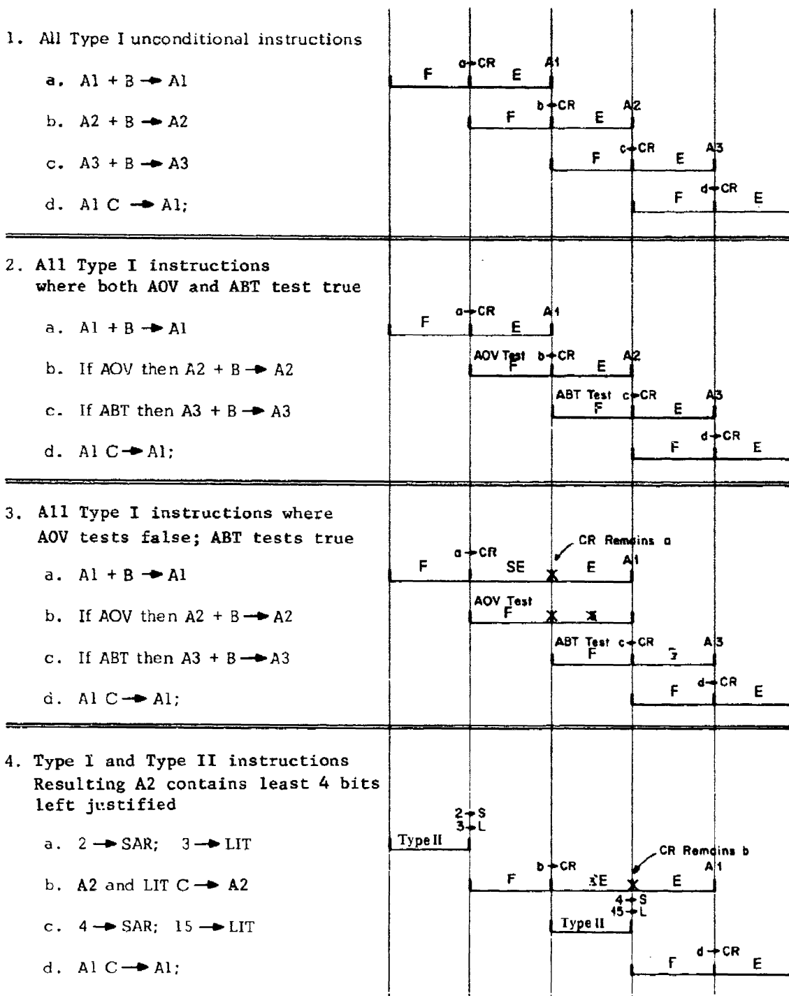
Figure 39. Timing Example
