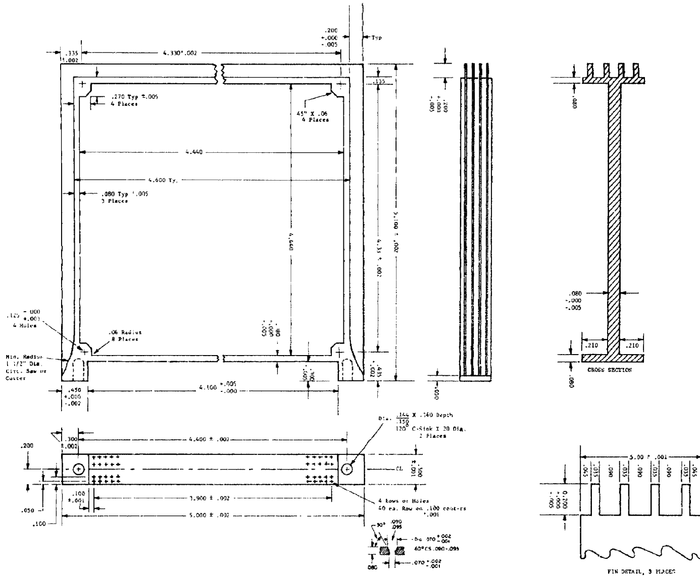
Figure 29. Submodule Housing
