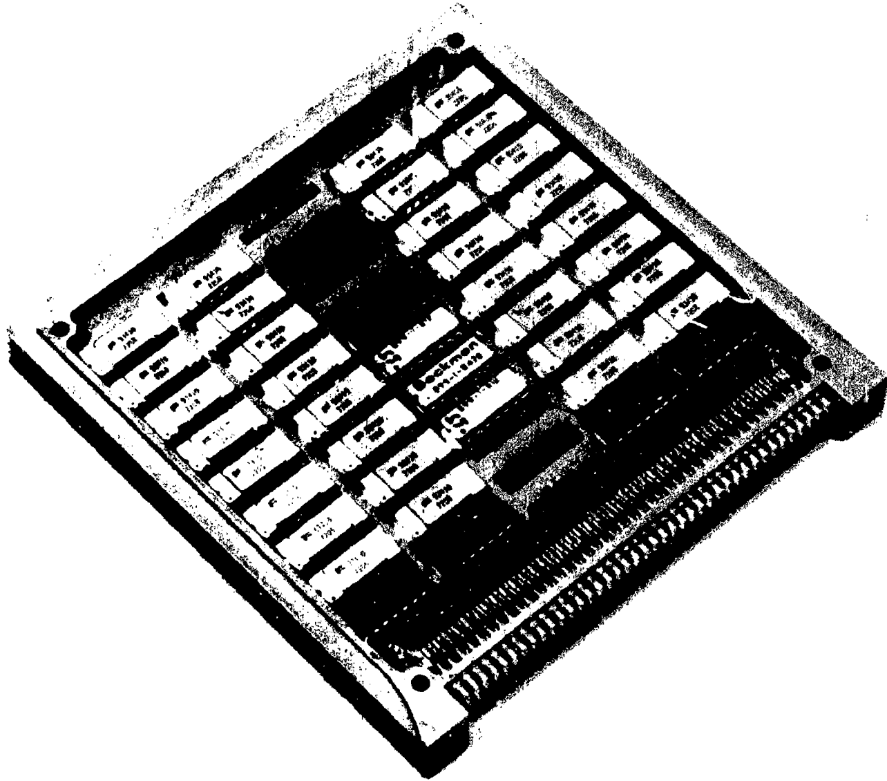
Figure 33. Microprogram Memory, Nanomemory Submodule Packaging
