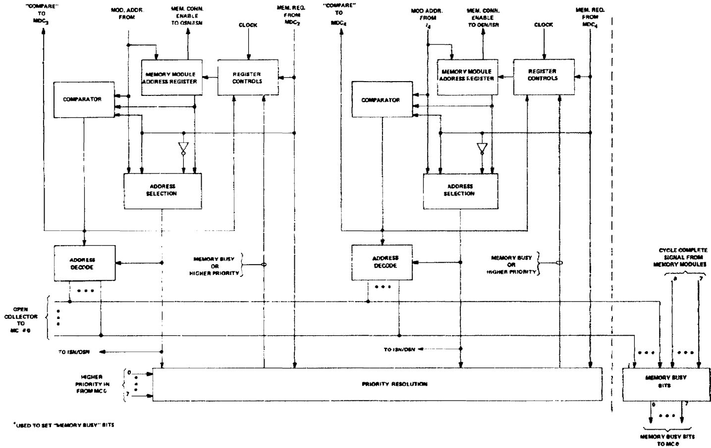
Figure 20. Memory Control No. 1, Block Diagram
