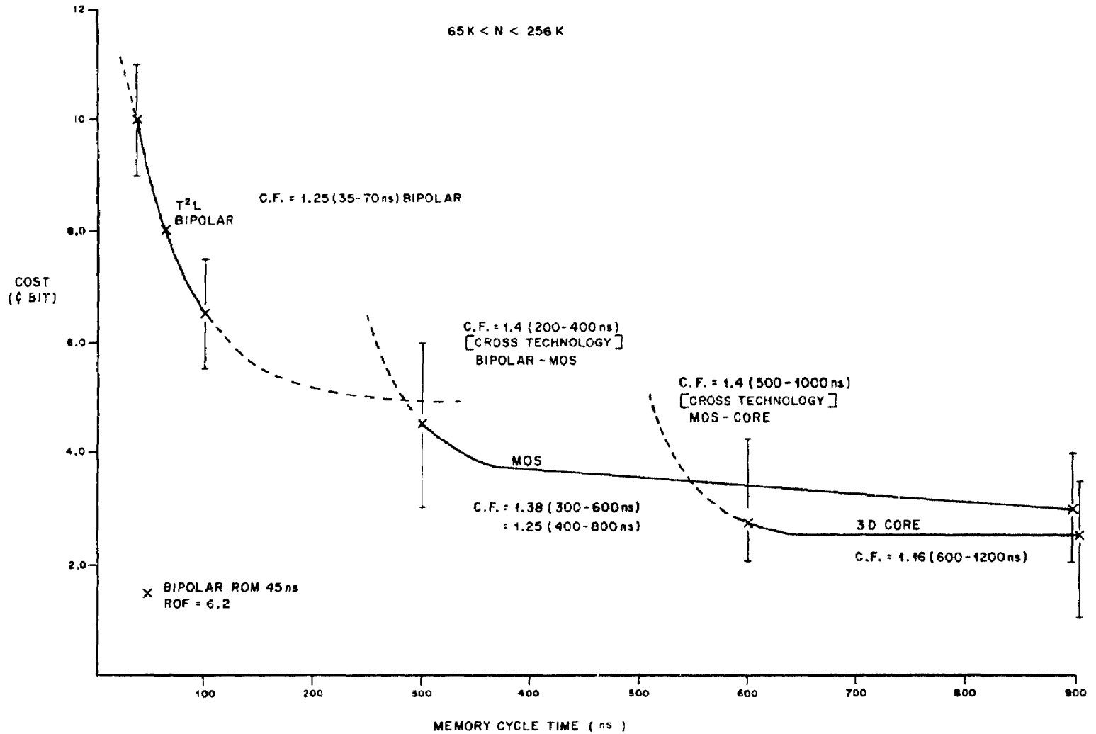
Figure 9. Memory Cost vs. Memory Speed
