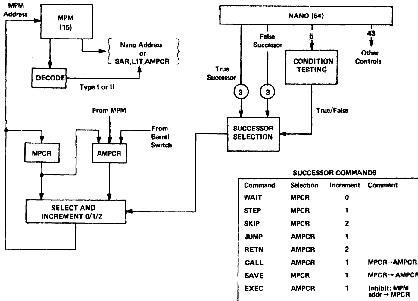
Figure 40. Microprogram Instruction Sequencing
