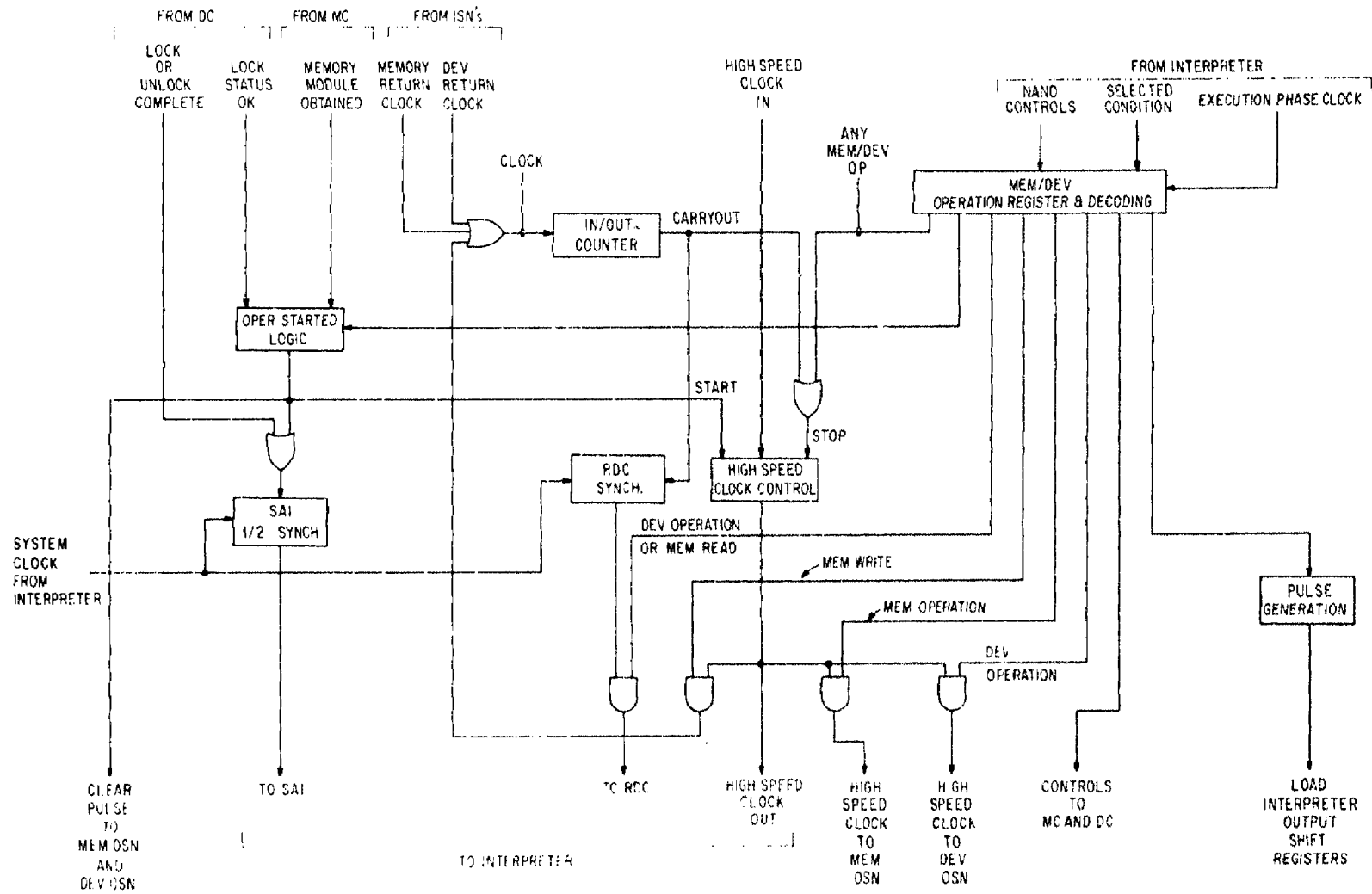
Figure 17. Memory/Device Controls (MDC) Block Diagram
