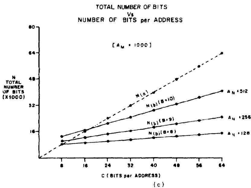
Figure 7. One Memory vs. Two Memory Implementation
