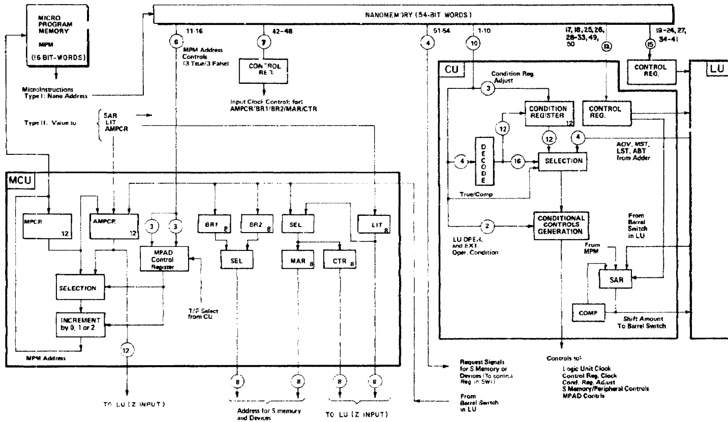
Figure 5. Interpreter Functional Units
