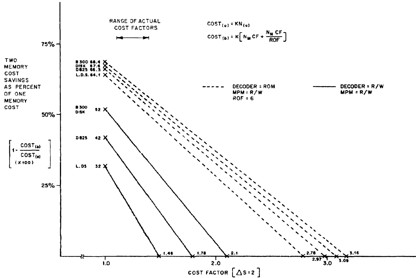
Figure 10. Two Memory Cost Savings vs. Cost Factor
