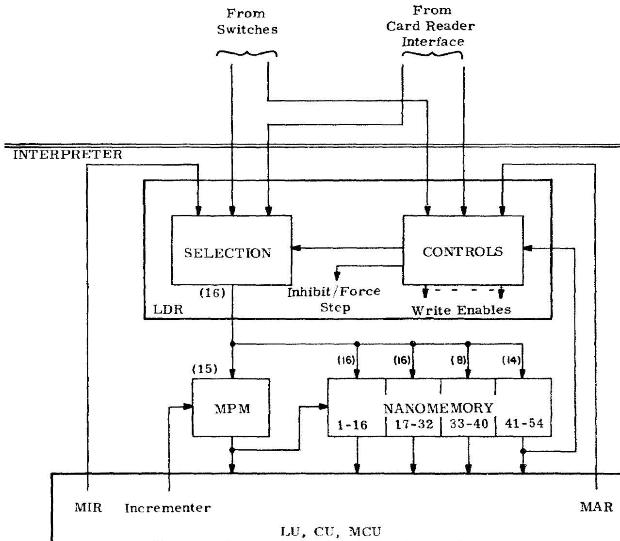
Figure 11. Implementation of Loading Functions Block Diagram
