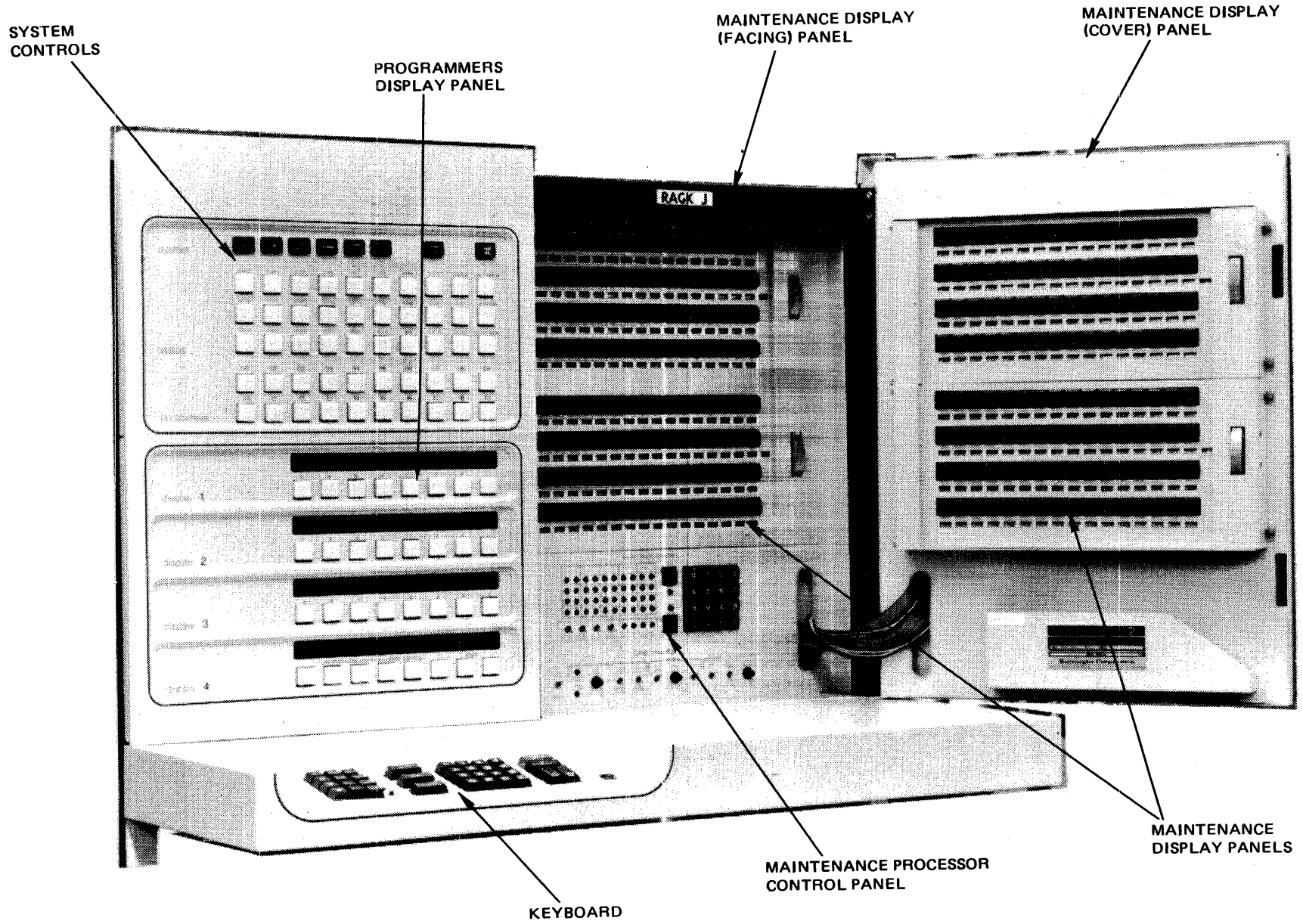
Figure 4-1. System Control and Display Registers
