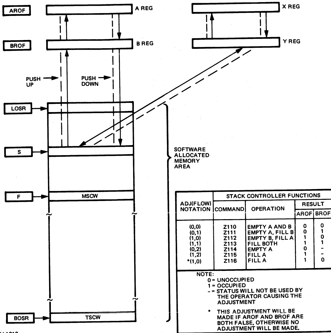
Figure 5-5. Hardware Stack Adjustment
