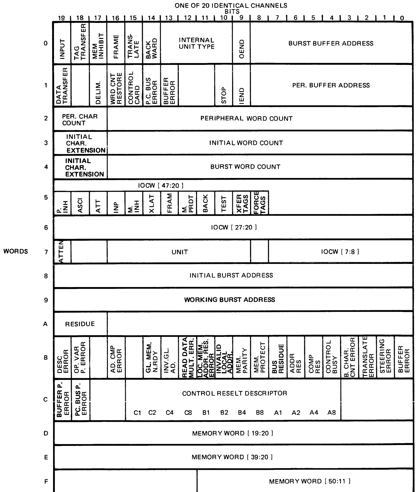
Figure 5-25. Multiplexor Scratch Pad Memory
