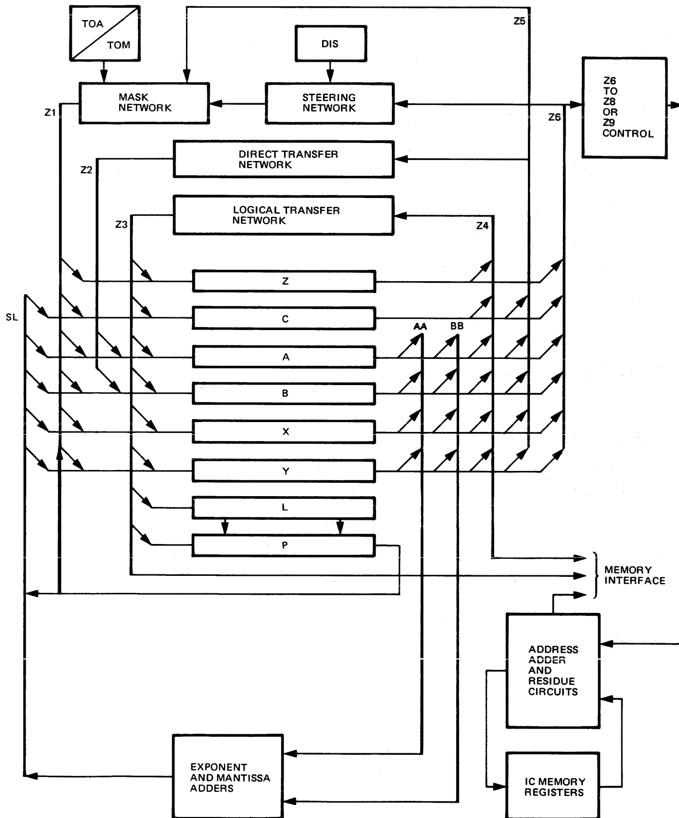
Figure 5-3. Internal Data Transfer Section
