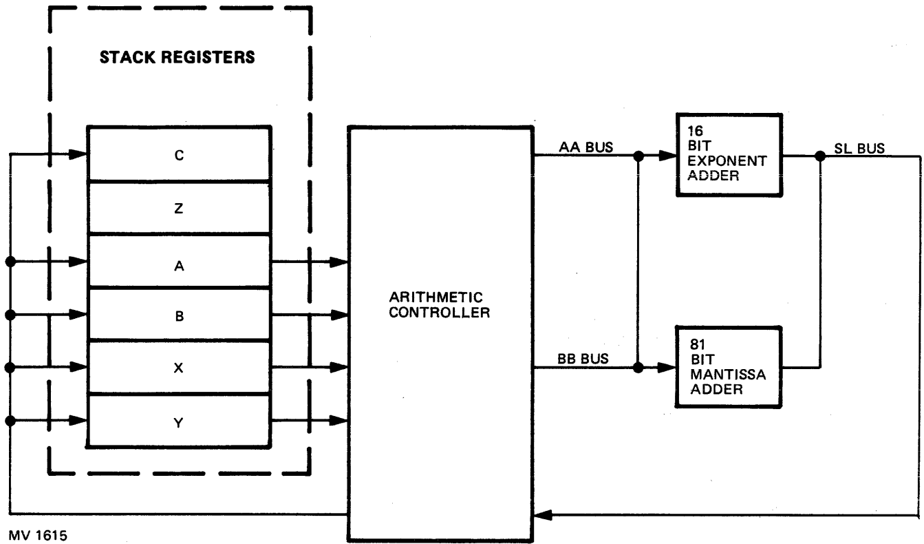
Figure 5-6. Arithmetic Control
