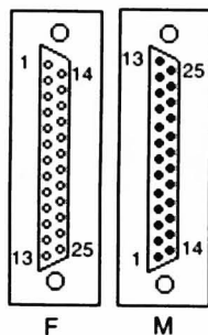
Figure B-1 Comm1—Serial Communication/Printer Ports
