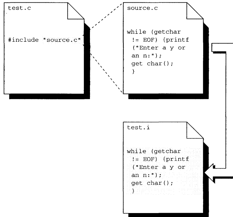
Figure 1-2 Including files
