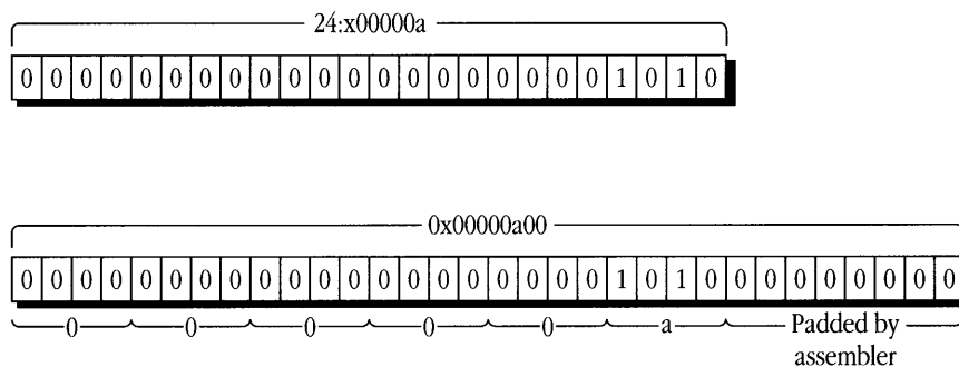
Figure 14-2 Integer boundaries
