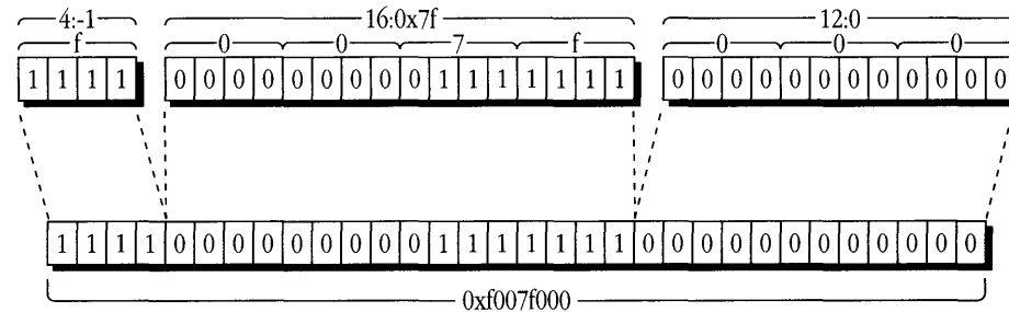
Figure 14-1 Bitfield concatenation
