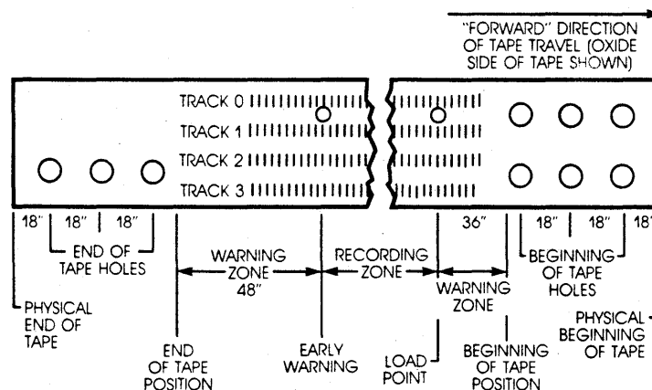
Figure 4-2. 1/4" Tape Layout
