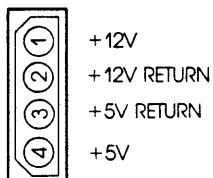
Figure 3-2. Power Connector, J2, Pin Assignments
