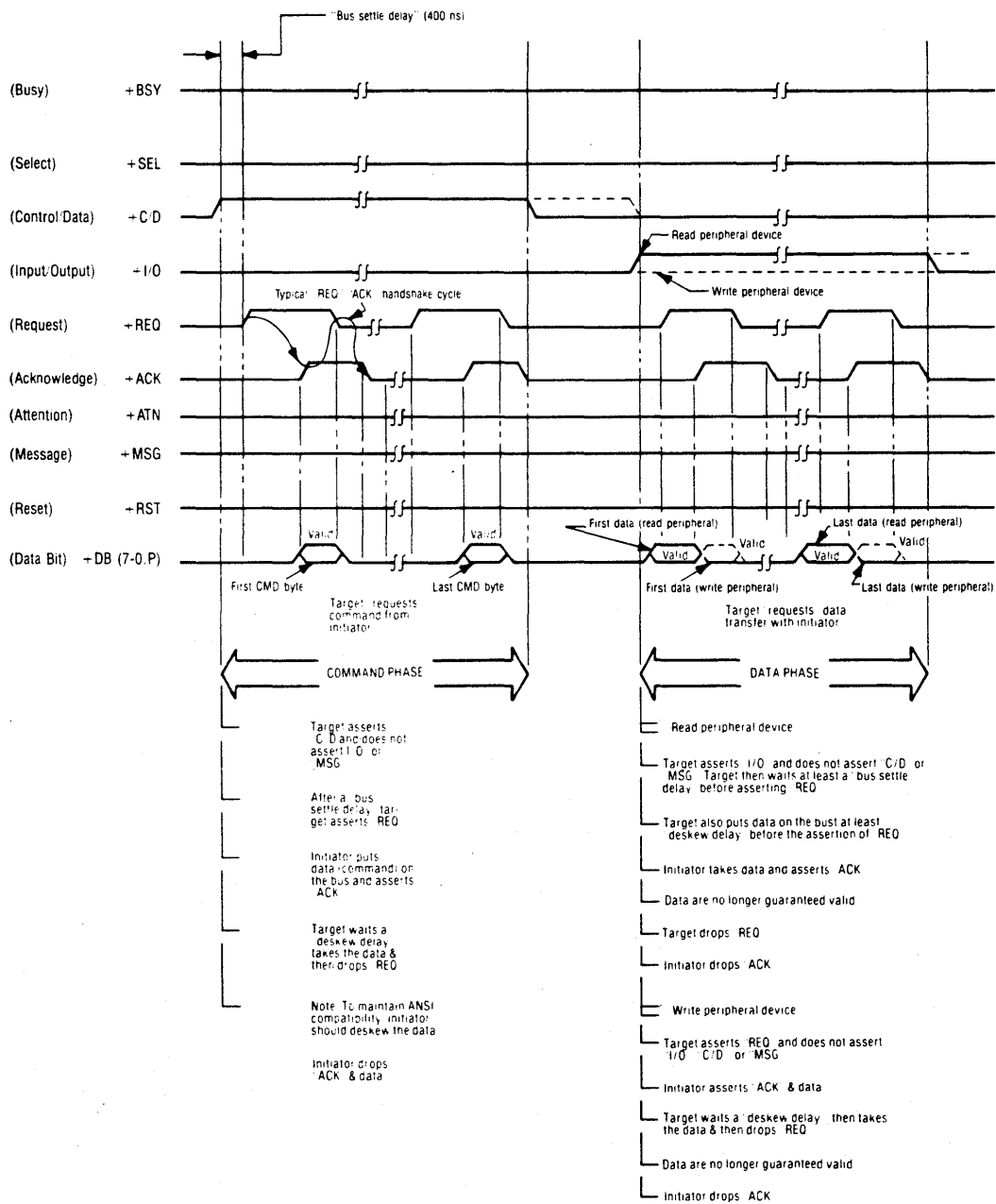
Figure 5-4. SCSI Bus Timing (con't)
