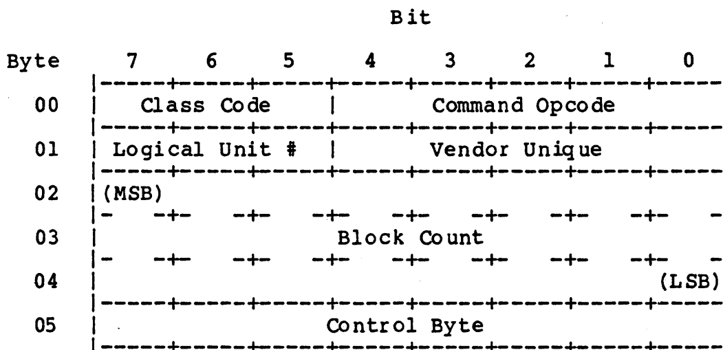
Figure 5-5. Class 0 CDB Supported by the ACB-3530
