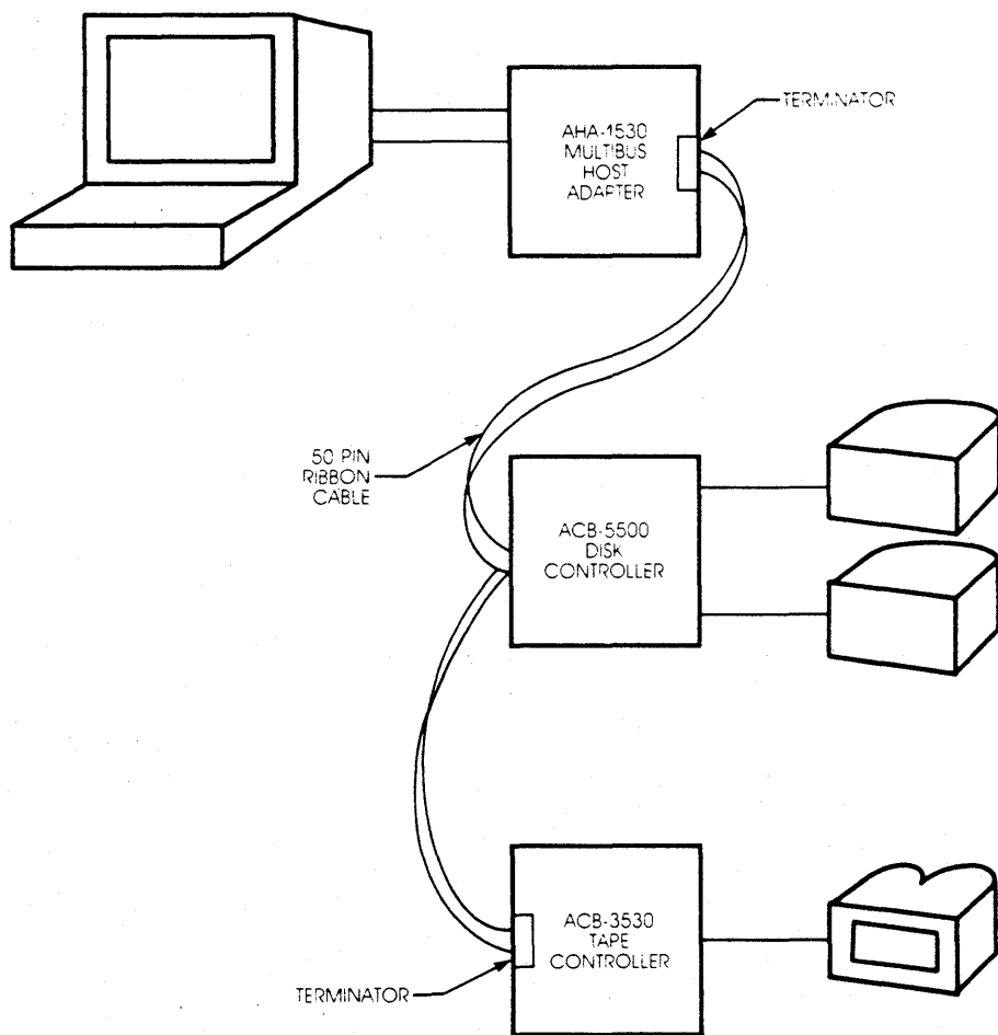
Figure 5-1. Typical SCSI Configuration
