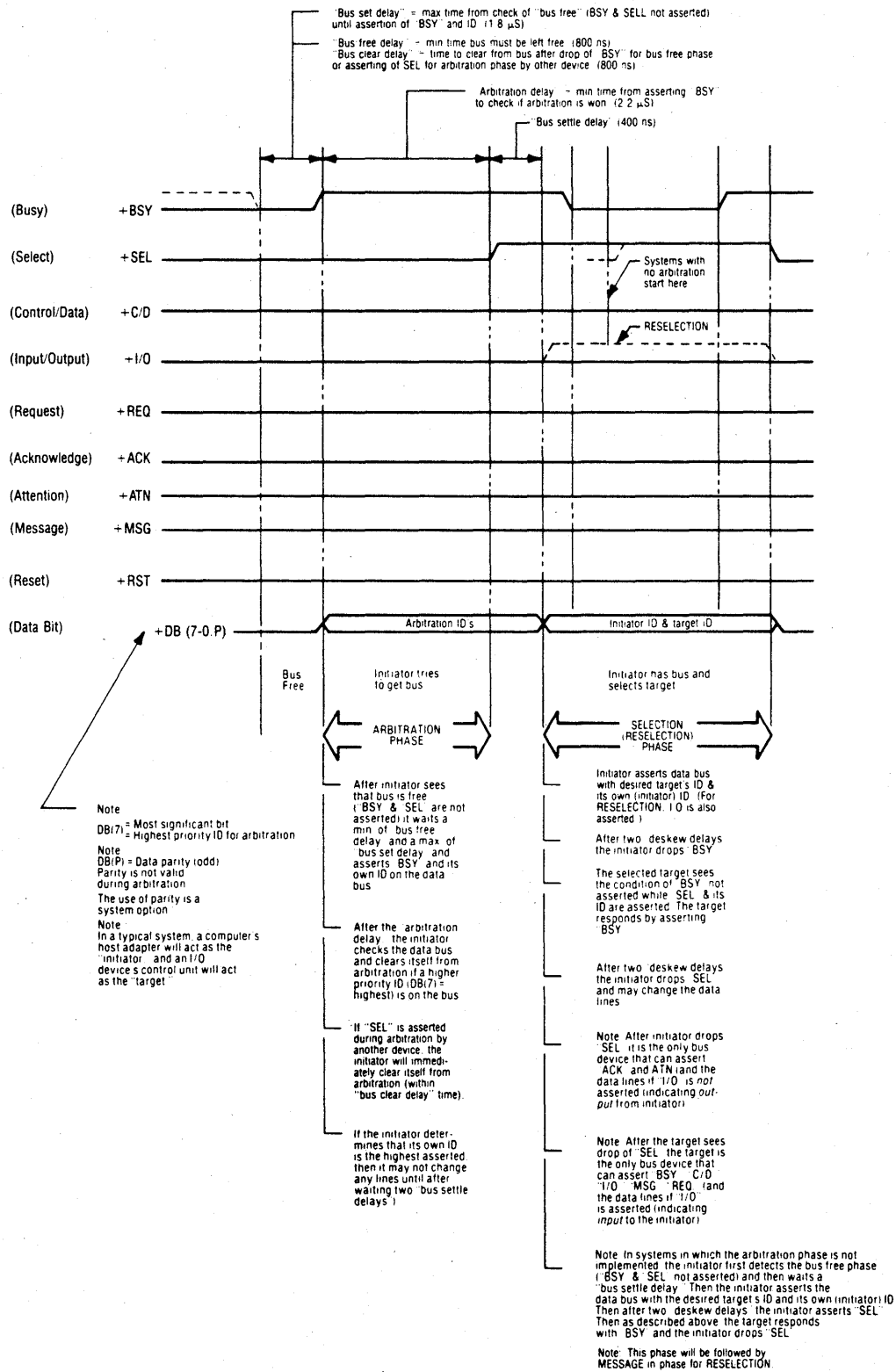
Figure 5-4. SCSI Bus Timing
