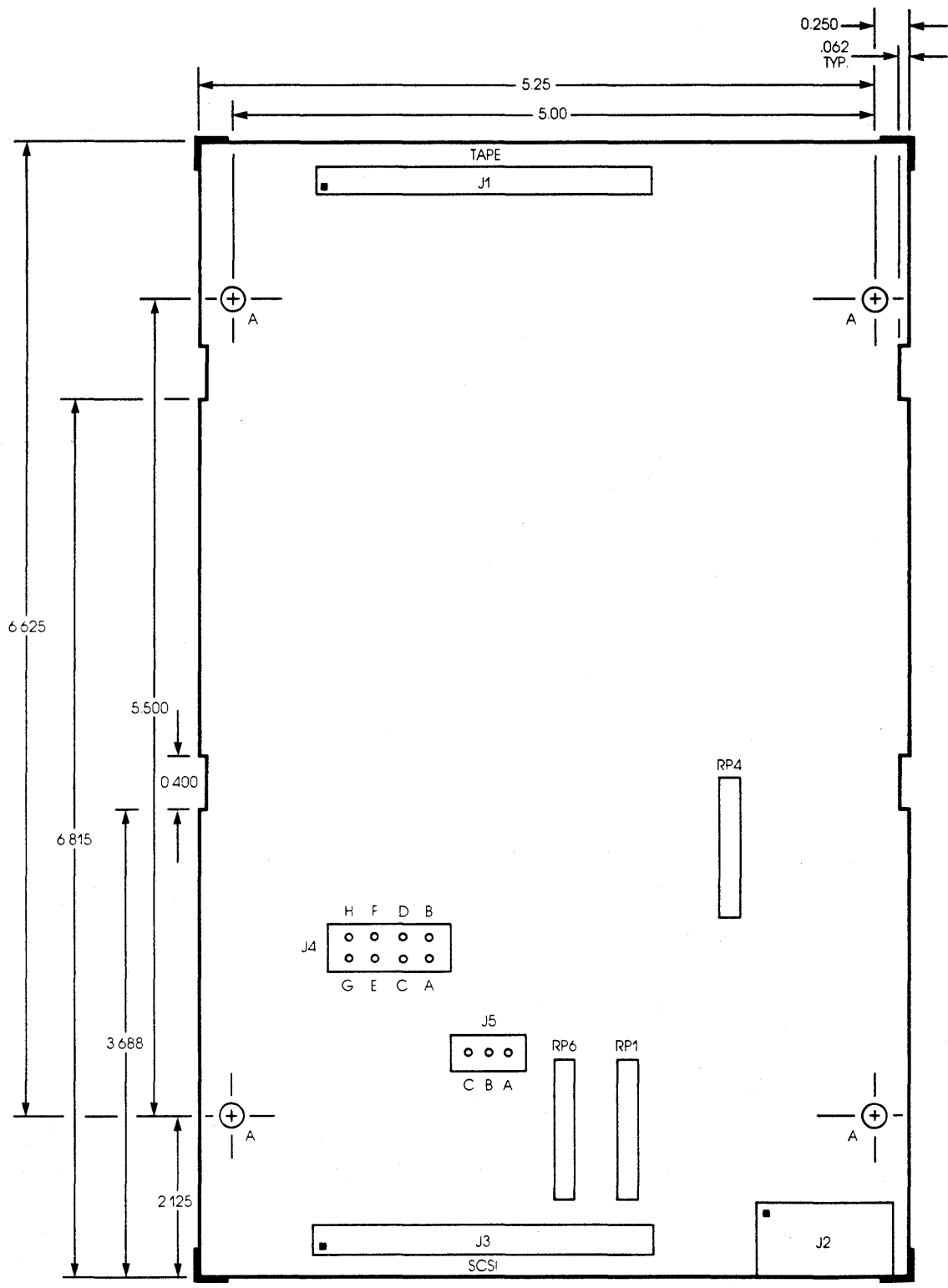
Figure 1-1. ACB-3530 Board Layout
