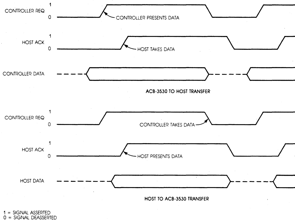
Figure 5-2. REQ/ACK Handshake
