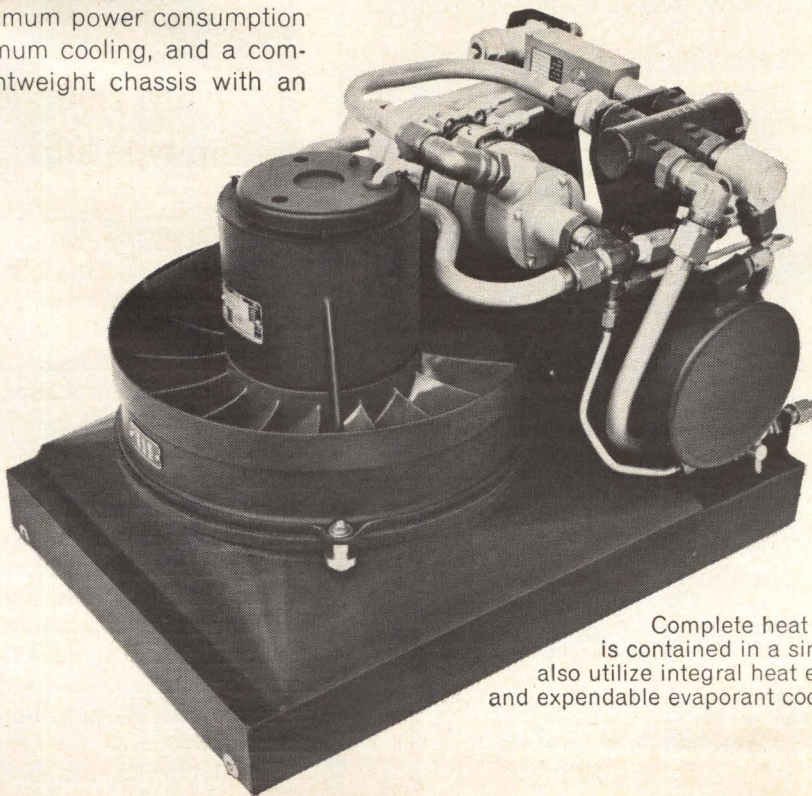
This AiResearch "ICE" system includes both the heat transport system and electronics enclosure with integrated heat exchanger.
