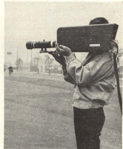
Single-tube color tv camera developed by Nippon Columbia Co. registers blue and red chrominance information as black-and-white stripes.
