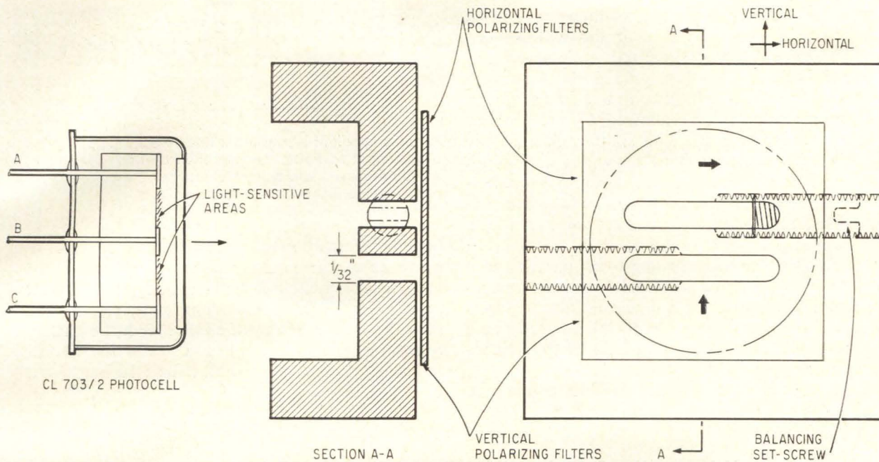
Slot dimensions in the aperture block narrow the angle of view to minimize the chance of noise accidentally triggering the device. Top and bottom slots are covered with horizontal and vertical polarizing filters respectively. The set screw compensates for imbalances in the photocell and the supply voltage circuitry by reducing the size of the light-sensitive area exposed.
