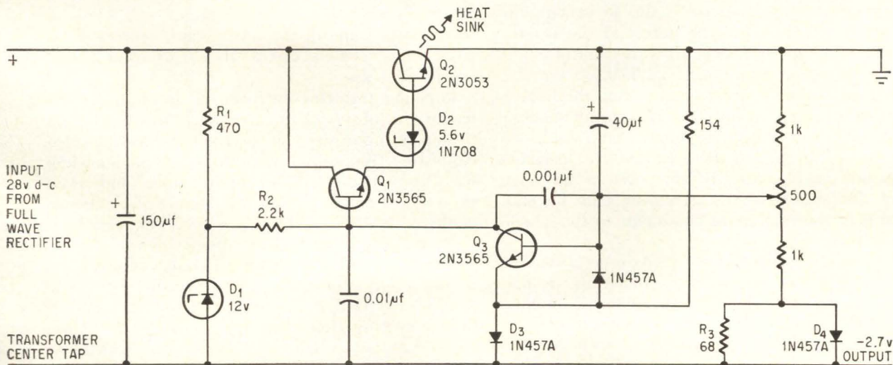
Zener diode D_2 provides amplifier Q_3 with the proper operating voltage. Reference voltage is established with a common diode, D_3 , instead of a zener diode since the zener would produce a larger voltage drop.
