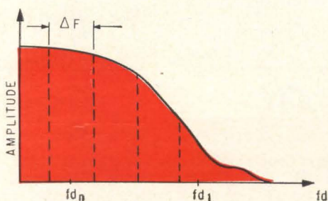
Terrain characteristics can be determined by the amplitude of backscattered radar signals measured within a fan-shaped beam of width \phi , since different types of terrain reflect different amounts of beam energy. Curves indicating the reflectance profile of the terrain below the spacecraft are obtained by plotting the amplitude of discrete frequencies in wideband doppler returns.
