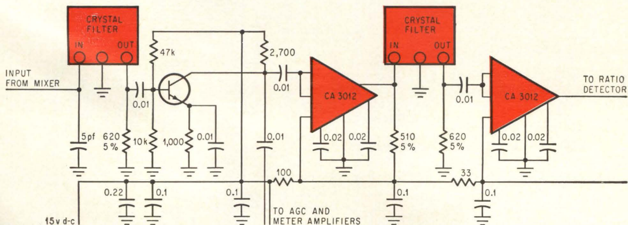
Quartz crystal filters are combined with high-gain IC amplifiers in the intermediate-frequency section of the f-m portion of Heath's a-m/f-m stereo receiver. Transistor stage following first filter is needed to drive automatic gain control and metering amplifiers. Gain of i-f stage is 120 db.
