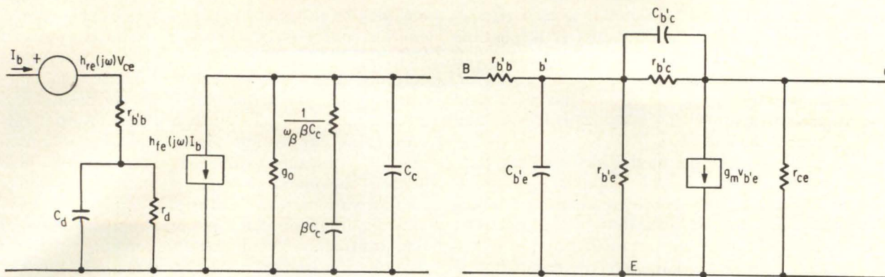
Although the circuit at the left is a good wideband h-parameter a-c model it suffers from one serious limitation—two of its parameters, h_{re} and h_{fe} , are frequency dependent. The limitation is overcome in the hybrid-pi circuit on the right.
