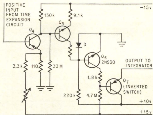
Q_4 — MULLARD LTD. TYPE BCY32 Q_7 — MULLARD LTD. TYPE OC202 Q_5 — MULLARD LTD. TYPE BCY43 D — MULLARD LTD. TYPE OA200
