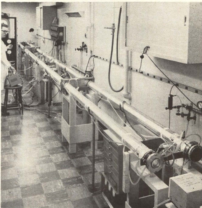
Dual-tube laser developed by Raytheon produces 1,200 watts, continuous-wave. By optically "folding" the tube, the laser's length is effectively doubled.
