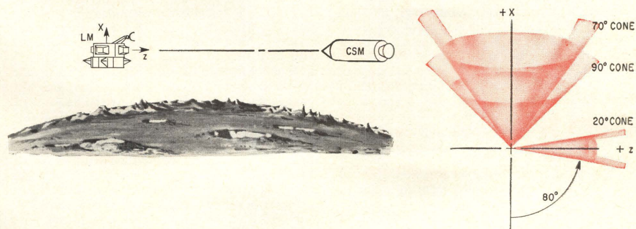
Lunar Module's antenna swings as it guides the capsule. During the landing phase shown in the upper drawing, the antenna ranges on the moon's surface. After the mission has been completed and the LM prepares to rejoin the Command and Service Module, the antenna swings upward and tracks the CSM across the sky. At rendezvous, the antenna will point along the spacecraft's "Z" axis.
