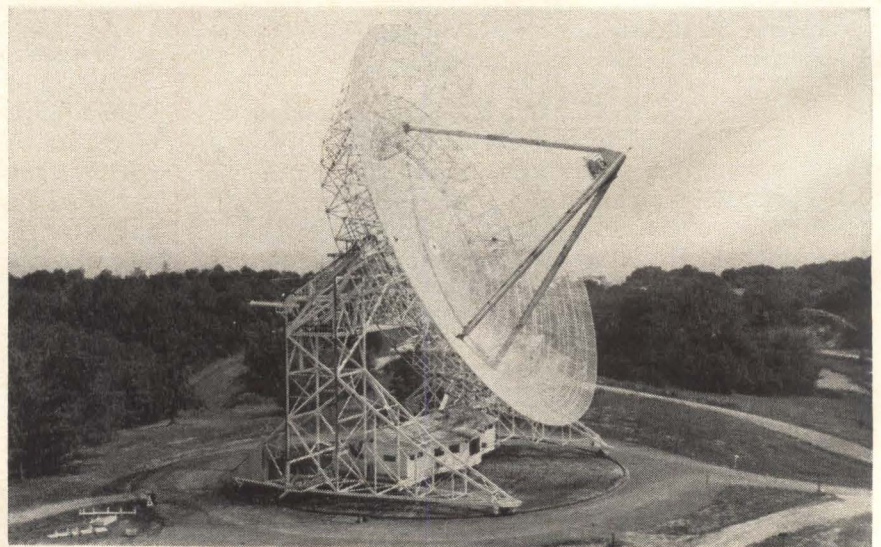
The Navy's giant antenna in Randle Cliff, Md., serves a dual purpose: it's used in antiballistic-missile work and to chart ionospheric conditions that would affect vhf signals in space-ground communications.
