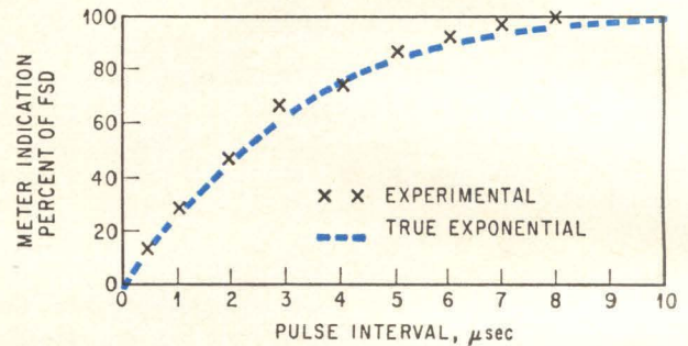
Time-voltage transfer curves for several ranges of the chronometer. Restricting the chronometer's operation to a portion of its complete range keeps the readout linear. The readout can also be made exponential if desired. The curve directly above shows an exponential characteristic compared with a true exponential curve.
