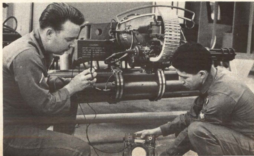
Launcher portion of minigun-rocket system used on UH-1B helicopters is inspected by instructors at Aircraft Repairman's school.
