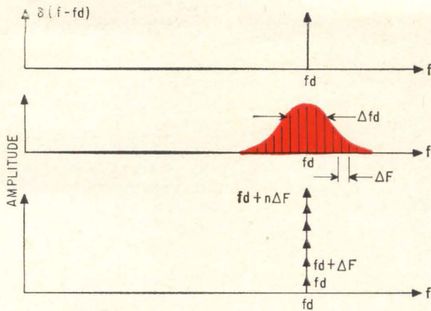
Doppler bandwidth of a pencil radar beam is very narrow (top), while a broad beam produces a Gaussian distribution of the returning doppler signals (center). Spectrum compression allows frequencies within the doppler spectrum to be superimposed to approximate the impulse function shown in the lower diagram.
