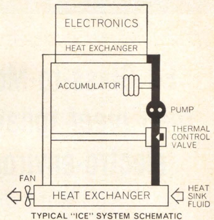
This AiResearch "ICE" system includes both the heat transport system and electronics enclosure with integrated heat exchanger.
