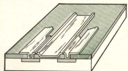
STEP 11. Fourth mask metallization pattern etched
