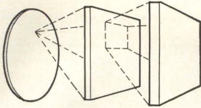
STEP 1. Wafer, MOS IC, and individual MOS FET
