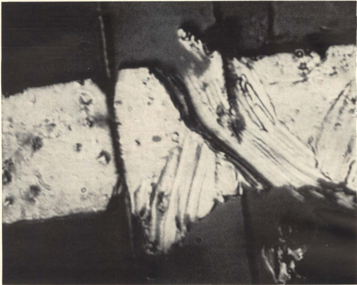
Scratched aluminum intraconnection can lead to an open circuit. The thinner conducting area has a reduced current capacity and therefore may burn through during operation.
