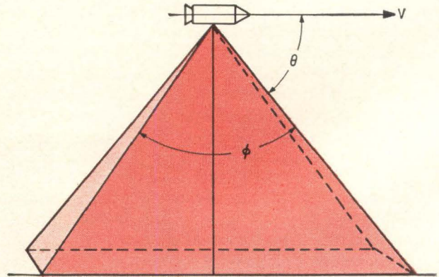
Terrain characteristics can be determined by the amplitude of backscattered radar signals measured within a fan-shaped beam of width \phi , since different types of terrain reflect different amounts of beam energy. Curves indicating the reflectance profile of the terrain below the spacecraft are obtained by plotting the amplitude of discrete frequencies in wideband doppler returns.
