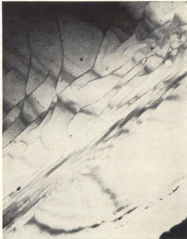
Dislocation structure , discontinuities on surface, are shown magnified with an electron microscope. The dislocation is at the surface of a power transistor near the junction region. Such a fault could lead to a soft junction and to abnormal electrical properties in the IC.
