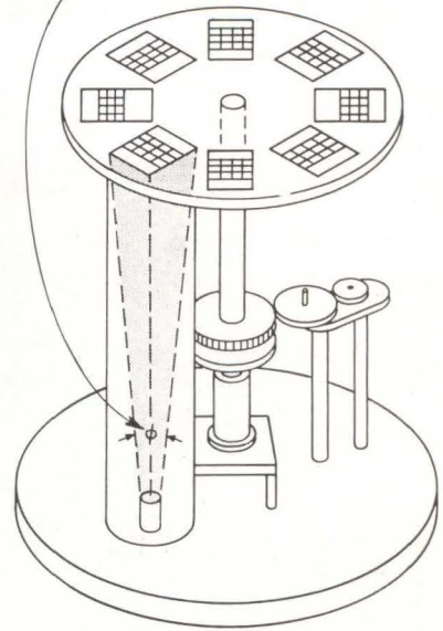
SEQUENTIAL process equipment (left) (vacuum chamber removed) deposits films on successive substrates with separate firings of source material. Diagram (right) shows how substrates are located far enough away from source material to subtend small area of minimum vaporization angle thus getting high depositional accuracy—Fig. 2
