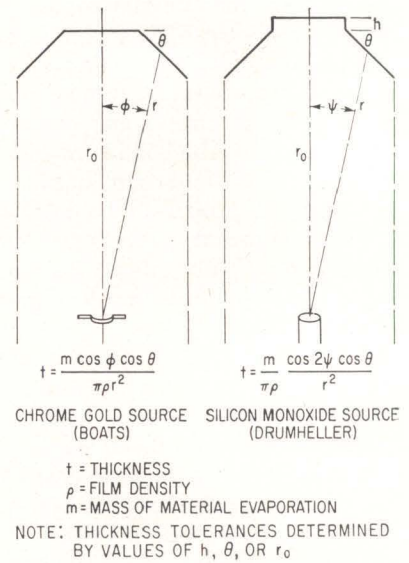
ONE-SHOT process equipment (left), shown with vacuum chamber removed, deposits films on several substrates with one firing of source material. Diagram (center) shows details of substrate holder and general location with respect to source material. Geometric diagrams (right) are used to accurately position holder with respect to source material in accordance to material used; note also modifications in shape of holder's support frame to accommodate silicon monoxide deposition—Fig. 1
