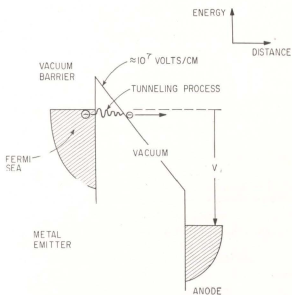
SIMPLIFIED REPRESENTATION OF THE FIELD EMISSION PROCESS
