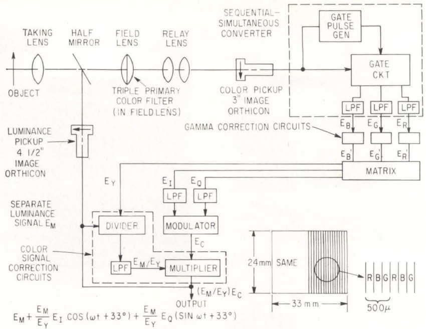
(A) IMAGE IS SPLIT for luminance and color pickup. NTSC color signals are generated by combination of color filter, image orthicon and gating circuit (A). Filter consists of alternating red, blue and green color stripes (B)
