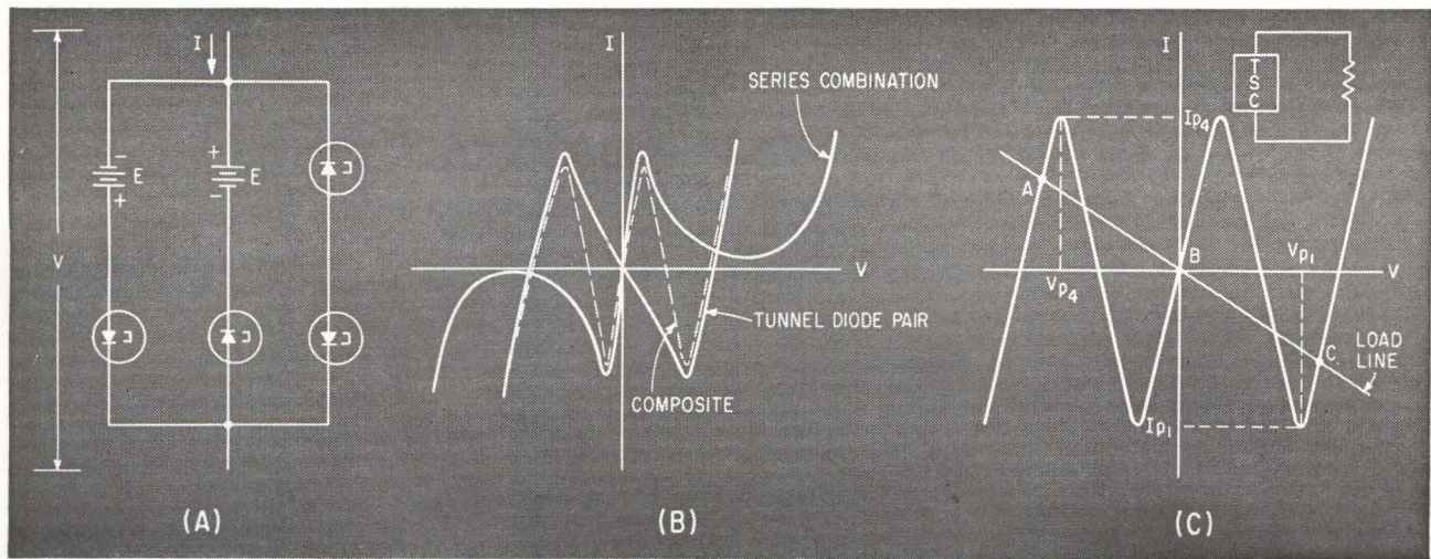
TRISTABLE circuit (A) produces the composite curve (B) with operation explained by (C)—Fig. 2
