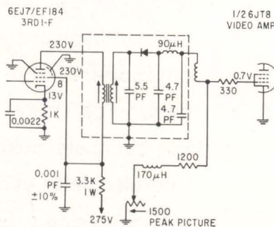
PEAK PICTURE control circuit used by Zenith to improve pictures
