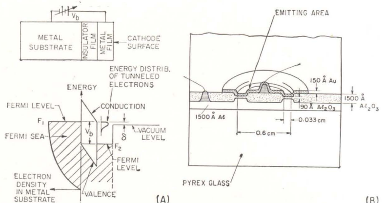
ENERGY relations (A) and one type of construction (B) for tunnel cathodes—Fig. 6
