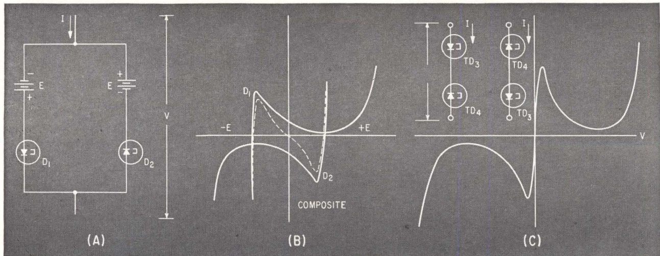
TUNNEL DIODE pair (A) produces the composite volt-ampere curve of (B). A series diode combination produces the curve of (C)—Fig. 1
