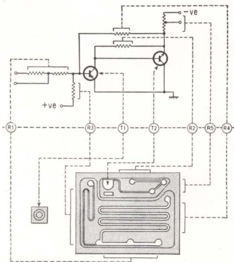
INTEGRATED silicon microcircuit by Ferranti Ltd. is constructed from two silicon chips and contains two transistors and six resistors. Photo of circuit at right shows mounting in a reduced height JEDEC TO-5 case
