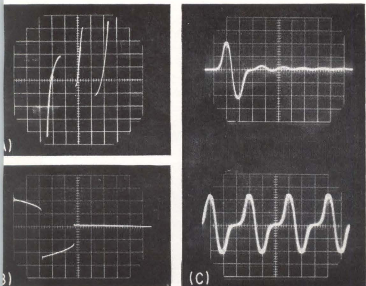
TRISTABLE volt-ampere characteristics (A), bipolar voltage pulse (B) and bipolar voltages with high-speed pulses shown at (C) Fig. 4
