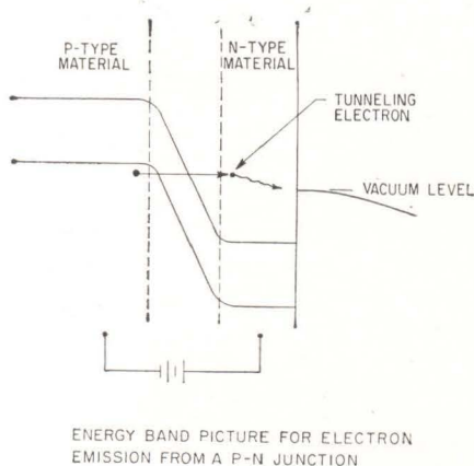
P-N JUNCTION cathode must overcome severe problems to become practical—Fig. 5
