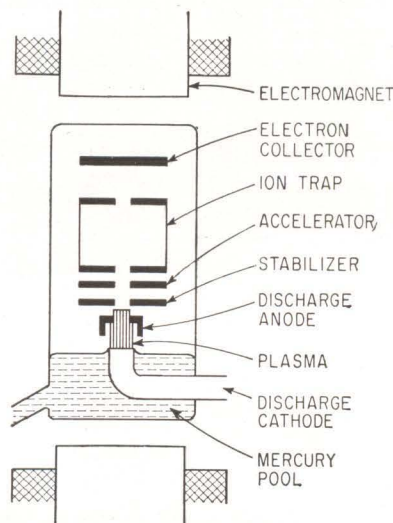
PLASMA cathodes, as suggested by K. G. Hernquist—Fig. 3
