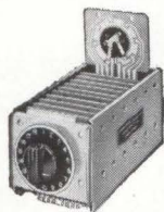
3" x 2 1/2" Rotary Selector Switch, Series RS30. Manually (illustrated), solenoid or motor operated.
