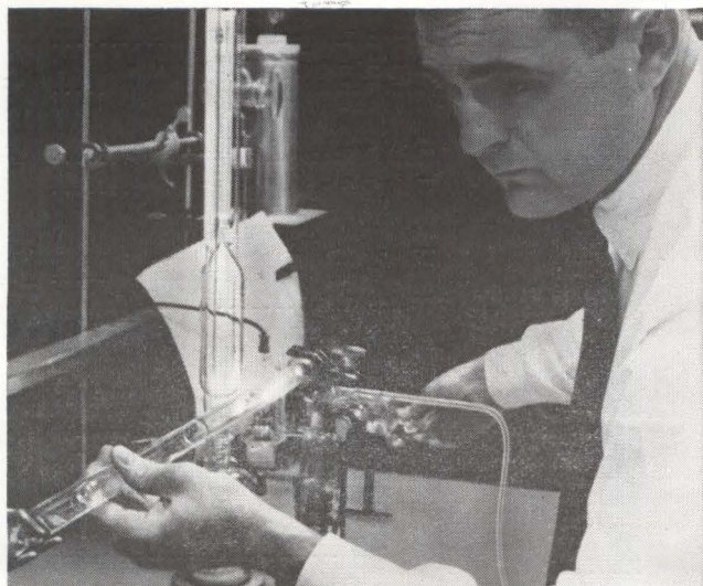
In this method of preparing ultrapure gallium arsenide, gallium reacts with arsenic in a quartz tube with oxygen added under pressure to suppress dissociation of \text{SiO}_2 .
