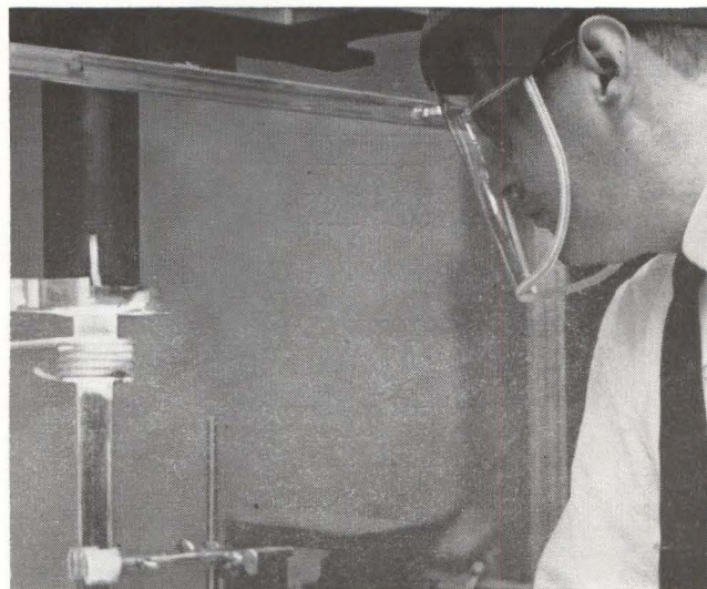
In this alternative method, gallium arsenide crystals are pulled from gallium and arsenic melted in aluminum nitride crucibles, which do not liberate silicon contaminants.
