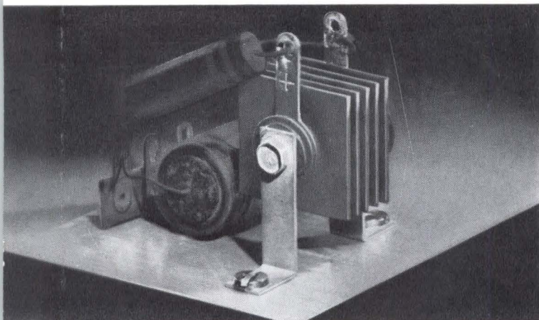
Space-consuming plate-type rectifiers take valuable chassis area, require additional space for adequate isolation and mounting hardware.
