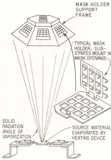
ONE-SHOT process equipment (left), shown with vacuum chamber removed, deposits films on several substrates with one firing of source material. Diagram (center) shows details of substrate holder and general location with respect to source material. Geometric diagrams (right) are used to accurately position holder with respect to source material in accordance to material used; note also modifications in shape of holder's support frame to accommodate silicon monoxide deposition—Fig. 1
