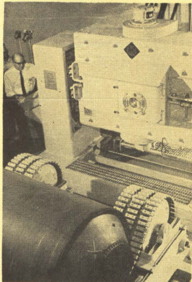
BETATRON automated x-ray system made for Redstone Arsenal by Allis-Chalmers indicates flaws on roll-chart recording instead of film. Photosensitive system detects flaws in rocket (foreground) as difference in light output of sodium-iodide crystals
