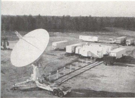
AIR-TRANSPORTABLE ground terminals may be similar to this 30-ft dish, 11-vehicle system built by Bendix for Syncom
