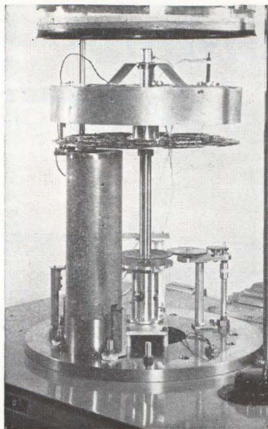
SEQUENTIAL process equipment (left) (vacuum chamber removed) deposits films on successive substrates with separate firings of source material. Diagram (right) shows how substrates are located far enough away from source material to subtend small area of minimum vaporization angle thus getting high depositional accuracy—Fig. 2
