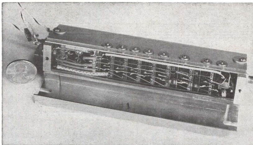
COMPLETE log i-f amplifier showing module construction and relative size compared with a penny
