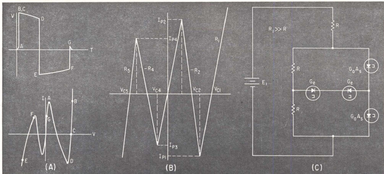
BIPOLAR voltage pulse with tristable composite curve (A). Linear equivalent model is shown at (B) and a practical circuit at (C)—Fig. 3
