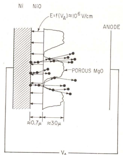
ELECTRONS are multiplied in MgO layer and some escape—Fig. 4
