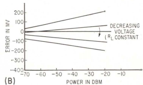
TEMPERATURE COMPENSATION of the load resistor decreases error at the high power levels (A); further improvement may be had by using a temperature compensated -6 volt supply (B)—Fig. 7
