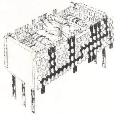
TYPICAL ministac circuit with wiring on side mountings; dark side-sections are wiring punched from standard material
