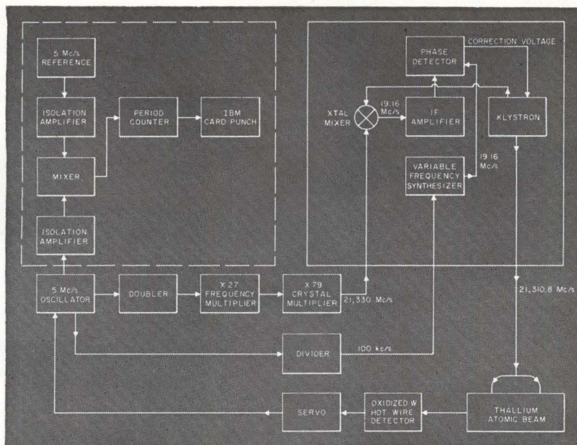
THALLIUM MEASUREMENT SYSTEM at National Bureau of Standards has phase-locked klystron loop to excite resonance
