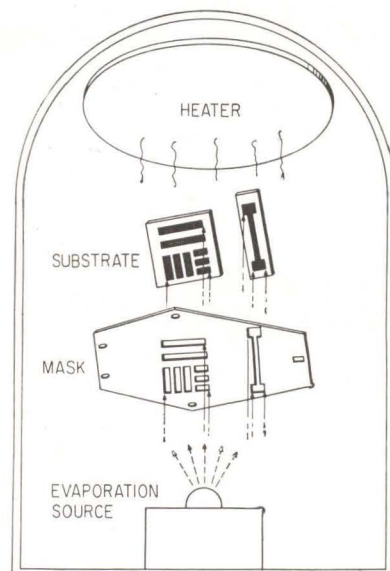
FABRICATION of thin-film circuits is performed using a vacuum evaporation system—Fig. 3
