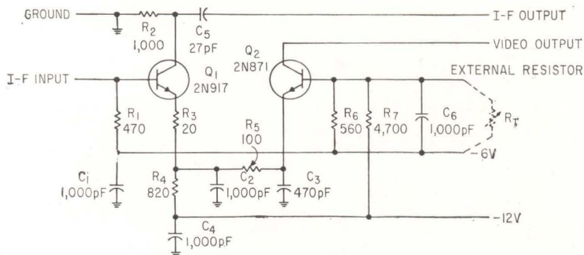
SINGLE log i-f module—Fig. 1
