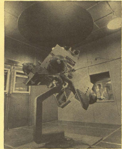
SATELLITE simulator at Westinghouse Air Arm simulates movements of orbiting satellite. It's balanced on 12-inch, air-floated ball bearing. Attitude is changed by small air jets, warm aluminum dish overhead simulates earth
