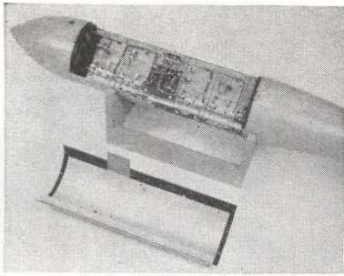
CASING is removed to show four transmitter sections. Each section transmits for 1/5 second each second on its own frequency
