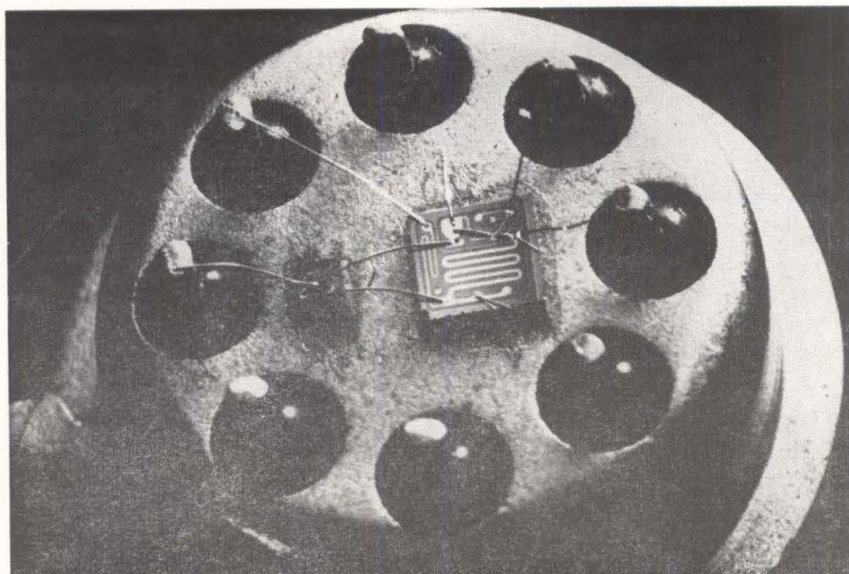
INTEGRATED silicon microcircuit by Ferranti Ltd. is constructed from two silicon chips and contains two transistors and six resistors. Photo of circuit at right shows mounting in a reduced height JEDEC TO-5 case
