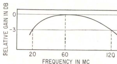
GAIN characteristic of a single log i-f stage—Fig. 2
