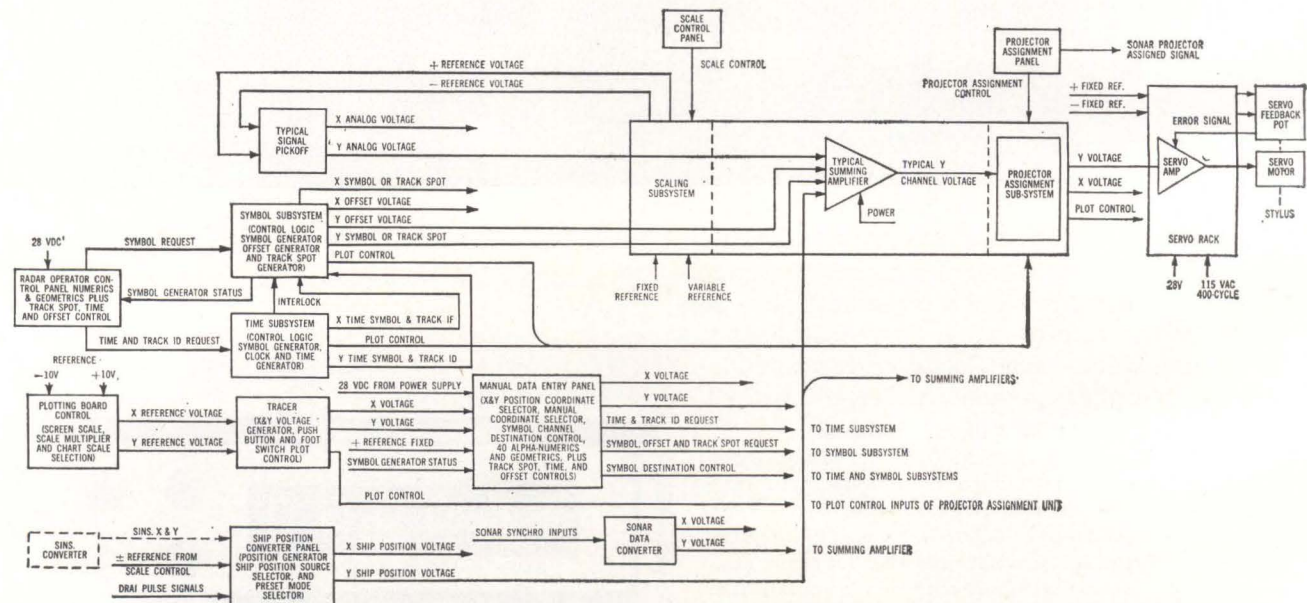
COMPLETE OPERATIONAL ORGANIZATION of the Tactical Navigational Display System. All inputs, plus a typical plotting channel are shown
