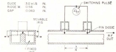
SOLID-STATE switched protector is designed to protect varactors in parametric receivers
