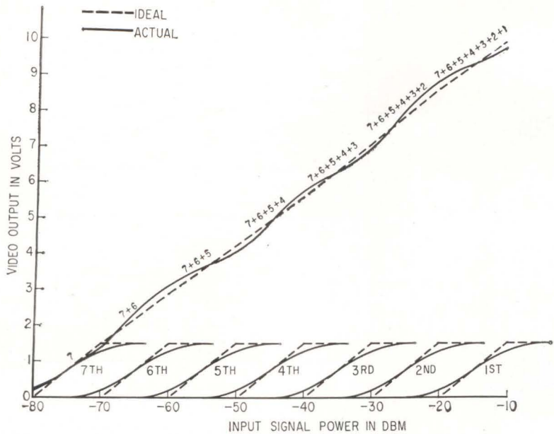
OVERALL PERFORMANCE characteristics of the complete seven-stage amplifier—Fig. 6
