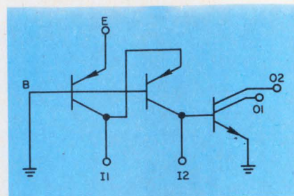
Current-hogging injection-logic NAND gate (left) is 20% smaller than equivalent I 2 L cells. Schematic of cell (right) shows CHL gate with a functionally integrated output transistor.
