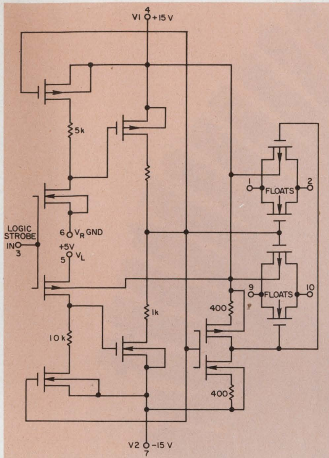
7. A typical driver gate using floating body, Intersil's IH5042, employs standard 0-to-3-V TTL levels to change the switch state.
