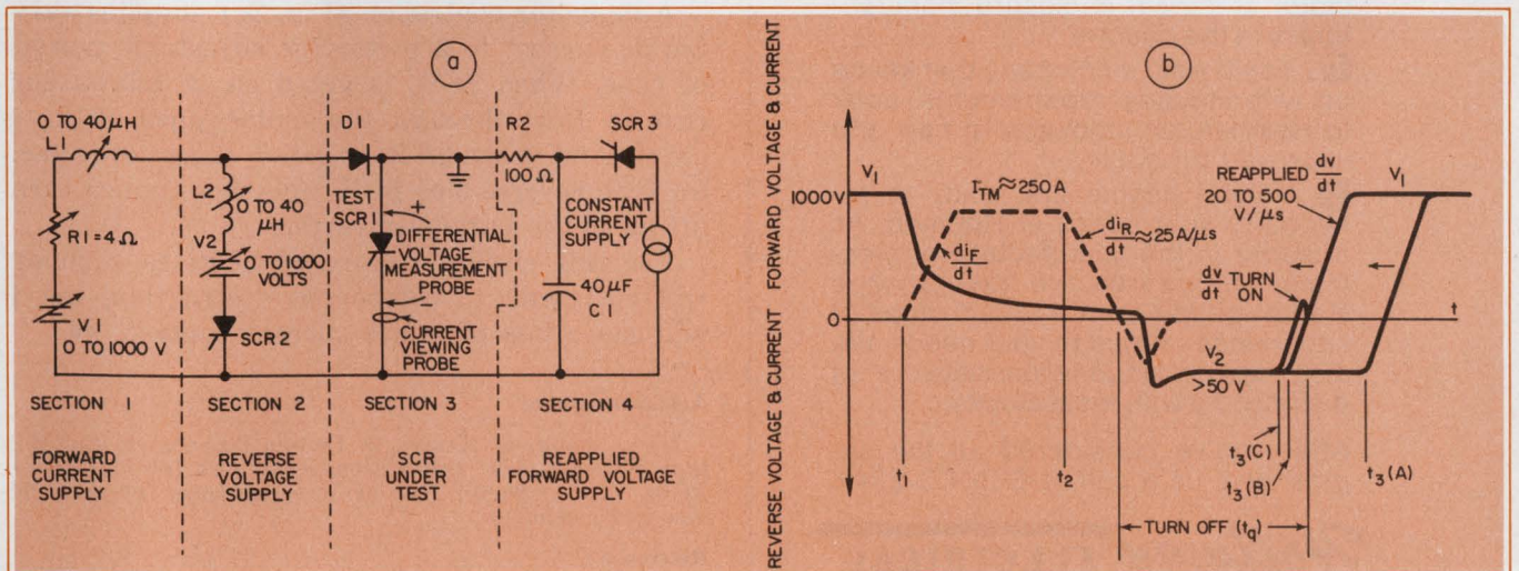
2. Simplified version of a typical SCR test circuit (a) can test for turn-off time as well as many other parameters.
