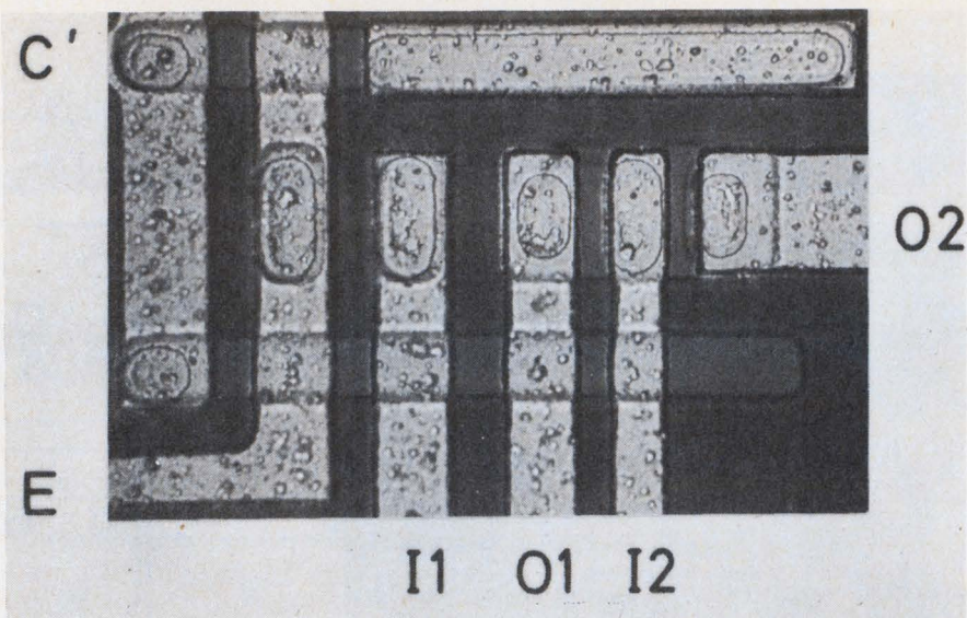
Current-hogging injection-logic NAND gate (left) is 20% smaller than equivalent I 2 L cells. Schematic of cell (right) shows CHL gate with a functionally integrated output transistor.
