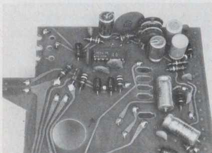
One mass-produced PLL IC is the FM stereo demultiplexer, shown here on a Delco FM auto radio PC board. This IC has a 76-kHz VCO, which is divided into 38-kHz segments for demodulating stereo information.
