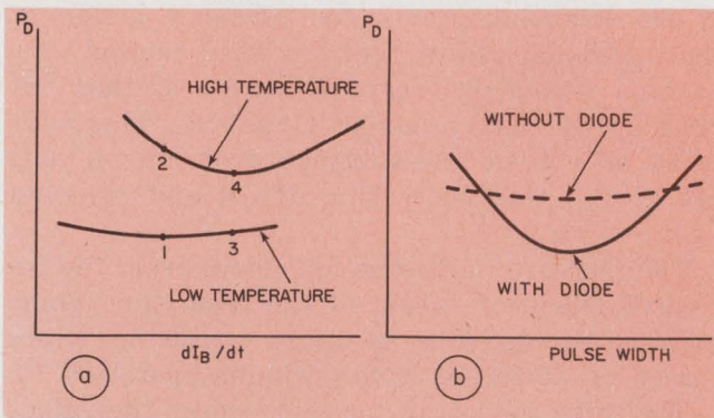
4. Power-dissipation curves of the output transistors are useful in determining safe operating levels for the circuit. Worst-case calculations provide the best guidelines for reliability and stress.
