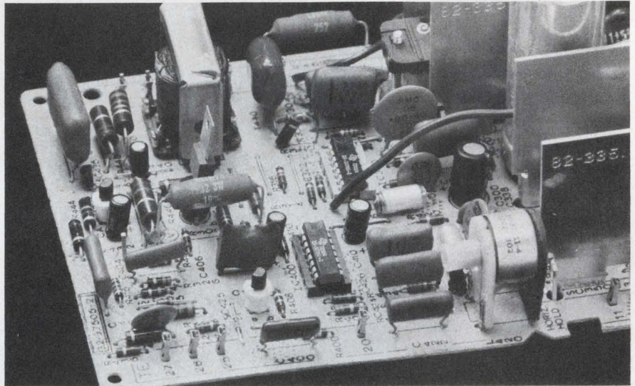
The horizontal oscillator and phase detector of this Sylvania TV-set PLL used for horizontal hold are in the IC (center, front). The oscillator tuning coil shown at the right stabilizes the oscillator frequency.
