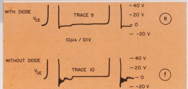
2. Typical horizontal output traces, taken at various points in the test circuit, are used as a reference for circuit modifications to optimize performance.
