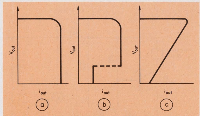
4. Various methods of overload protection can be used. They include current limiting (a), short-circuit shutdown (b) and current foldback (c).
