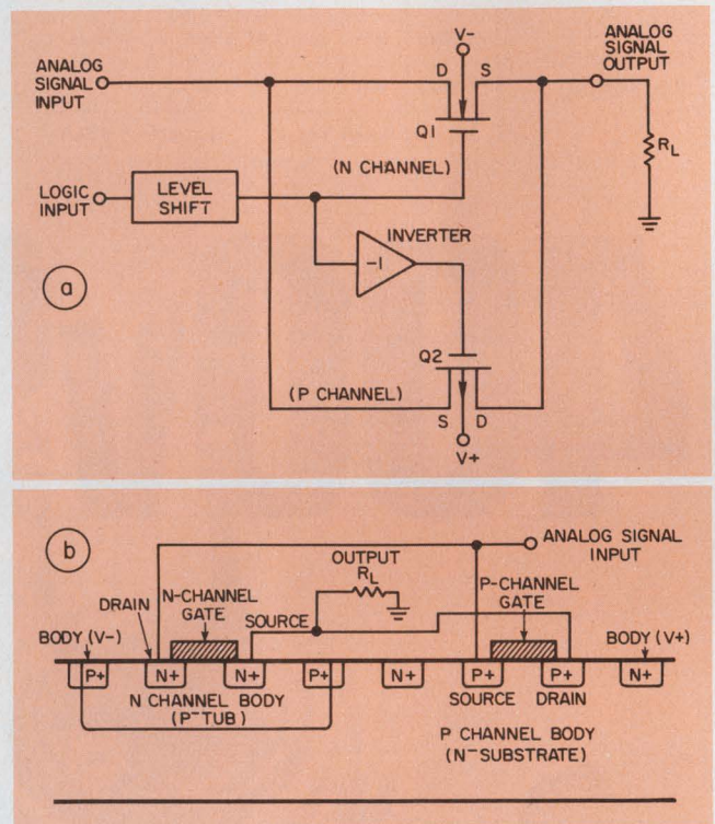
1. A typical CMOS analog switch employs an n and p-channel MOSFET in parallel (a). The gate's cross-section (b) contains three parasitic transistors that are inherent in conventional CMOS processing.
