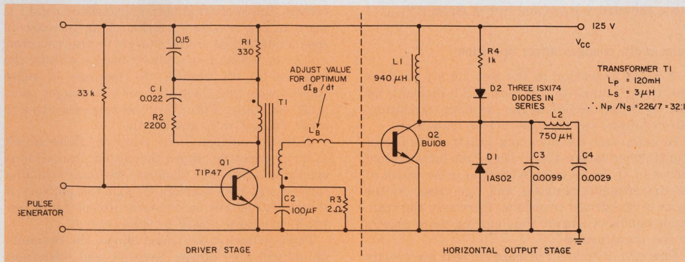
1. A test circuit can simulate the horizontal output stage of most CRT display systems. This can help evaluate the
