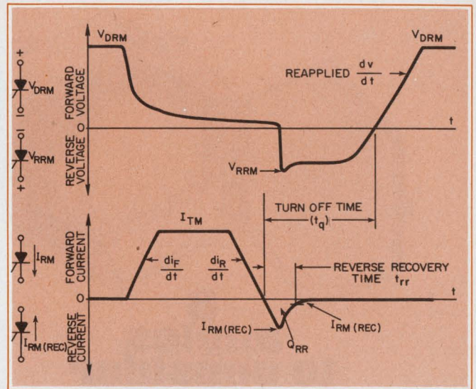
1. Voltage and current waveforms for an SCR start changing as soon as a gate signal is applied to the device. When the current waveform passes through zero, it starts the turn-off time period of the SCR.
