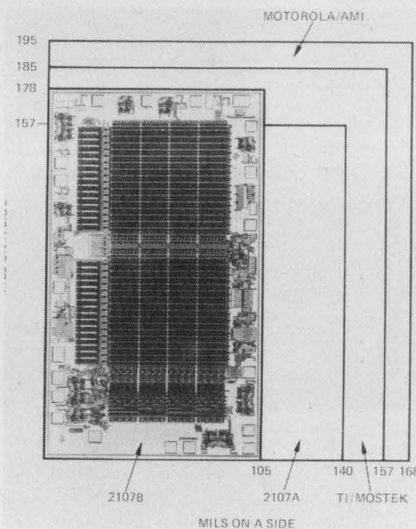
One of the smallest 4-k RAM chips is Intel's 2107B. The memory has 200-ns access.
