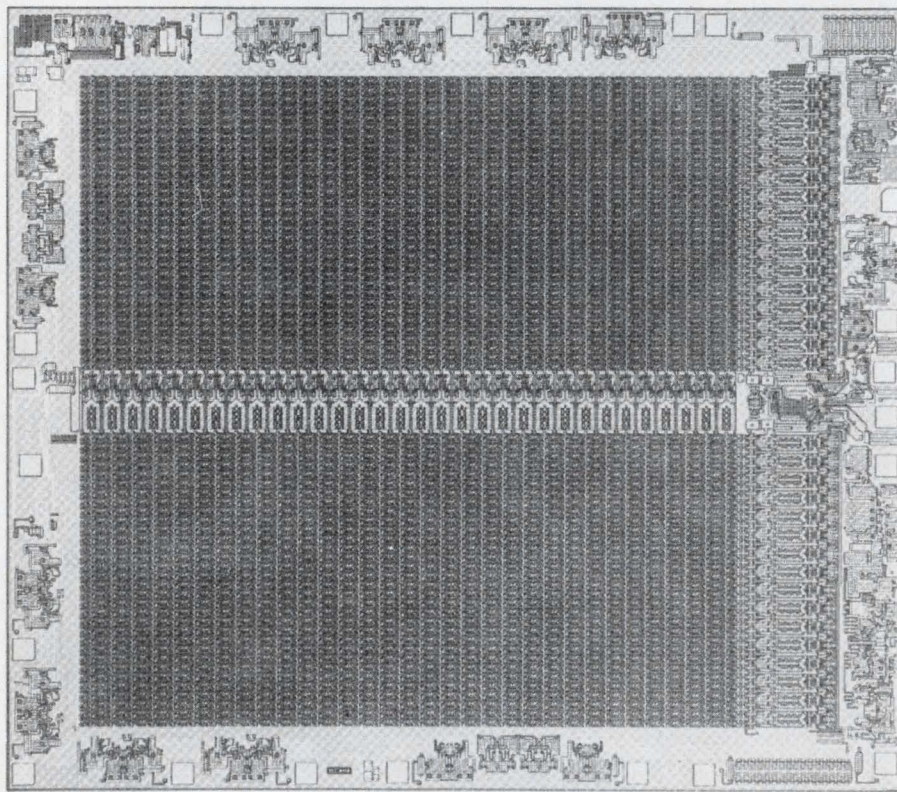
Aiming for ECL-oriented systems, Intel's latest 4096-bit MOS RAM has access time of less than 80 ns. The ECL-compatible chip employs charge-pump techniques to obtain operational features of static units.
