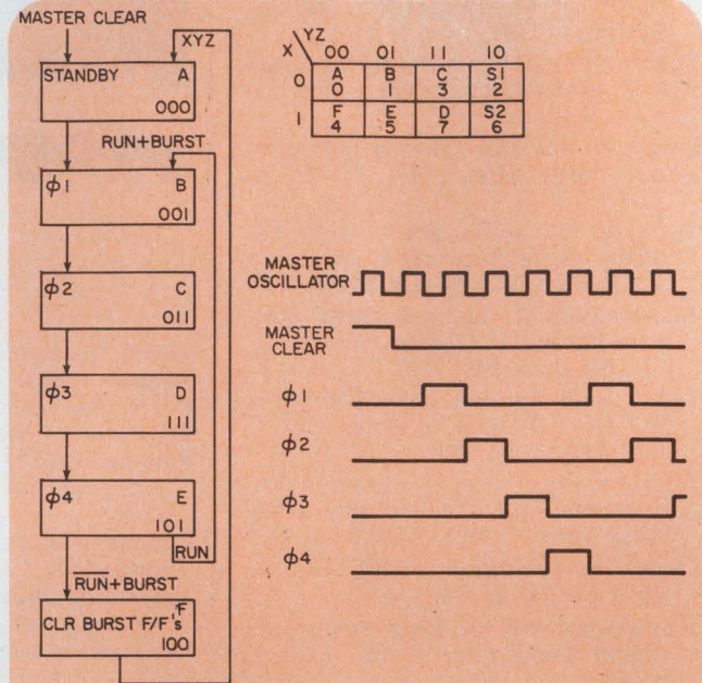
1. A timing diagram, state chart and Karnaugh map for a four-phase clock system illustrate a technique for designing a self-clearing mutiphase clock with an even number of phases.
