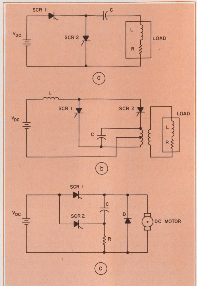
3. Some typical turn-off circuits for a series inverter (a), a parallel inverter (b) and a dc motor controller (c) don't require much additional circuitry.
