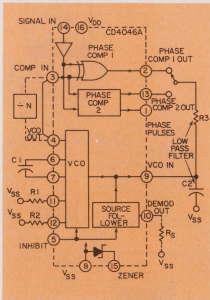
3. Micropower CMOS PLLs, like this RCA CD4046, draw but 75 \mu W. They are general purpose circuits.
