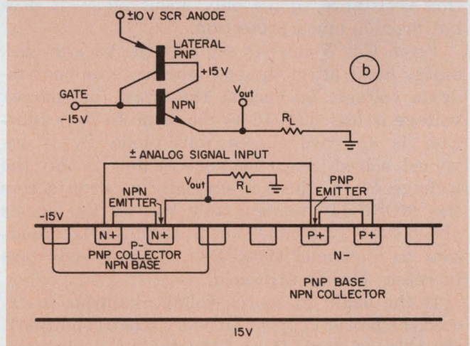
3. No SCR action can occur as long as the \pm 15 -V supplies are turned on. However, under normal operating conditions, such as the switching of analog signals (a), the circuit can latch up (b). A sufficiently high load resistance, R_L , can avoid destructively high currents.
