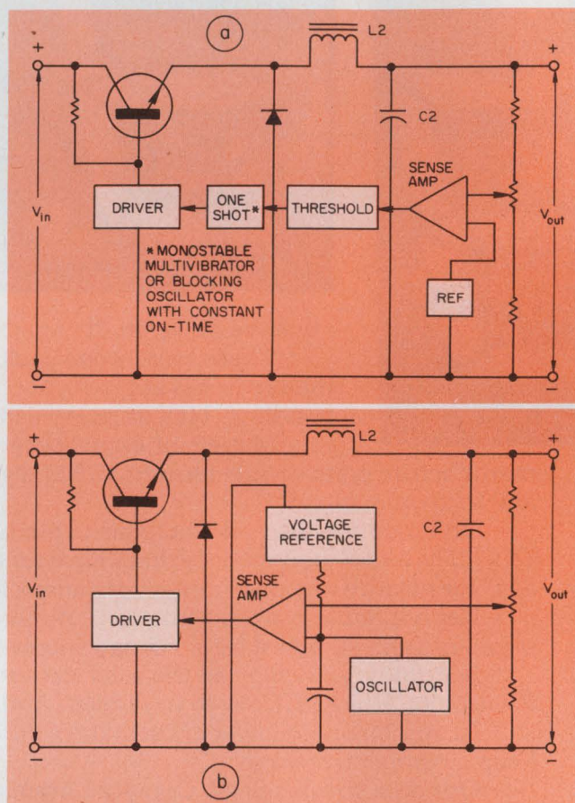
1. Switching regulators can be of the free-running type—in which the transistor operates at constant pulse width and variable frequency (a)—or of the fixed-frequency type, in which the transistor ON time varies (b). Efficiencies exceed those of conventional linear regulators.
