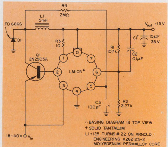
3. An IC regulator can be used as the basis for a switching design. Transistor Q_1 is added to increase the current-handling capability.
