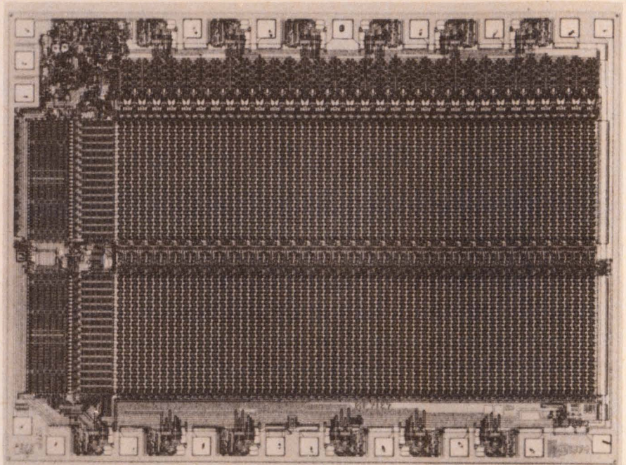
Avoidance of dummy cells simplifies circuit tolerances and reduces on-chip circuitry in Microsystems' 2107C, the company's latest 4-k RAM.
