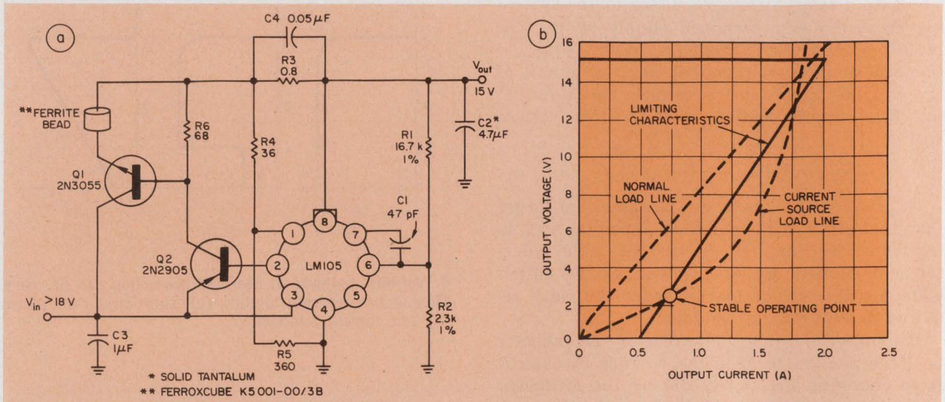
6. Foldback limiting is perhaps the best choice for over-load protection (a), but as shown in the limiting char-
