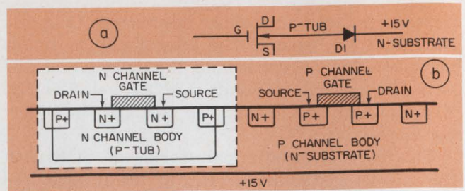
4. The floating-body technique eliminates the parasitic SCR. The technique uses back-to-back diodes that electrically float the body. The diode in series with the n-channel MOSFET body results automatically by use of the p-tub-to-substrate junction (b).
