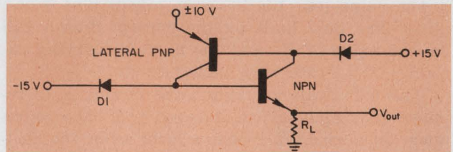
6. The diodes introduced by the floating-body technique allow either the positive or negative 15-V supply to be turned off without latch up.
