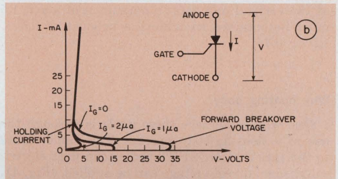
2. A parasitic SCR results from the combination of vertical and horizontal npn transistors with a lateral pnp (a). Either the base of the npn or pnp can trigger the dual-gate SCR and the parasitic device has the characteristic curve shown in "b."
