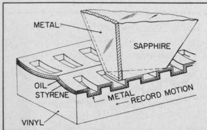
Capacitance pickup detects variations in the width and separation of slots in record groove that contains recorded information.
