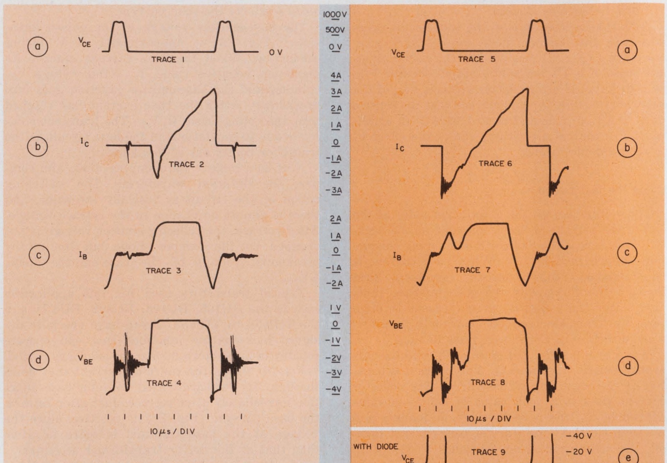
2. Typical horizontal output traces, taken at various points in the test circuit, are used as a reference for circuit modifications to optimize performance.
