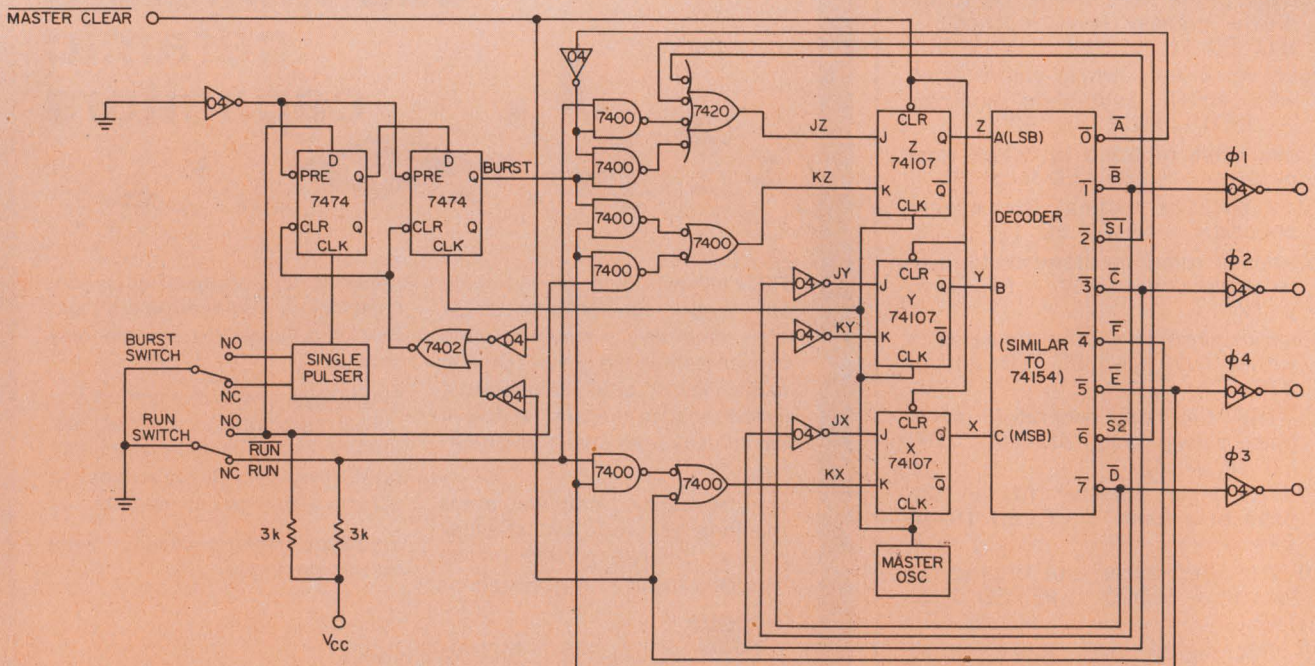
2. A multiphase clock should automatically resume its normal sequence even if temporarily thrown off
