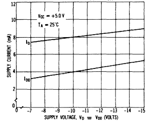
FIG. 7: SUPPLY CURRENT ( I_O and I_{DD} ) VS SUPPLY VOLTAGE ( V_O and V_{DD} )
