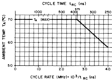
Fig. 1 Maximum ambient temperature versus cycle rate for extended frequency operation. T_A (max) for operation at cycling rates greater than 2.66 MHz ( t_{CYC} < 375\text{ns} ) is determined by T_A (max) ^{\circ}\text{C} = 70 - 9.0 \times (\text{cycle rate MHz} - 2.66) for -3.
