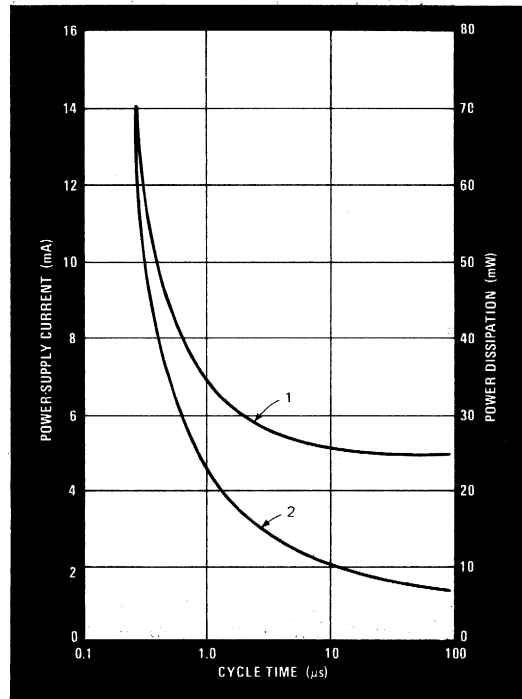
The 4104 is the only static RAM with frequency-dependent power dissipation, resulting from the use of dynamic interface circuits. Clock-on time (low-level) for curve 1 is 100 ns; clock-off time (high-level) for curve 2 is 200 ns. For both curves, ambient temperature is 25 C and power-supply voltage is 5 V.
