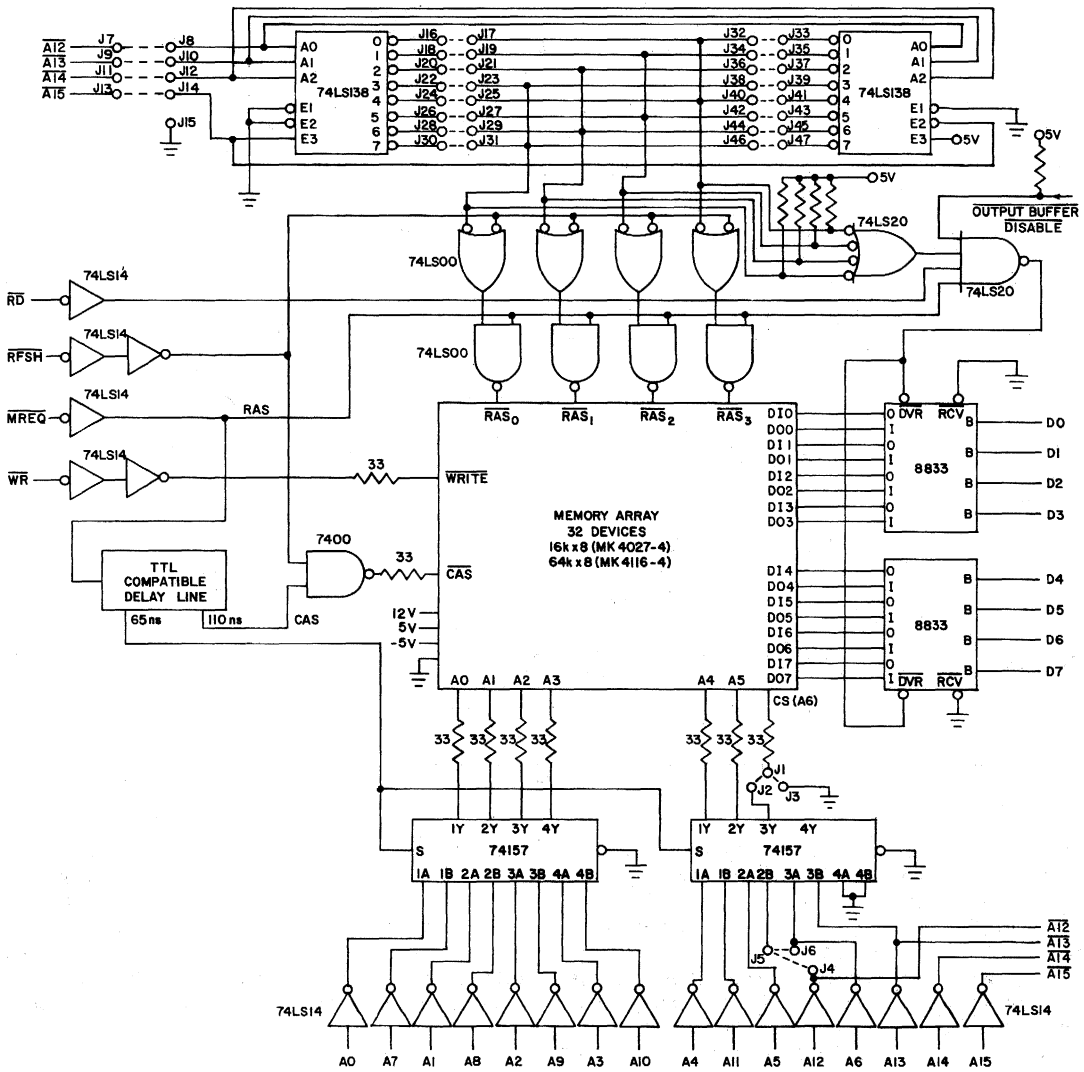
DESIGN EXAMPLE NO. 2 SCHEMATIC DIAGRAM Figure 8.
