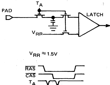
Figure 5: ADDRESS AND DATA INPUTS
