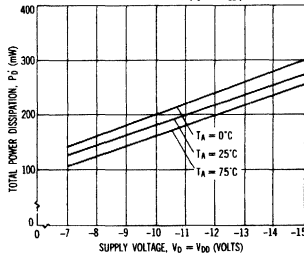
FIG. 3: TOTAL POWER DISSIPATION ( P_D ) VS SUPPLY VOLTAGE ( V_O and V_{DD} )
