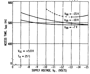
FIG. 2: ACCESS TIME VS SUPPLY VOLTAGE ( V_O )
