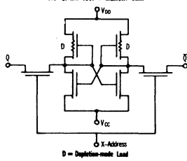
FIG. 8: MX 4007 P MEMORY CELL
