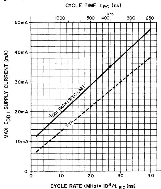
Fig. 10 Maximum I_{DD1} versus cycle rate for device operation at various frequencies. I_{DD1} (max) curve is defined by the equation: I_{DD1} (max) [mA] = 10 + 9.4 x cycle rate [MHz].
