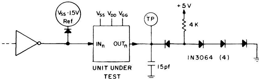
FIGURE #1 t_{ACC} and t_{OD} test circuit
