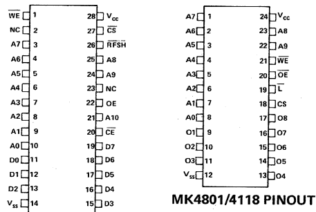
MK 4816 PINOUT
