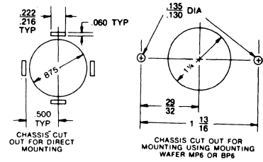
BP6 BAKELITE MOUNTING WAFER
