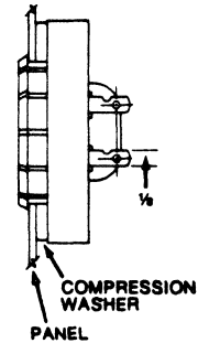
TYPICAL PANEL INSTALLATION
